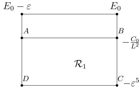
Figure 6.2: Free resonance region below [E_0 - \varepsilon, E_0]
