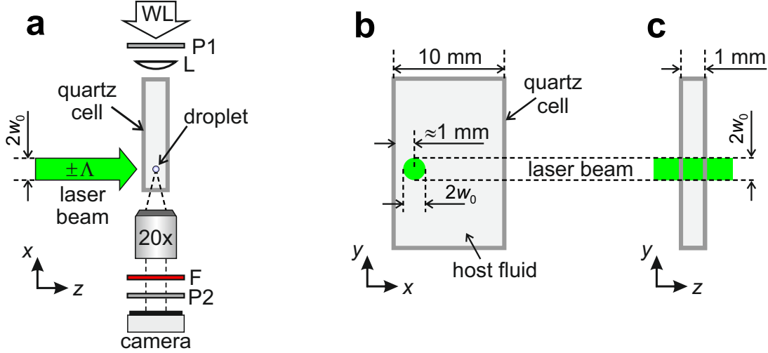
Figure 2.2: (a) Sketch of the experimental setup. Bragg- or anti-Bragg polarized laser beam illuminates a radial cholesteric droplet immersed in a host fluid inside a quartz cell. Elements of the imaging system: white light (WL) source, convex lens (L), microscope objective, CMOS camera, red filter (F) and (optional) crossed linear polarizers (P1, P2). (b, c) Schematic side views of the sample.
