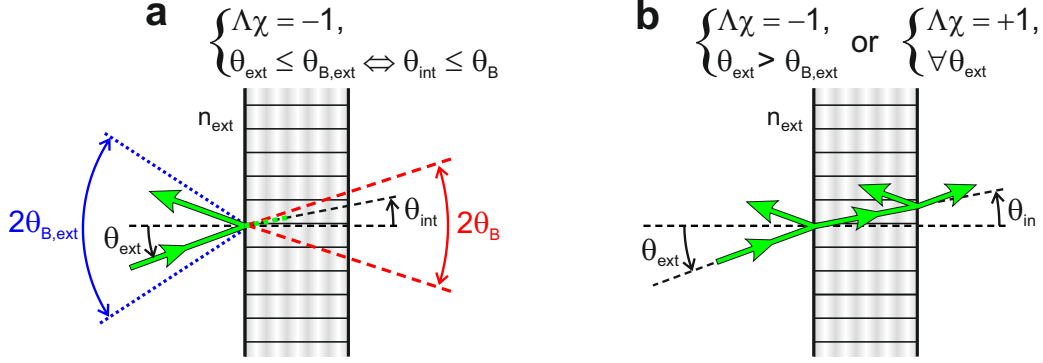
Figure 1.3: (a) Bragg-polarized light is completely reflected if its incident angle falls within the cone having the half-apex angle \theta_{B,\text{ext}} . (b) Circular Bragg reflection is absent either if the incidence angle exceeds \theta_{B,\text{ext}} and the light is Bragg-polarized, or for any incidence angle if the polarization is anti-Bragg.
