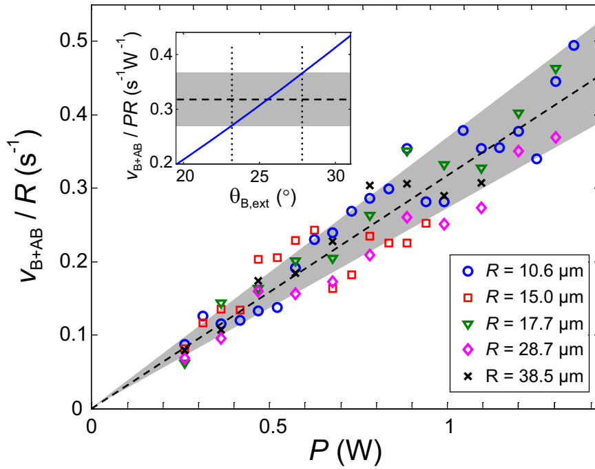
Figure 2.8: The ratio v_{\text{B+AB}}/R is plotted as a function of total beam power P of one beam for various values of the droplet radius R . Dashed curve refers to the best linear fit. Inset: solid line is the theoretical ratio v_{\text{B+AB}}/(PR) vs. \theta_{\text{B,ext}} whereas dashed line and gray area refer to the mean value and the standard deviation range of the experimental dataset v_{\text{B+AB}}/(PR) , respectively. This allows the experimental determination of the precision of \theta_{\text{B}} , see vertical dotted lines.
