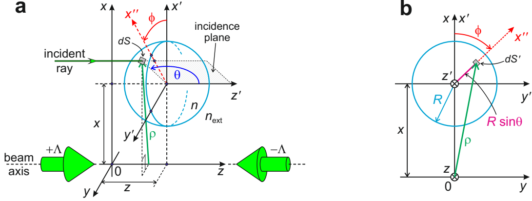
Figure 3.7: (a) Sketch of a spherical droplet (with \chi = -\Lambda ) interacting with the considered two-beam chiral optical field. A single ray impinging on a surface element dS of the droplet is depicted. (b) Distance \rho between the surface element and the beam axis z can be easily derived using the projection on the (x, y) plane ( dS' represents the projection of dS ).
