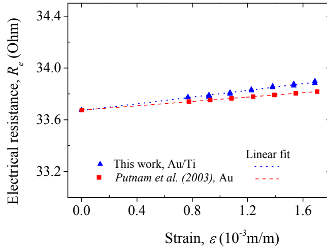
Figure 6.16: Variation of electrical resistance as a function of strain for a Au/Ti heater (blue-dotted line). Results obtained by Putnam et al. (2003) (red-dashed line)
