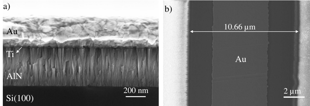
Figure 3.9: (a) SEM micrograph of 20 nm and 230 nm thick Ti and Au layers deposited onto an AlN film. (b) SEM top view of a microfabricated 3\omega strip of \approx 10\text{ }\mu\text{m} width.
