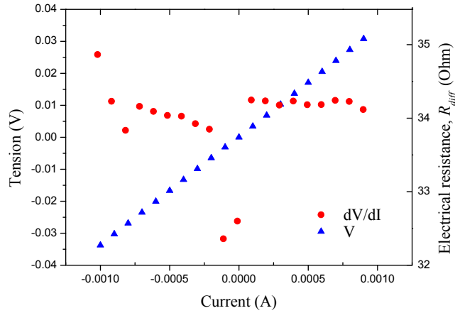
Figure 3.20: Typical raw data of a V(I) measurement for a load of 11 N (obtained for a fixed constant value of strain = 1,69 \times 10^{-3} m/m). A current varying from -1 mA to 1 mA is driven between the outer pads, while the voltage is measured between the two inner probes. The electrical resistance as a function of strain is obtained by determining the slopes of the various V(I) curves measured for different strain values.
