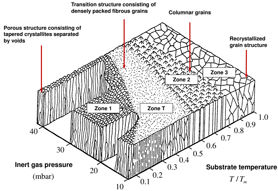
Figure 2.6: Thornton structure zone model. Adapted from Thornton (1977).
