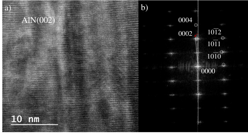
Figure 5.14: a) HRTEM micrograph of columnar grains from a L = 3 \times (\approx 270 \text{ nm}) multilayer (domain III), and b) its corresponding indexed FFT pattern.
