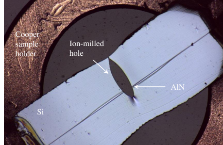
Figure 2.13: Optical micrograph of the bonded together face-to-face AlN/Si slabs with the ion-milled hole
