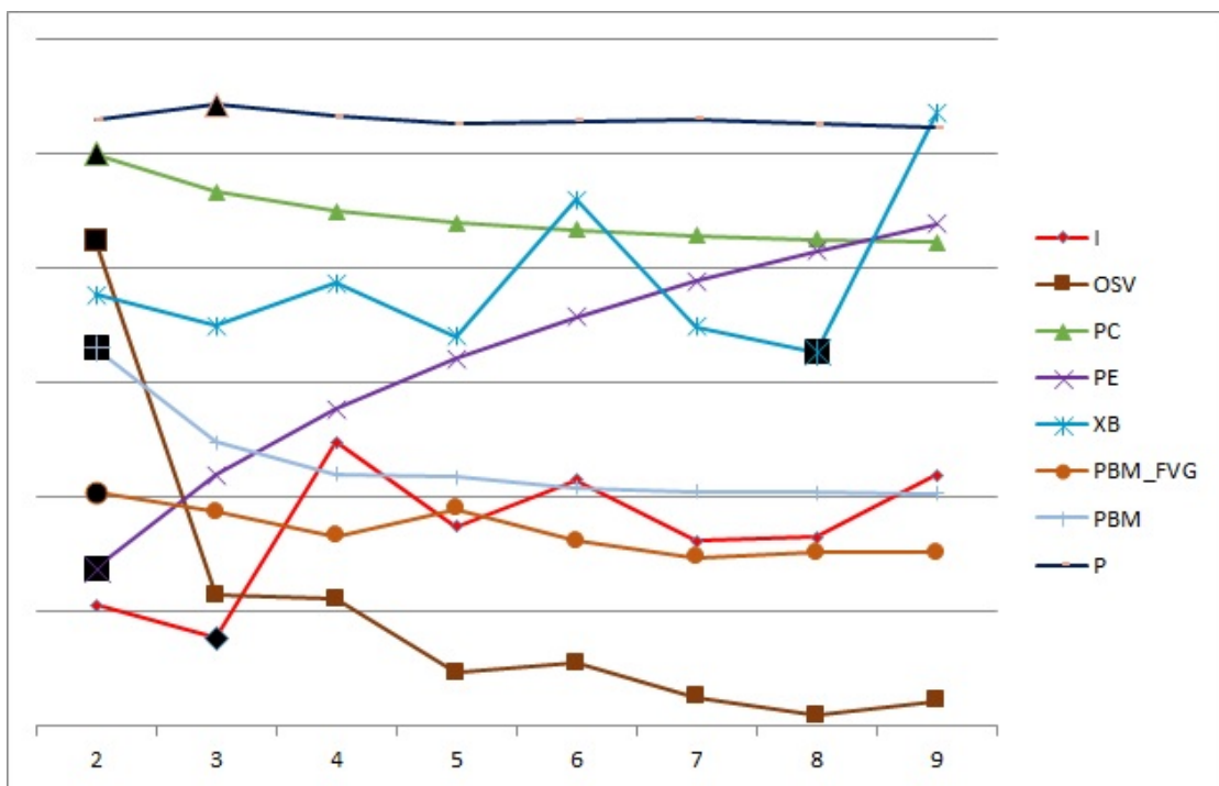
FIGURE 5.37: CVIs for Balance data set with different number of clusters (lines are scaled for display purpose)
