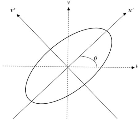
FIGURE 3.1: Anisotropic Gaussian with orientation \theta
