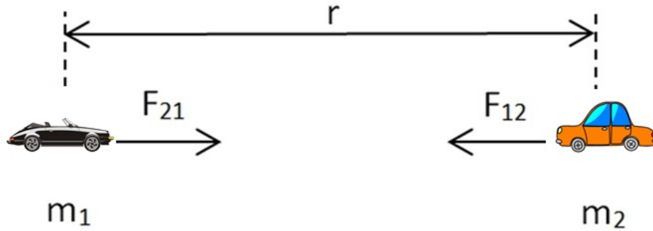
FIGURE 4.1: Illustration of Newton's law of attraction forces between two objects
