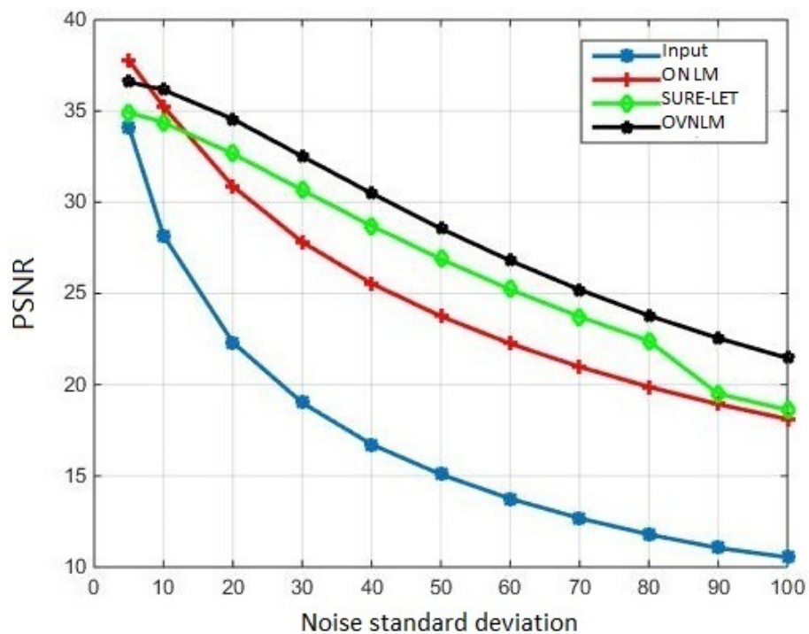
FIGURE 5.16: PSNR curves for subject 1
