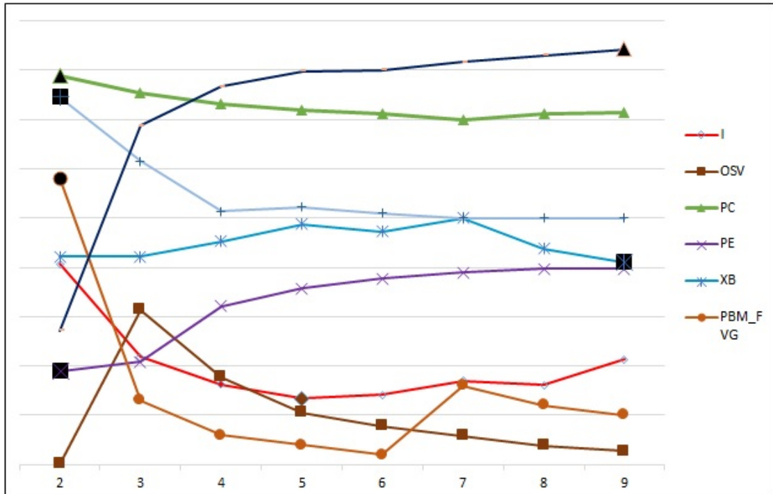
FIGURE 5.40: CVIs for Yale_5 data set with different number of clusters (lines are scaled for display purpose)
