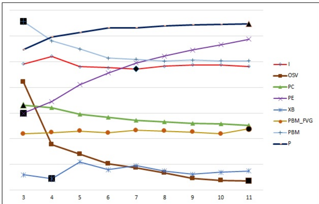
FIGURE 5.41: CVIs for Yale_7 with different number of clusters (lines are scaled for display purpose)
