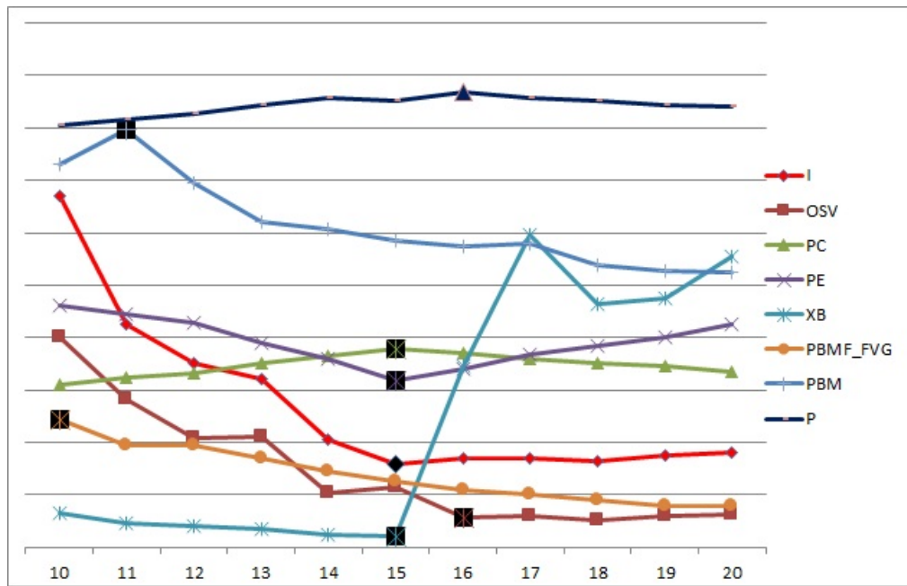
FIGURE 5.28: CVIs for S1 with different number of clusters (lines are scaled for display purpose)
