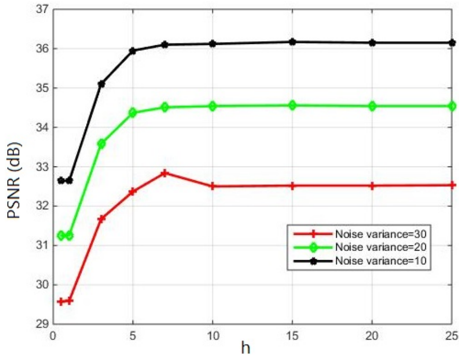
FIGURE 5.19: Variation of PSNR with relative to h
