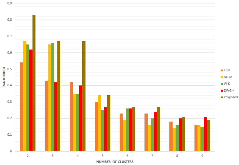
FIGURE 5.20: Thyroid - Rand index
