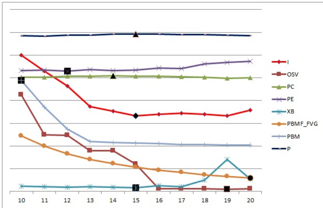
FIGURE 5.34: CVIs for S4 with different number of clusters (lines are scaled for display purpose)
