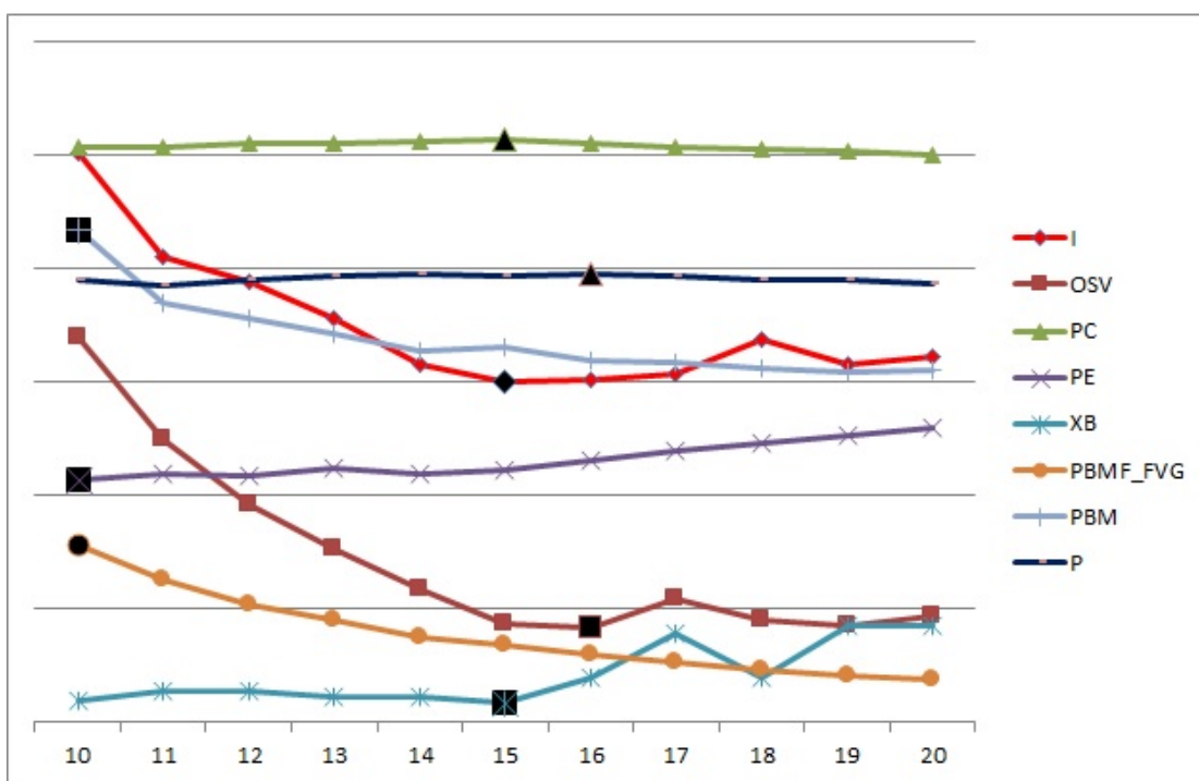
FIGURE 5.32: CVIs for S3 with different number of clusters (lines are scaled for display purpose)
