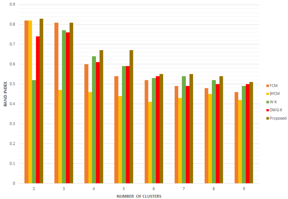
FIGURE 5.21: Imbalanced Glass - Rand index
