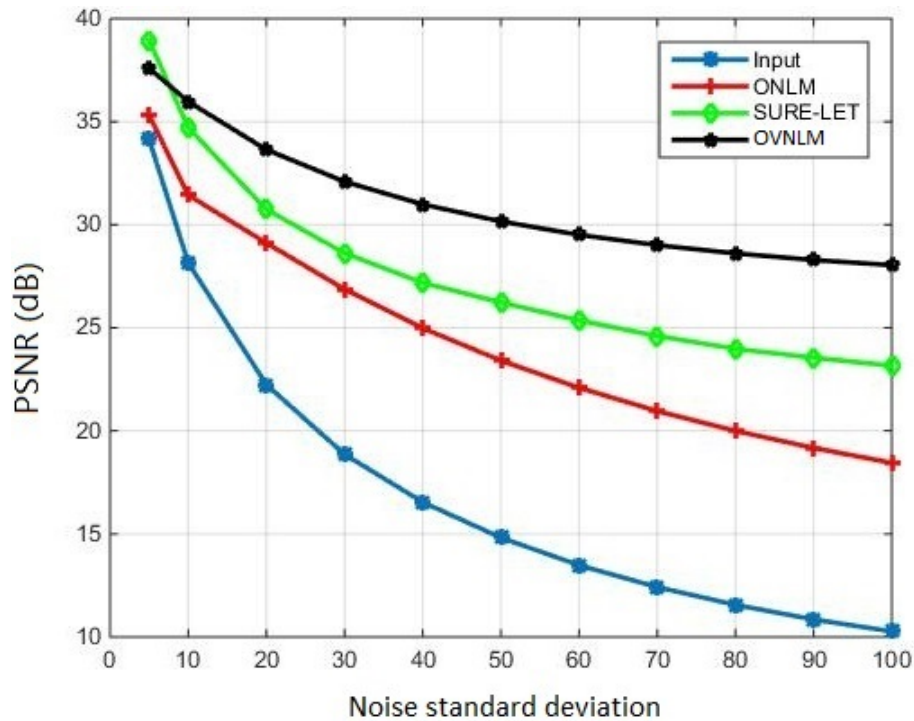
FIGURE 5.18: PSNR curves for subject 2
