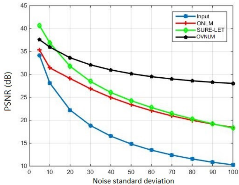
FIGURE 5.8: PSNR variation according to noise standard deviation for Lena image
