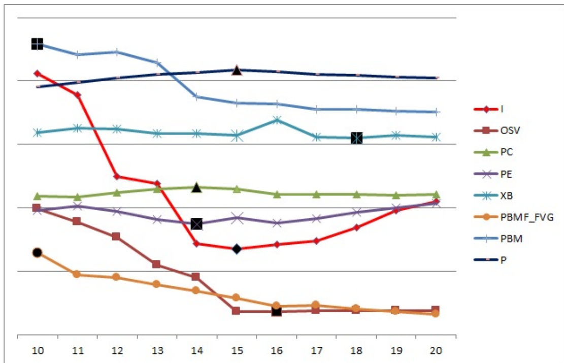
FIGURE 5.30: CVIs for S2 with different number of clusters (lines are scaled for display purpose)
