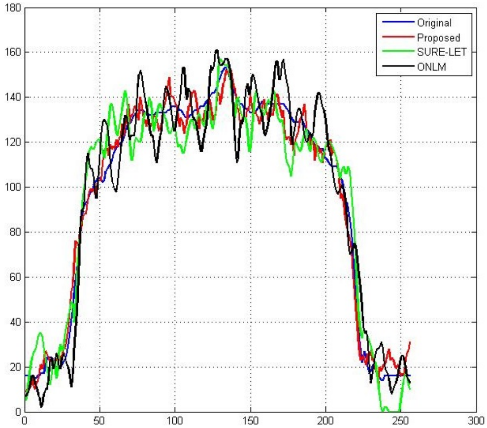
FIGURE 5.12: Pixel variation along a profile for subject 1
