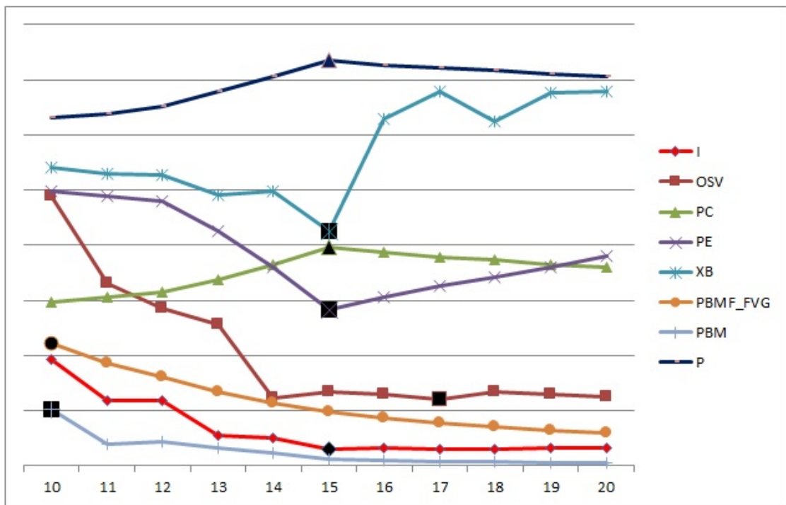
FIGURE 5.36: CVIs for R15 with different number of clusters (lines are scaled for display purpose)
