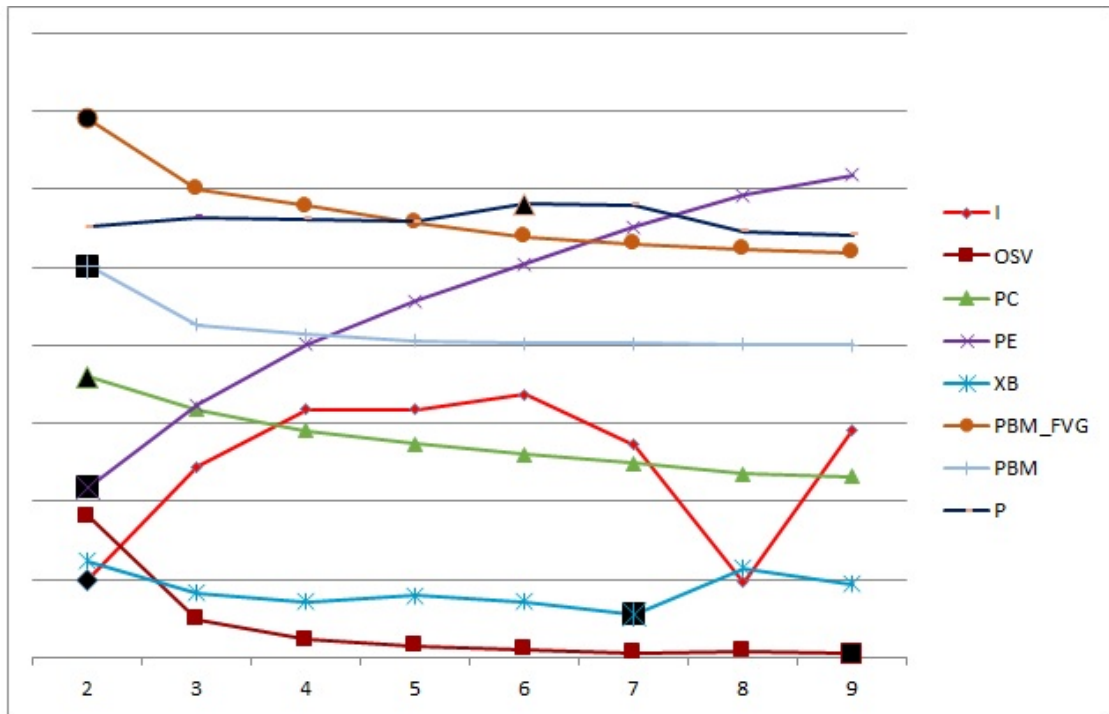
FIGURE 5.38: CVIs for Banana data set with different number of clusters (lines are scaled for display purpose)
