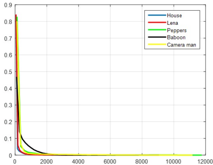
FIGURE 3.2: Normalized histogram of the variance of several famous images
