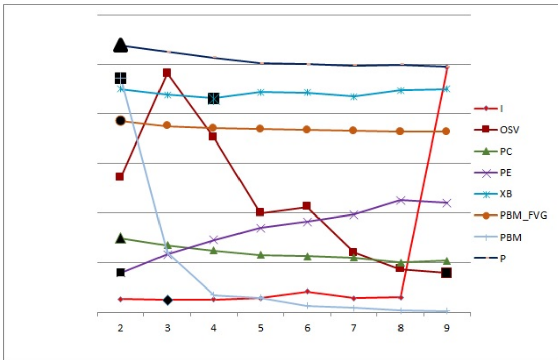
FIGURE 5.39: CVIs for Iris data set with different number of clusters (lines are scaled for display purpose)
