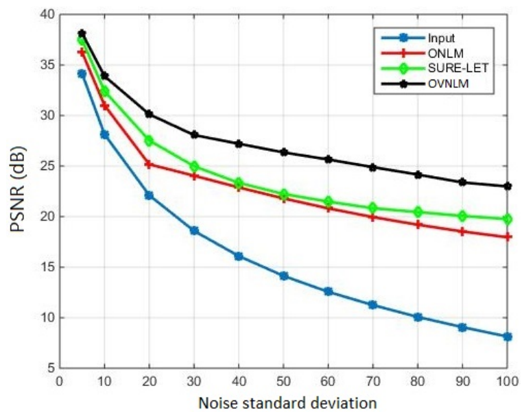
FIGURE 5.10: PSNR variation according to noise standard deviation for Baboon image
