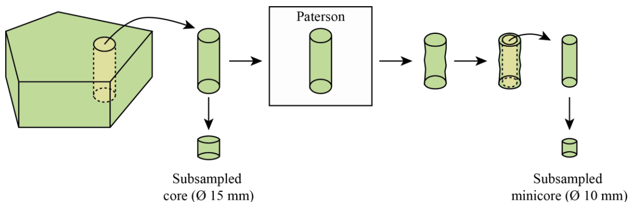
Figure 4: Sampling strategy.
