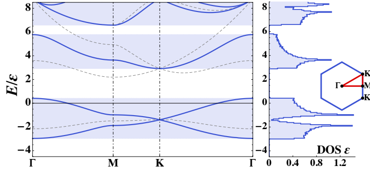
Figure 3.17 : Honeycomb lattice: band structure (left) and DOS (right) for the AAG at \alpha = -0.5 . Left: Behavior of the five lowest energy bands along the irreducible symmetry path in the inset (at right). Dashed (gray) curves show the band structure for the corresponding triangular lattice. Right: DOS [defined in Eq. (3.3.1)] obtained by sampling the band energy in N_s = 3300 points within the symmetry path. The histogram bin size is \delta E = 0.06\epsilon ( \epsilon = \hbar^2/ma^2 ).
