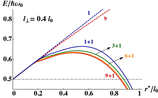
Figure 2.7 : Ground-state energy E_{2B}(r^*) of the Hamiltonian \mathcal{H}_{2B} , for g_{1D} = 0 and l_{\perp}/l_0 = 0.4 , including 1 (blue), 3 (green), 6 (orange), and 9 (red) harmonic oscillator states, without (dashed lines) and with (solid lines) the “bare” bound state |\phi_{-1}\rangle in the projection basis. The quantities \omega_0 , l_0 and l_{\perp} are defined like in Fig. 2.6.
