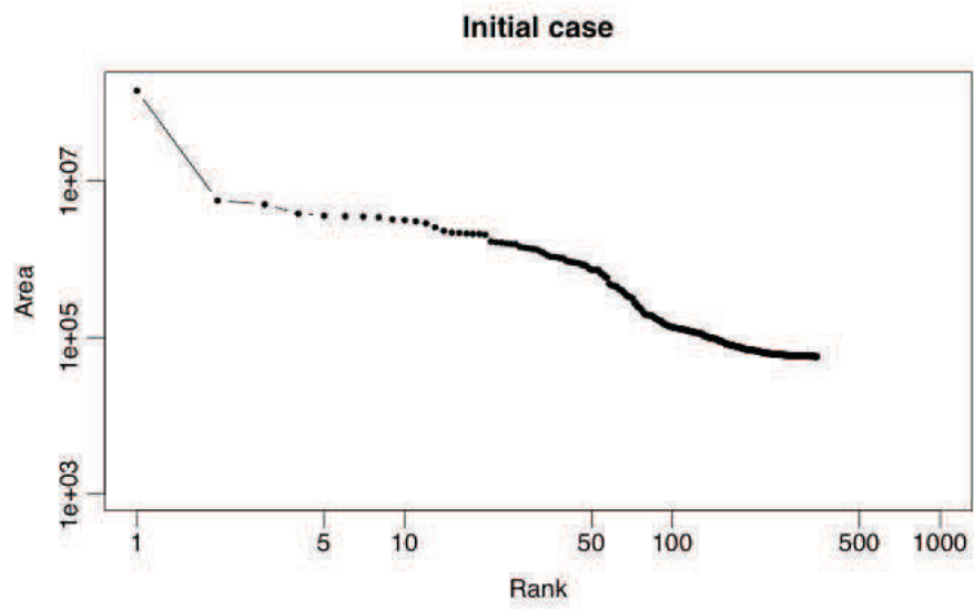
Figure 4.11: The rank-size distribution of the initial case built-clusters (log-log plot).
