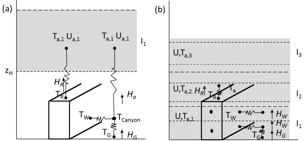
Figure 2.8: Distinction between single and multilayer canopy models (adapted from Kusaka et al. [2001] T_a is the air temperature of the mesoscale grid ( I_1, I_2 , and so on), the obstacle average height is z_H . T_R is the roof surface temperature, T_W the one of the walls, T_G of the ground. Then, H_a is the sensible heat flux from the canyon to the atmosphere, H_W and H_G are that from respectively the walls and the ground to the canyon, and H_R that from the roof to the atmosphere.
