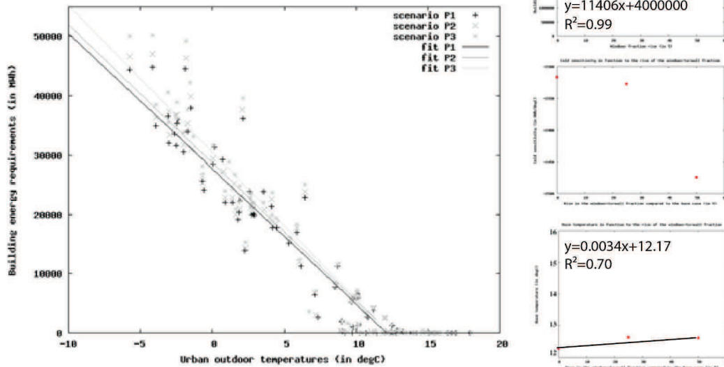
Figure 3.20: At left, sketch of the relationship between the building energy requirements and the urban outdoor temperatures with changes in the window-to-wall fractions. At right, the figures plot the relationships between the building energy requirements EC , the cold sensitivity P , and the base temperature T_0 .
