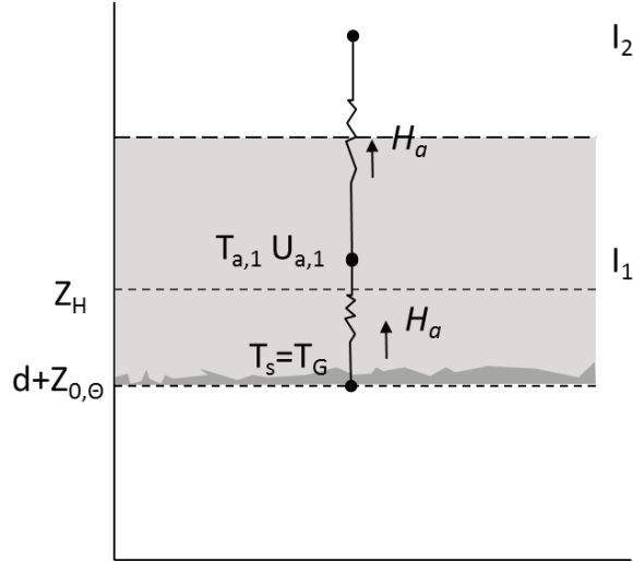
Figure 2.7: Slab model (adapted from Kusaka et al. [2001] ) T_a and U_a are respectively the air temperature and the wind speed of the mesoscale grid ( I_1, I_2 , and so on), the obstacle average height is z_H , d is the displacement height, z_{0,\theta} is the roughness length for heat. T_S is the equivalent surface temperature, and T_G of the ground. Then, H_a is the sensible heat flux from the canyon to the atmosphere.
