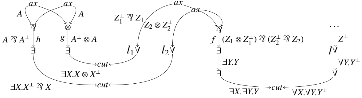
Figure 5.2: \phi_G^{lim}(l, []) = (Z_1 \otimes Z_1^\perp) \wp (Z_2^\perp \wp Z_2) [\phi_G^{lim}(l_1, [])/Z_1; \phi_G^{lim}(l_2, [])/Z_2] \phi_G^{lim}(l, []) = (Z_1 \otimes Z_1^\perp) \wp (Z_2^\perp \wp Z_2) [A^\perp/Z_1; A^\perp/Z_2] \phi_G^{lim}(l, []) = (A^\perp \otimes A) \wp (A \wp A^\perp)
