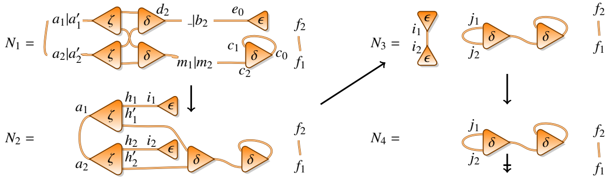
Figure 6.6: Example of reduction with the library L_{comb} .
