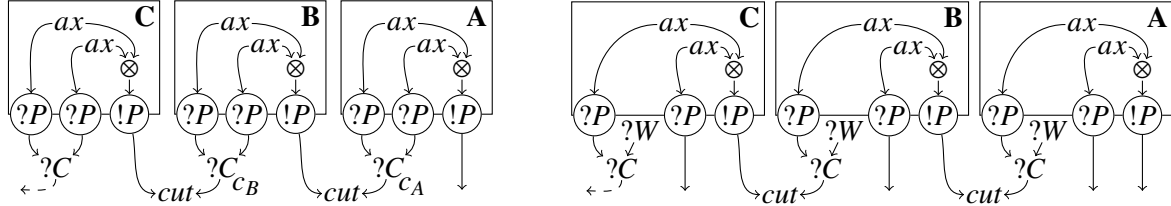
(a) This proof-net (if extended to n boxes) reduces in O(2^n) reduction steps
