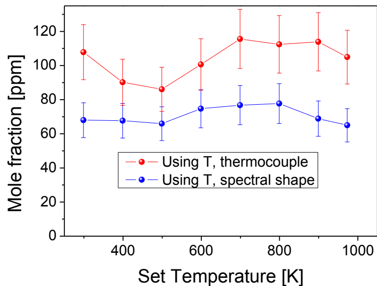
Figure 6.15: NO mole fraction as a function of the gas temperature. The NO mole fraction remains constant with increasing gas temperature. Conditions: U = 3 kV, f = 30 kHz, d = 2 mm, v = 1.7 m/s, z = 25 cm.
