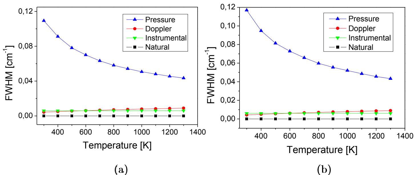
Figure 3.23: Comparisons of broadening widths as a function of the gas temperature. (a) line at 1900.076 \text{ cm}^{-1} (b) line at 1900.517 \text{ cm}^{-1} . The broadening of both lines is dominated by collisional broadening.
