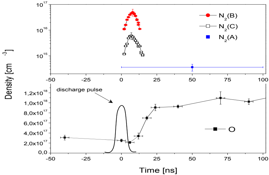
Figure 2.12: Temporal evolution of N_2(A, B, C) and O densities during first 100 ns. Figure taken from [ Stancu et al. , 2009].
