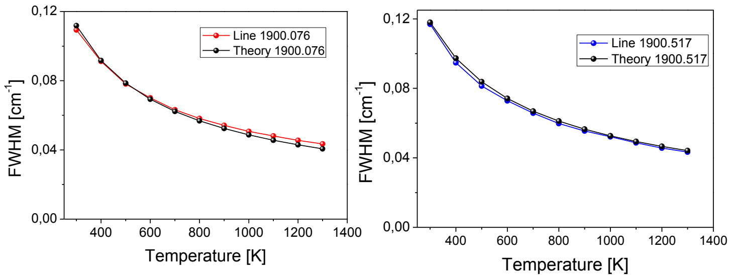
Figure 3.21: Comparison between individual and global fits.
