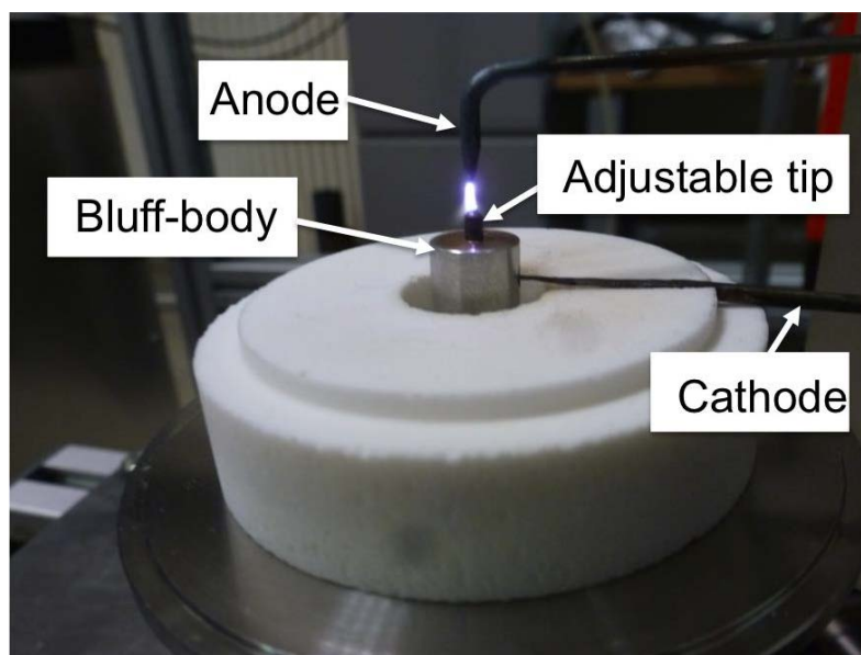
Figure 4.1: Discharge assembly with the bluff-body and the two electrodes. Bluff body tip is 5-mm long with a diameter of 2 mm. This configuration is mainly dedicated to combustion applications.
