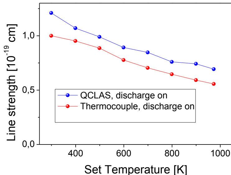
Figure 6.13: Line 1 intensity as a function of the set gas temperature. Two cases: using the temperatures measured with the thermocouple and with the collisional spectral width. Conditions: U = 3 \text{ kV} , f = 30 \text{ kHz} , d = 2 \text{ mm} , v = 1.7 \text{ m/s} , z = 25 \text{ cm} .
