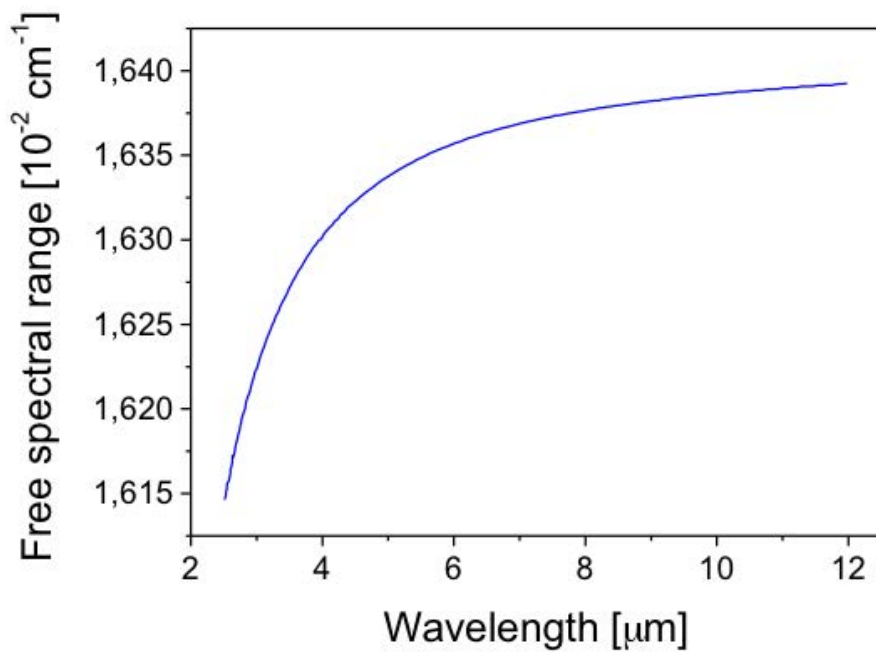
Figure 4.22: Germanium etalon free spectral range as a function of the wavelength. At 5.2 μm, FSR ~ 0.0163 cm -1 .
