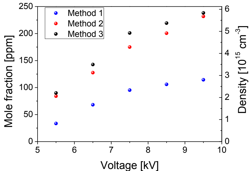
Figure 6.4: Comparison of the three methods for NO density determination. Method 1 systematically underestimates the NO density while methods 2 and 3 give close results.
