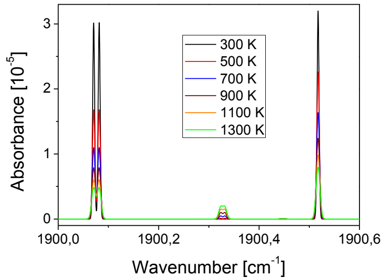
Figure 3.14: Absorbance spectra of both transitions for temperatures from 300 to 1300 K. P = 1 mbar, L = 1 mm, N = 2.45 \times 10^{13} cm -3 .
