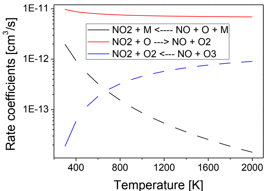
Figure 6.27: Rate constants for reactions R15 to R17. The formation rates are dominated by the reactions of NO 2 molecules with O atoms whereas reverse rates at 2000 K are dominated by the reactions of NO with ozone.
