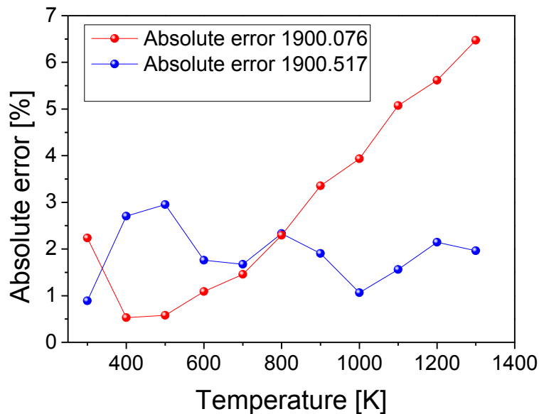
Figure 3.22: Error induced by neglecting line overlap.
