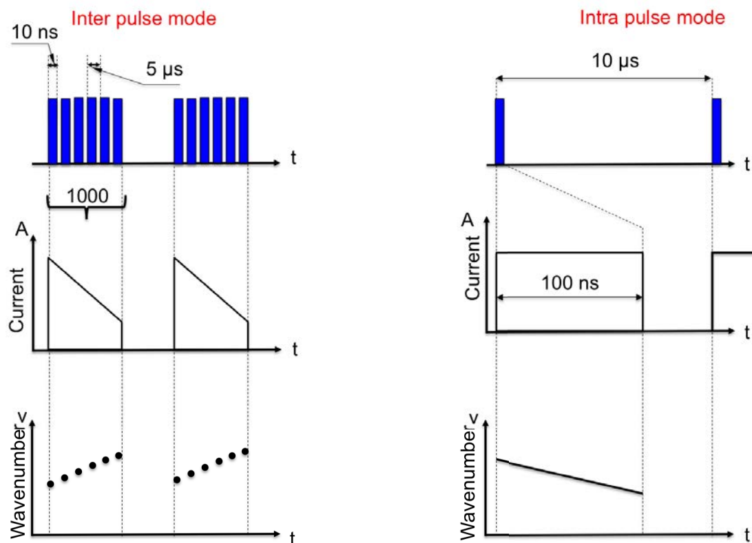
Figure 4.8: Principles of inter-pulse and intra-pulse laser tuning modes. A complete spectrum is recorded after about 5 ms using the inter-pulse mode while it takes 100 ns in intra-pulse mode.
