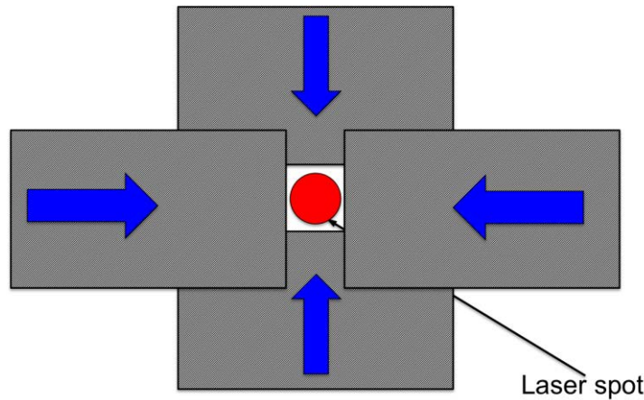
Figure 4.12: Measurement of IR-laser spot size at discharge center. Transmitted signal measured by the detector is the same with a 300\ \mu\text{m} \times 250\ \mu\text{m} window defined by the four knives as without it.
