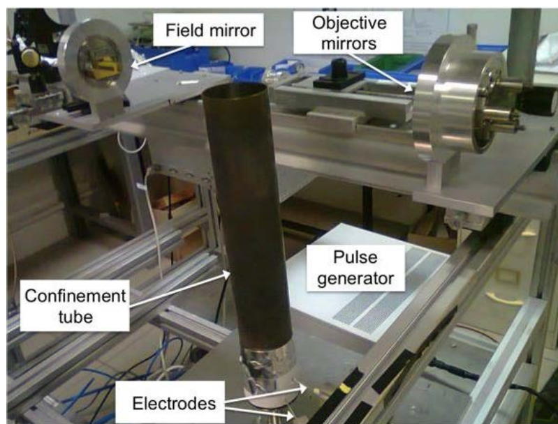
Figure 4.17: Side view of the multiple pass absorption cell with the discharge generation system and the confinement tube. NRP discharges are generated near the bottom of the confinement tube.
