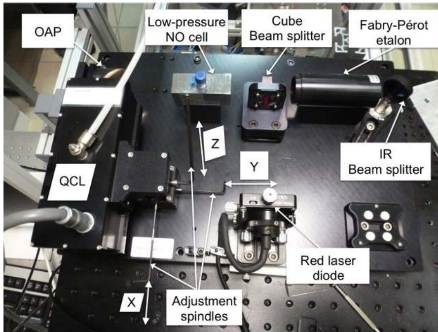
Figure D.2: Signal maximization. Positioning of the QCL at the focal point of the OAP mirror using precise adjustment spindles.
