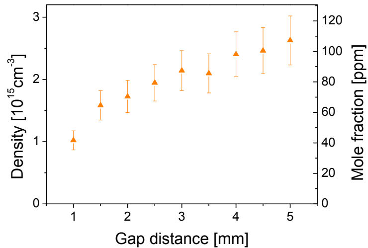
Figure 6.7: NO density/mole fraction as a function of the gap distance. The NO mole fraction increases with gap distance. Conditions: U = 5.3 \text{ kV} , f = 30 \text{ kHz} , v = 8.63 \text{ m/s} , z = 50 \text{ cm} , T = 300 \text{ K} .
