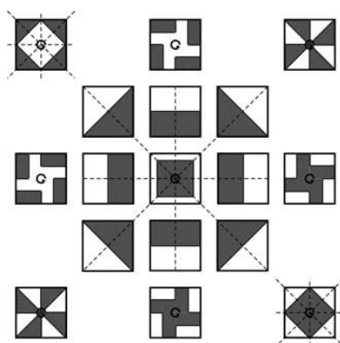
Fig. 2. The square profile possesses 4 mirror planes and a 4-fold rotational axis ( 4 \cdot M, R_4 ). For a constant passive/active area ratio of 50 : 50, those symmetry elements can either be maintained by the material distribution (centre, upper left and downer right corner), decreased to a single mirror plane (inner contour) or to one 4-fold rotational axis (outer contour). The inner contour is used as RUC for the outer contour showing that the 4-fold patterned cross-section can still possess 4 mirror planes if the RUC possess a mirror plane passing through the centre of rotation.
