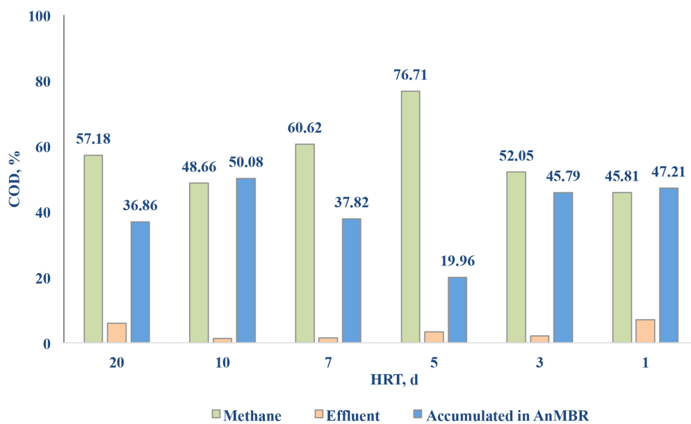
Figure 8.7: COD balance
