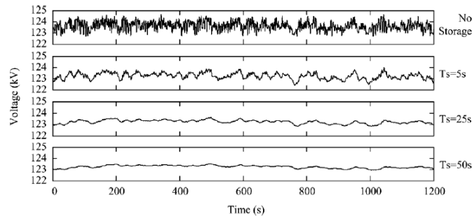
Fig. 14. Voltage at PCC, deploying ESS with different ratings at the PCC in the high energy sea state ( B_L = 10e5 Kg/s and M_L = 5e5 kg, Z_{grid} = j 50.52 \Omega ).
