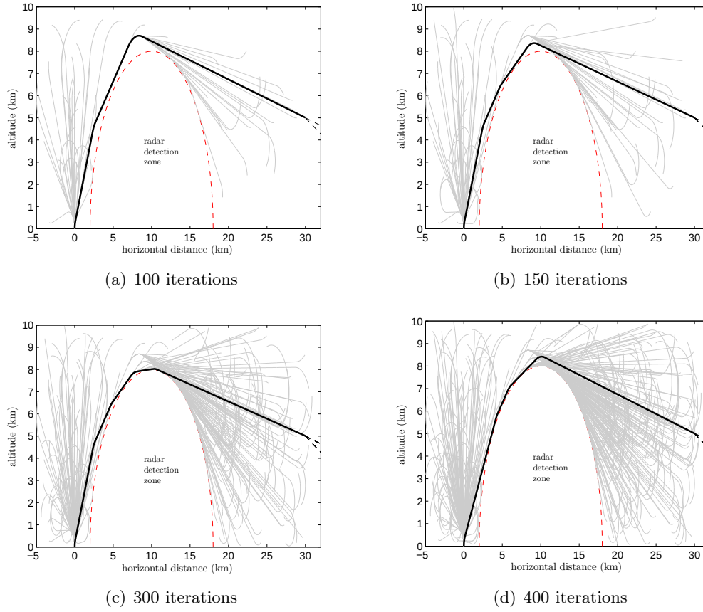
Figure 7.6: Exploration tree expansion and results for scenario 1
