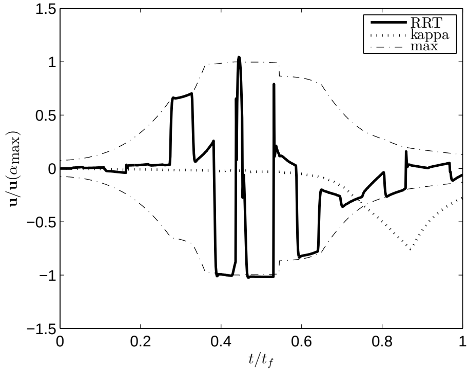
(b) \text{RRT}_{\text{kappa}} : Lateral accelerations along the solution trajectories
