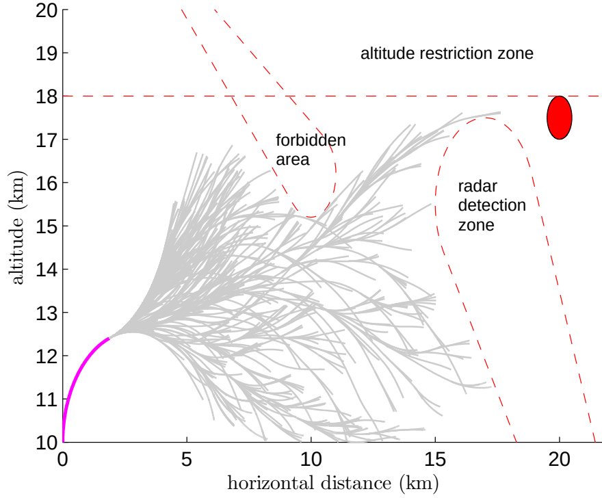
Figure 6.13: Scenario 3: Simulation result using \text{RRT}_{\text{kappa}}
