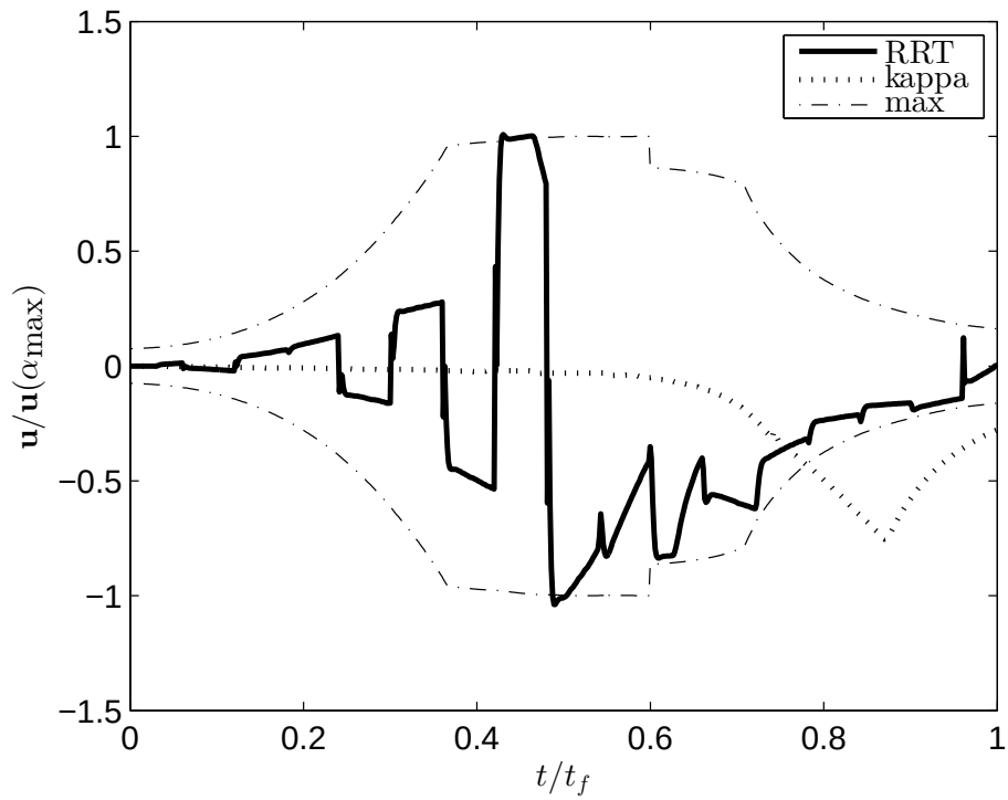
(b) \text{RRT}_{\text{PN}} : Lateral accelerations along the solution trajectories
