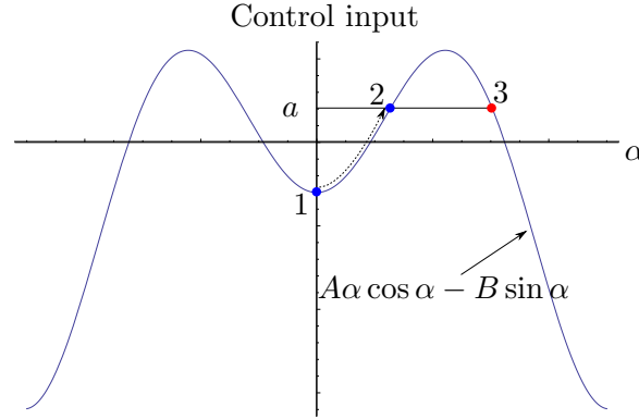
Figure 2.6: Relation between the control input a and the angle of attack \alpha
