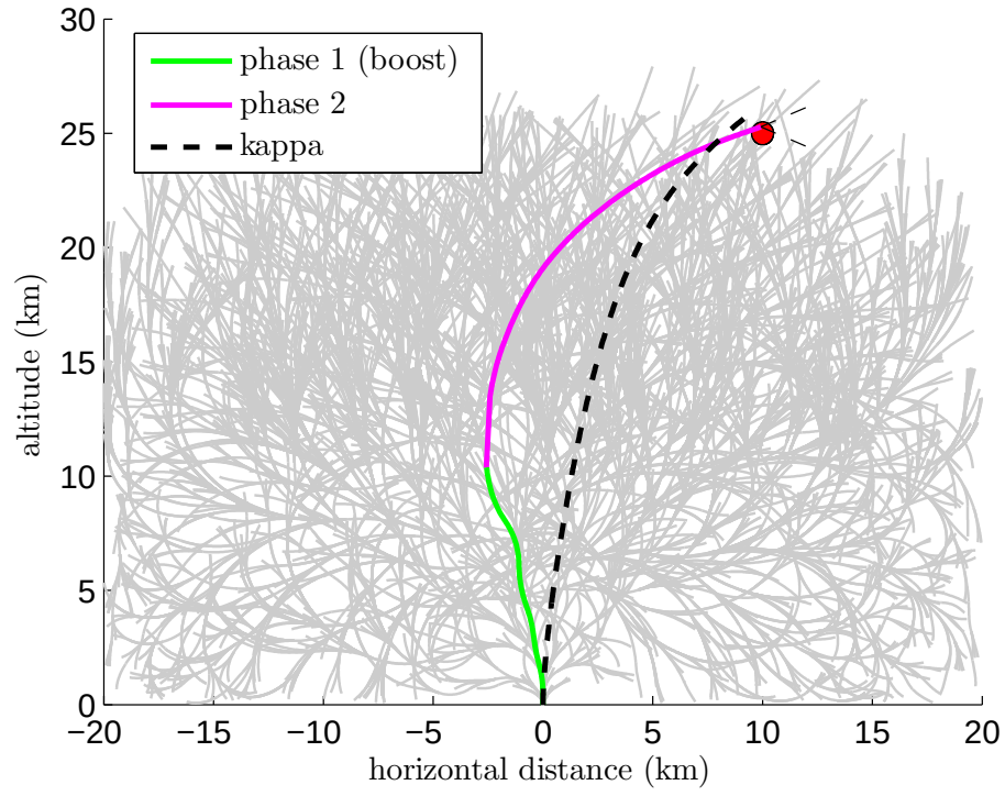
(a) \text{RRT}_{\text{PN}} : Trajectories
