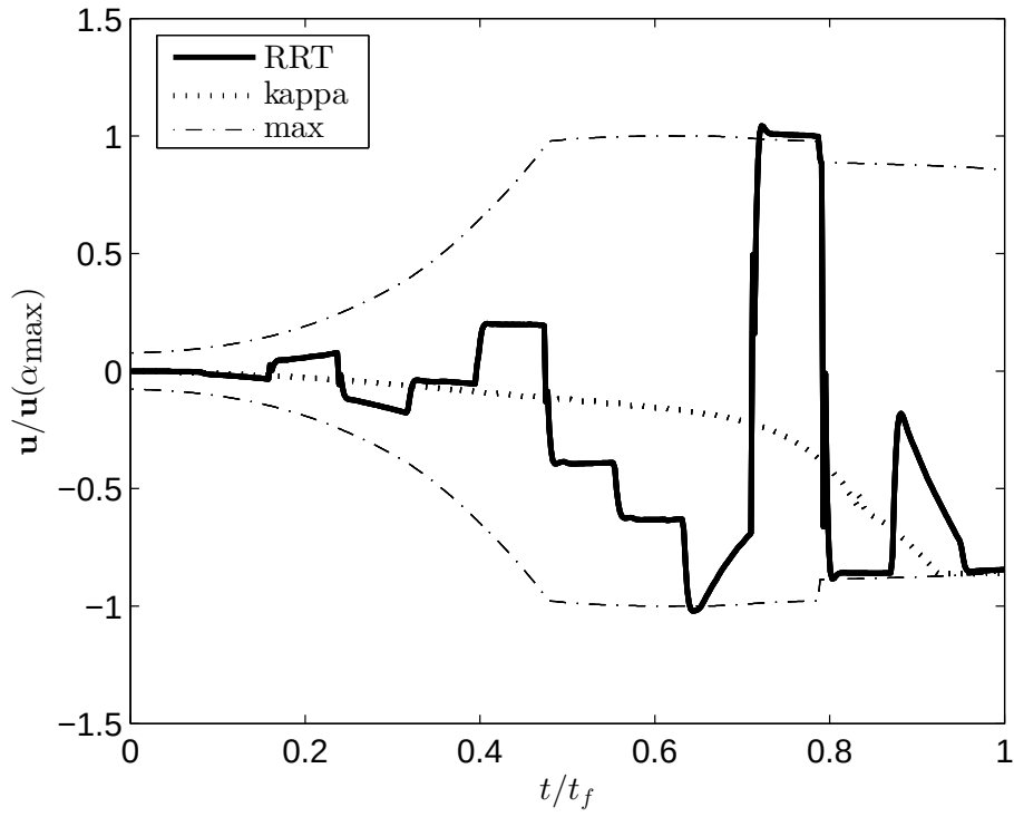
(b) \text{RRT}_{\text{kappa}} : Lateral accelerations along the solution trajectories
