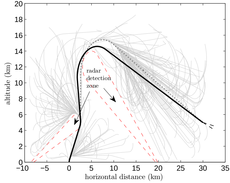
(a) 400 iterations
