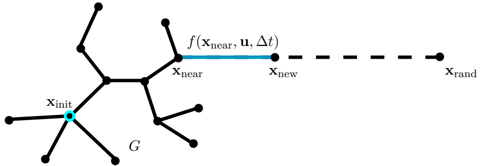
Figure 4.6: The rrt_extend operation
