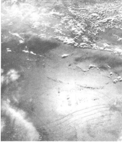
Figure 2: Sea-surface expressions of solitons in the Andaman Sea, observed and photographed by V.Brand, 23 July 1975, from the Apollo spacecraft, after undocking from the USSR's Soyuz.
