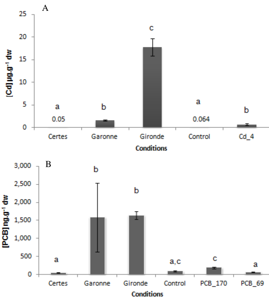
Fig.1 Mean hepatic Cd ( \mu\text{g}\cdot\text{g}^{-1} , dw) (A) and muscle PCBs ( \text{ng}\cdot\text{g}^{-1} , dw) (B) concentrations in controls, in fish experimentally exposed to dissolved Cd at 4\ \mu\text{g}\cdot\text{L}^{-1} (Cd_4) or to PCBs-contaminated food at two concentrations (PCB_170, PCB_69 for 50\ \text{ng}\cdot\text{g}^{-1} and 300\ \text{ng}\cdot\text{g}^{-1} , respectively) and in wild animals (Certes, Garonne, Gironde). Results are expressed as mean \pm SE ( n=5 ). Means designated with different letters are significantly different (LSD test, P < 0.05 ).
