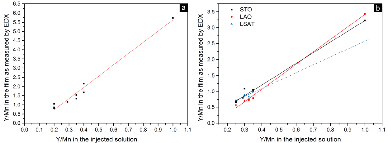
Figure III.9. Atomic ratios Y/Mn in the film as measured by EDX vs. Y/Mn in the injected solution for the depositions at 800\text{ }^\circ\text{C} on a) Si substrate and b) STO, LAO or LSAT substrates.
