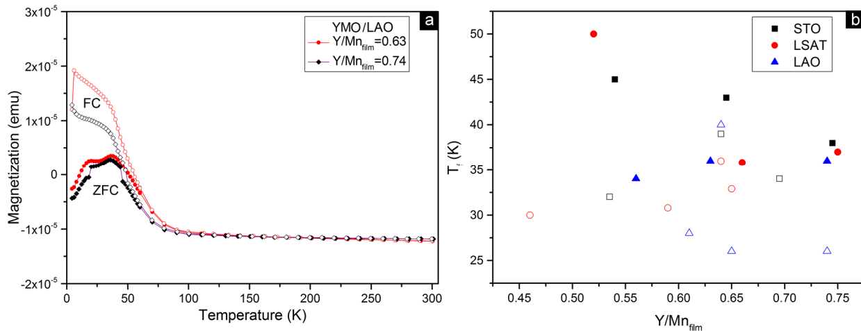
Figure VI.28. a); Temperature dependence of the magnetization ( M(T) ) for the YMO/LAO films deposited with no. inj.=4000 and at two different Y/Mn_{solution} (0.35 and 0.30) corresponding to Y/Mn_{film}=0.74 (in black) and Y/Mn_{film}=0.63 (in red); b) The freezing temperature ( T_f ) as derived from the ZFC curves for the YMO films on STO, LAO and LSAT substrates (the open symbols represent the films deposited at constant Y/Mn_{solution} ratio and variable number of injections and the close symbols those with constant number of injections and variable Y/Mn_{solution} ratio).
