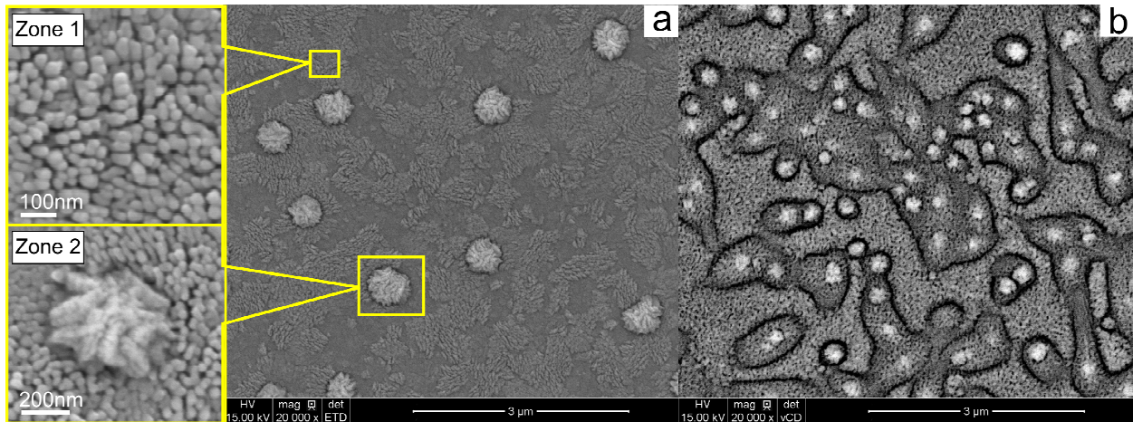
Figure IV.10. Top view SEM images of h-YMO films: a) YMO-800-1-s1 sample. Zone 1 shows a columnar morphology, zone 2 displays a dendritic-like feature; b) YMO-850-1.2 sample.
