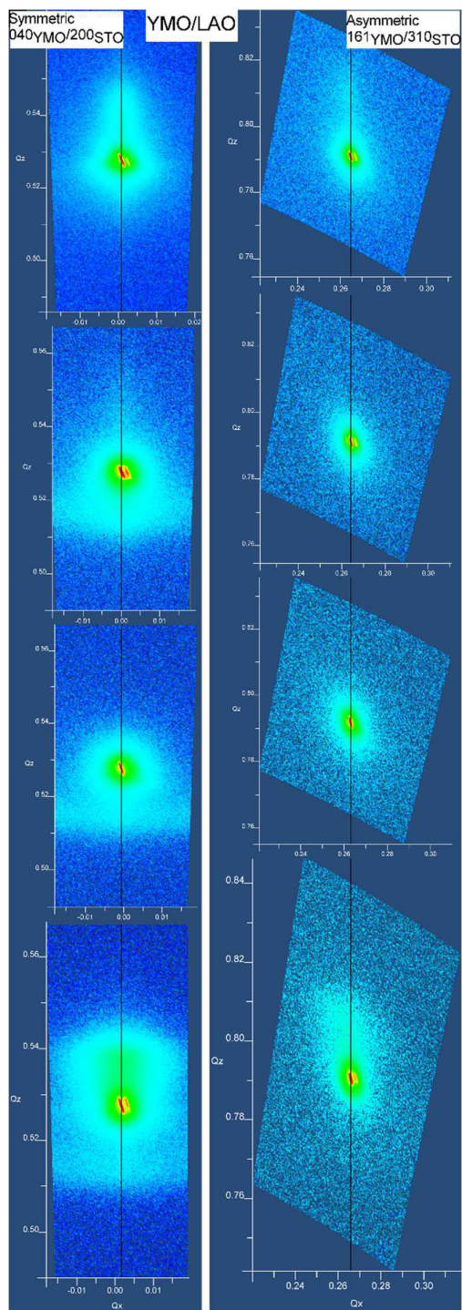
Figure E.1. RSM for YMO films on LAO substrate with different thicknesses (from top to bottom: 500, 1000, 2000 and 4000 inj.) at Y/Mn ct. ( Y/Mn_{solution}=0.325 ) around the symmetric reflection 040_{YMO} and asymmetric reflection 161_{YMO} .
