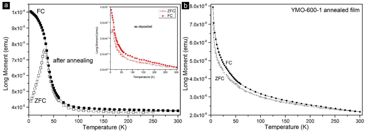
Figure V.14. Temperature dependence of the magnetization in both the ZFC (open symbol), and FC (filled symbol) modes for YMO-600-1 sample annealed a) ex-situ at 900 °C; b) in-situ at 1100 °C. Inset of a): temperature dependence of the magnetization for the as-deposited film.
