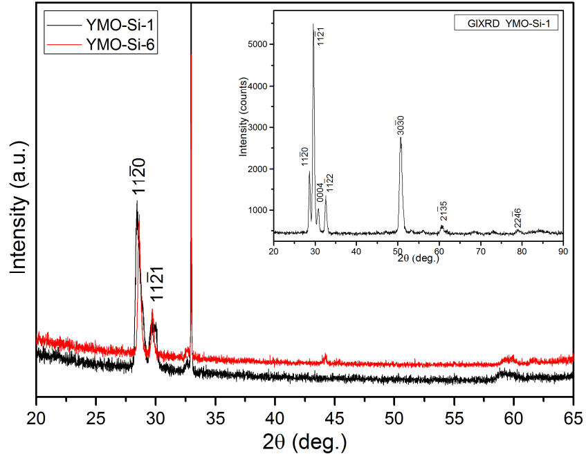
Figure IV.17. \theta -2 \theta XRD patterns of h -YMO films deposited by PLD at different O 2 pressures. The Miller indices correspond to the reflections of the hexagonal YMnO 3 phase (JCPDS card No. 11-9577). Inset: The GIXRD pattern of the YMO-Si-1 sample.
