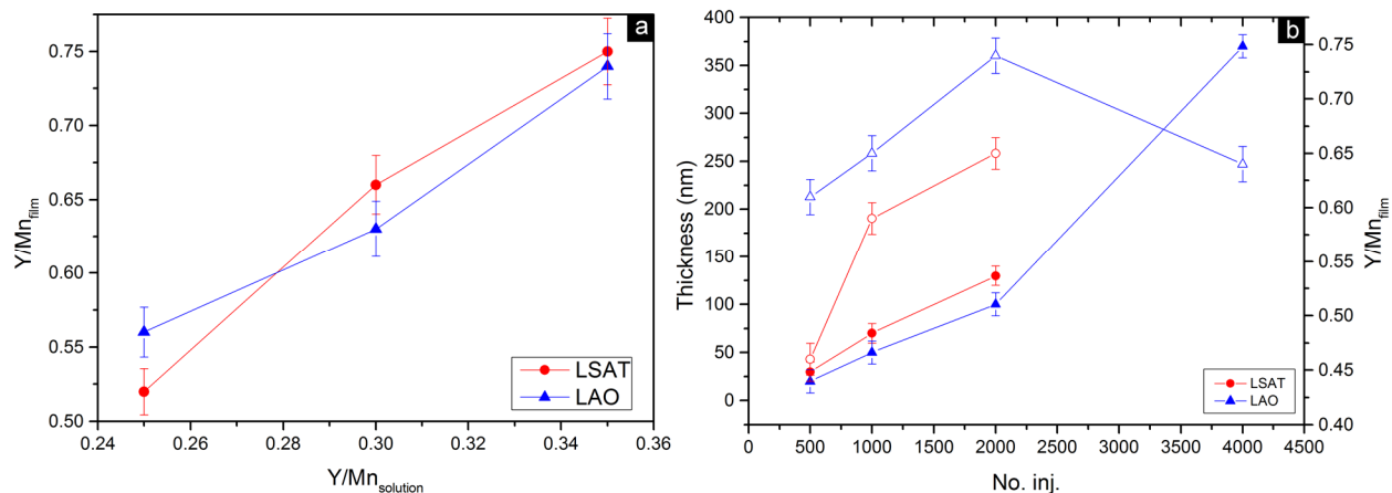
Figure VI.21. EPMA results for YMO films on LAO and LSAT substrates. a) Variation of the Y/Mn_{film} as a function of the increasing Y/Mn_{solution} ; and b) Evolution of the film thickness (close symbols) and the Y/Mn_{film} (open symbols) as a function of the number of injections in the precursor solution.
