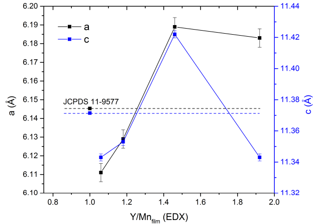
Figure IV.9. The lattice parameters a and c of the h -YMO phase vs. the Y/Mn ratio (measured by EDX) in the film (dotted lines represent the values from the JCPDS card No. 11-9577).
