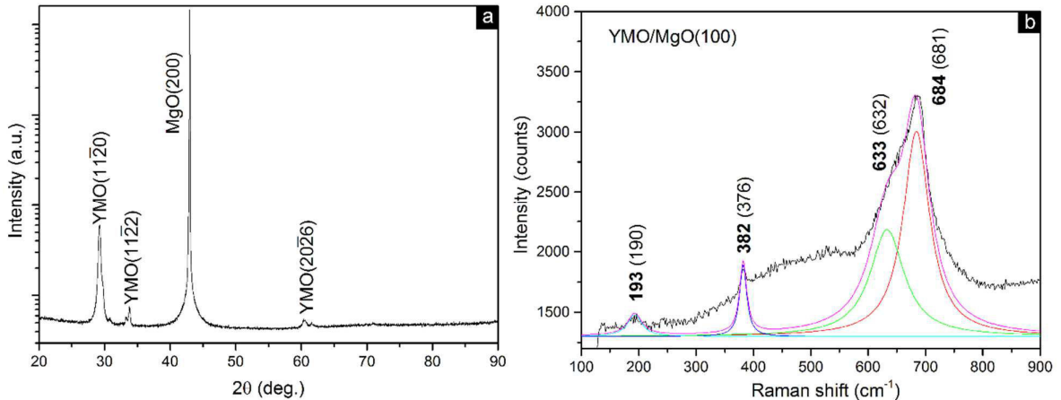
Figure A1. YMO film on MgO(100) substrate deposited with the vertical PI-MOCVD setup: a) XRD pattern; b) Raman spectrum in which the experimental position of each mode are marked by bold numbers (in parentheses are given the values from Iliev et al.[1]). The MgO does not have any active Raman mode.
