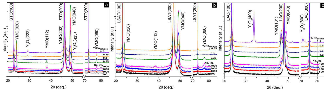
Figure VI.23. \theta - 2\theta XRD patterns of o -YMO films grown on top of STO (a), LSAT (b) and LAO (c) substrates. The patterns represented in the bottom part correspond to thickness varying samples ( \text{Y}/\text{Mn}=0.325 and No. inj. from 500 to 4000) and those in the top part to the varying composition ( 0.25 < \text{Y}/\text{Mn}_{\text{solution}} < 1 , No. inj. 4000) – see Table VI.7 for thicknesses and \text{Y}/\text{Mn}_{\text{film}} .
