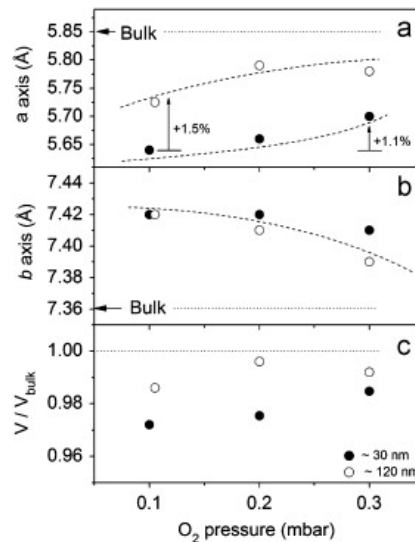
Figure VI.9. Lattice parameters of films grown at different pressures, \sim 30 nm thick (closed symbols) and \sim 120 nm thick (open symbols): (a) a -axis, (b) b -axis and (c) unit cell volume. Horizontal dashed lines correspond to the bulk values (from [4]).
