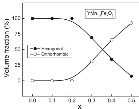
Figure I.7. Volume fraction of hexagonal and orthorhombic phases of YMn 1-x Fe x O 3 (from [22]).
