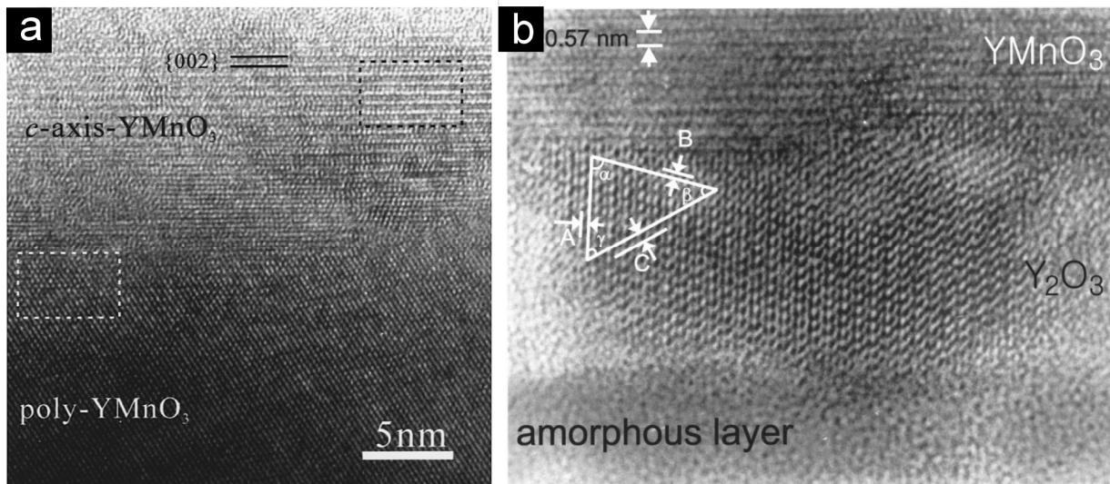
Figure I.18. HRTEM images showing: a) interfacial microstructure between the c -axis-oriented h-YMO layer and the polycrystalline h-YMO layer (from [122]); b) h-YMO film on top of the \text{Y}_2\text{O}_3 and amorphous layers (from [118]).
