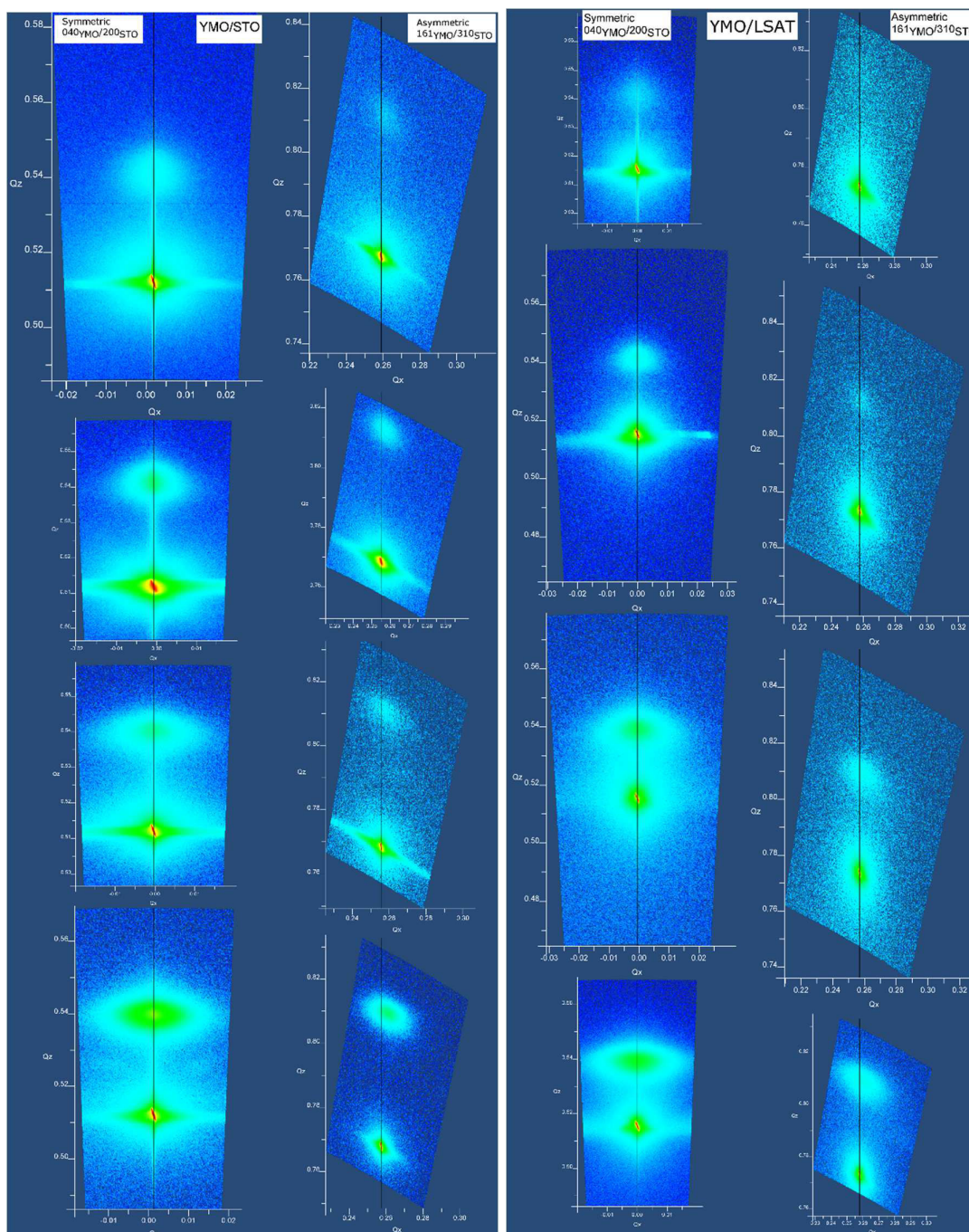
Figure E.1. RSM for YMO films on STO (left) and LSAT (right) substrates with different thickness (from top to bottom: 500, 1000, 2000 and 4000 inj.) at Y/Mn ct. ( Y/Mn_{solution}=0.325 ) around the symmetric reflection 040_{YMO} and asymmetric reflection 161_{YMO} .
