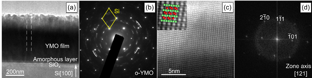
Figure IV.29. TEM results of the o -YMO film deposited by MOCVD: a) low magnification cross-section image showing three different layers on top of the Si substrate; b) SAED pattern of a region of (a) containing several columnar grains and the Si substrate; c) HRTEM image of the o -YMO film in a particular [121] -zone axis orientation. In the inset an enlargement overlapped with the structure simulation; d) FFT of the HRTEM image from (c) showing that the orientation corresponds to [121] -zone axis.
