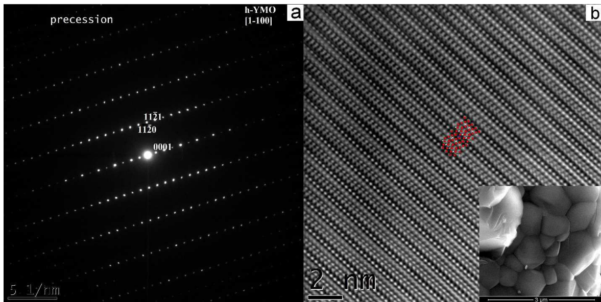
Figure C.1. ED pattern (a) in [1-100] -zone axis and corresponding TEM image (b) overlapped with the simulated structure (CarIne) of a crystalline particle (see SEM image in inset of b) from the YMnO 3 sample.
