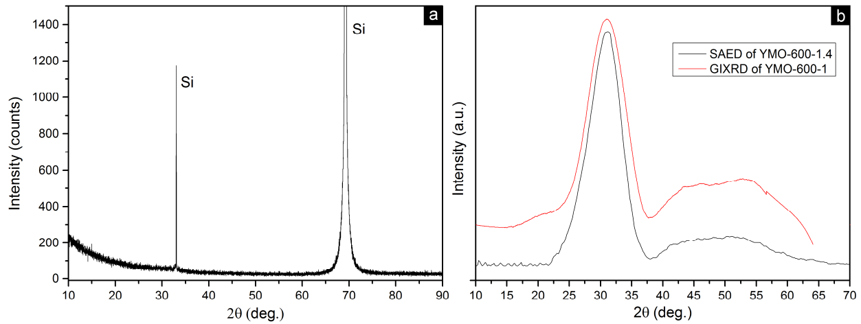
Figure IV.1. a) \theta - 2\theta XRD pattern of YMO-600-1-v sample; b) GIXRD pattern of YMO-600-1 sample overlapped with the transformed ED pattern into 2\theta range of the YMO-600-1.4 sample.
