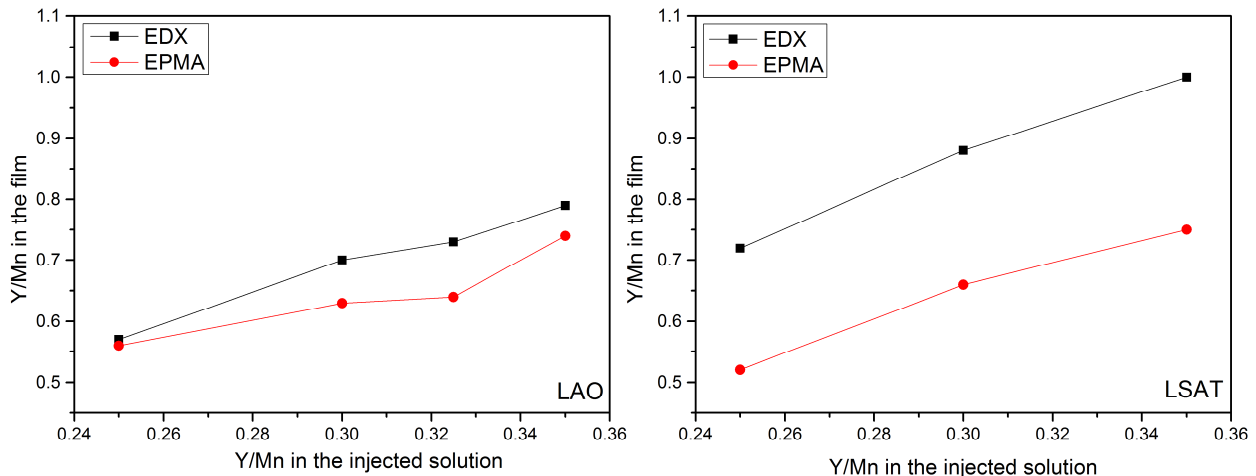
Figure III.10. Atomic ratios Y/Mn in the film as measured by EDX and EPMA vs. Y/Mn in the injected solution for samples deposited at 800\text{ }^\circ\text{C} on a) LAO and b) LSAT substrates.
