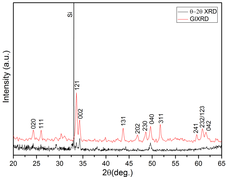
Figure IV.31. \theta - 2\theta XRD (black line) and GIXRD (red line) patterns of the o-YMO film grown by PLD ( P_{O_2}=0.3 bar, T=800 °C).
