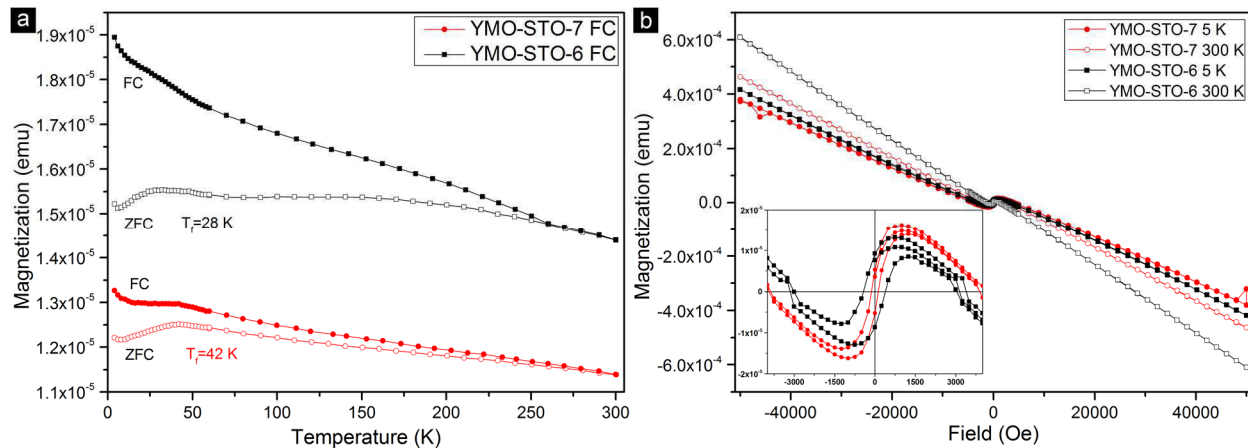
Figure VI.19. a) Temperature dependence of the magnetization ( M(T) ) for the YMO/STO films deposited by PLD at two different P_{\text{O}_2} : 1.4 \cdot 10^{-4} bar (YMO-STO-6 film in black) and 3 \cdot 10^{-1} bar (YMO-STO-7 in red); b) Field dependence of the magnetization ( M(H) ) at 5 and 300 K (in the inset: enlargement of the M(H) curve in the -5000 to 5000 Oe range).
