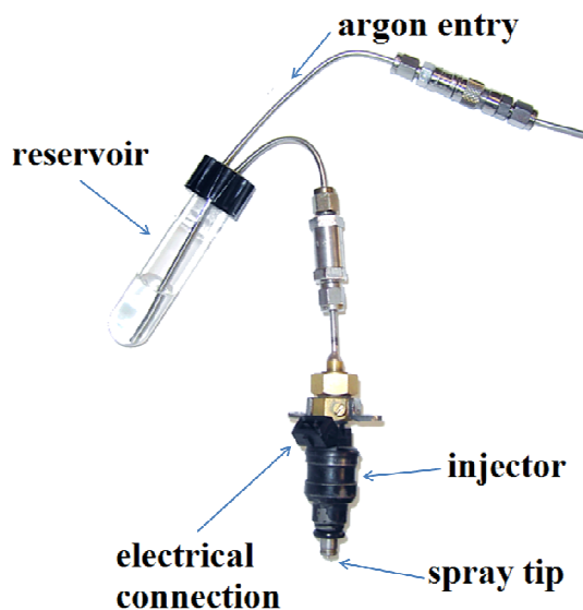
Figure II.3. Precursor injection system (from [6]).
