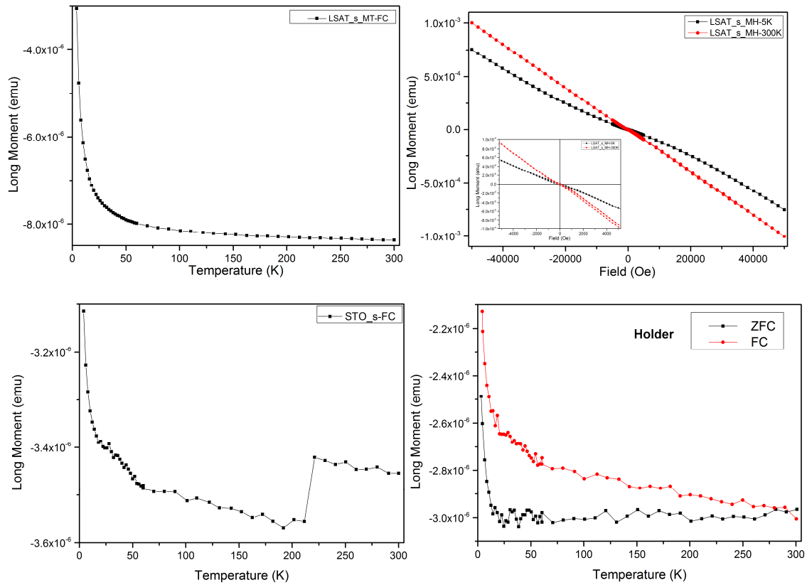
Figure D.2. Temperature dependence of the magnetization ( M(T) ) of bare LSAT and STO substrates and of sample holder (straw + plastic wrap) and field dependence of the magnetization ( M(H) ) for LSAT substrate.
