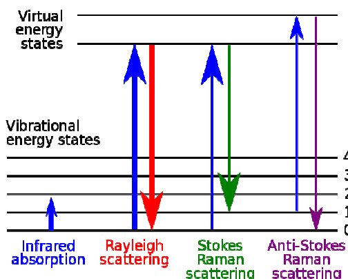
Figure II.13. Schematic diagram of the Raman effect showing the states involved in Raman signal. The line thickness is depicted depending on the intensity of different transitions (from [16]).
