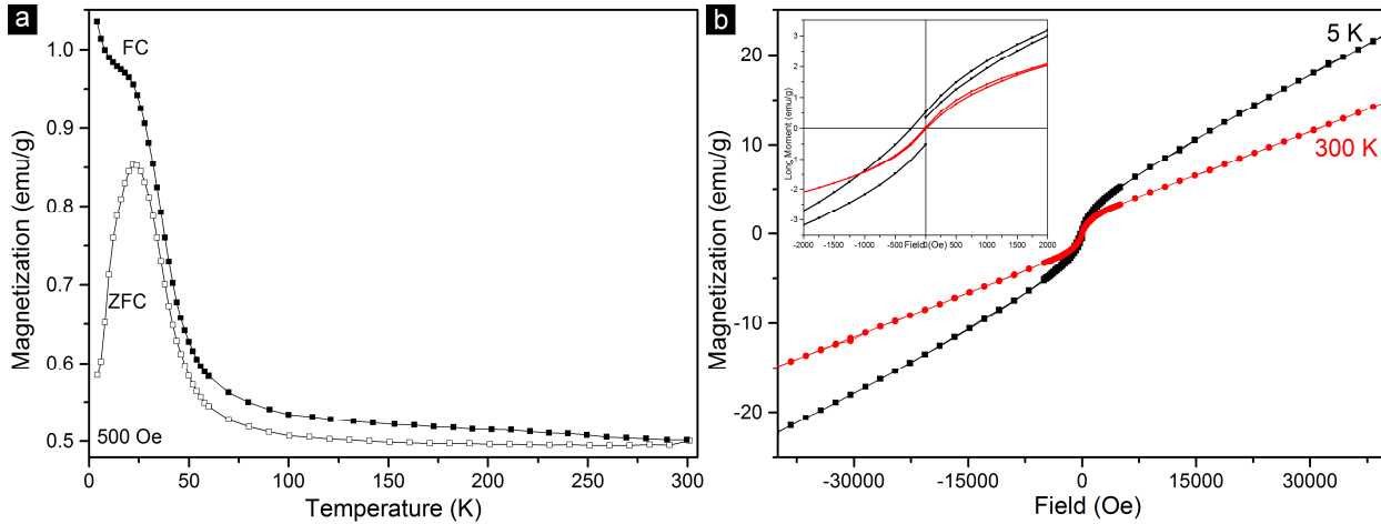
Figure IV.21. a) Temperature dependence of the magnetization ( M(T) ) for YMO-800-1-s1 film. Open (solid) symbols represent the M(T) taken in the ZFC (FC) mode; b) Field dependence of the magnetization ( M(H) ) at 5 and 300 K. Inset: enlargement of the M(H) curve in the low magnetization values.
