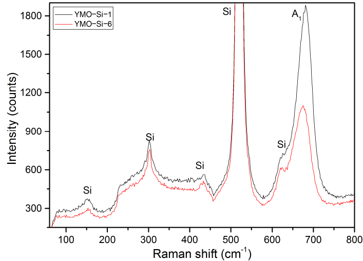
Figure IV.20. Raman spectra of YMO films deposited by PLD.
