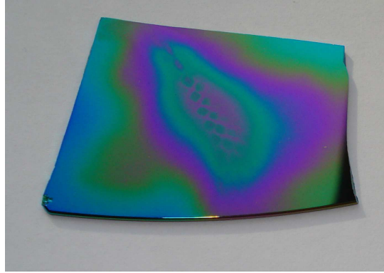
Figure III.2. An inhomogeneous \text{YMnO}_3/\text{Si} film deposited at high flow rate.
