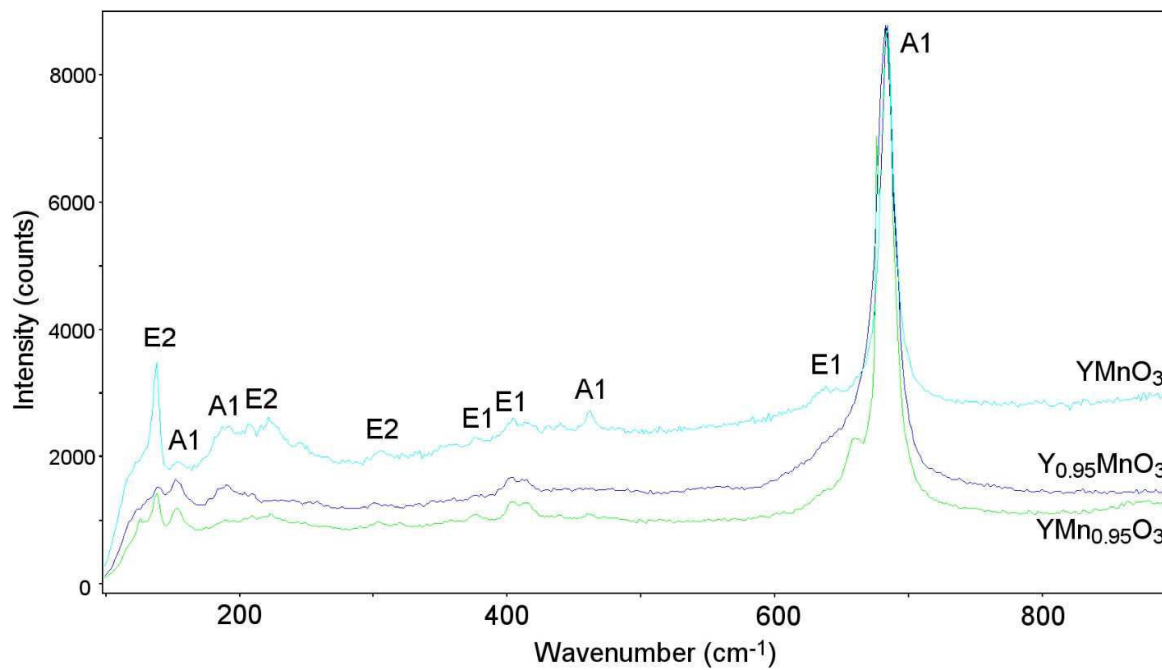
Figure C.3. Raman spectra of YMnO_3 , Y_{0.95}MnO_3 and YMn_{0.95}O_3 samples. The modes of the h -YMO phase are marked on each peak.
