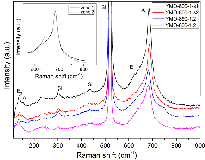
Figure IV.13. Raman spectra of h -YMO films elaborated in the horizontal PI-MOCVD device. Inset: A part of the Raman spectra collected in the two morphologically different regions (zone 1 and zone 2) of the YMO-800-1-s1 sample.
