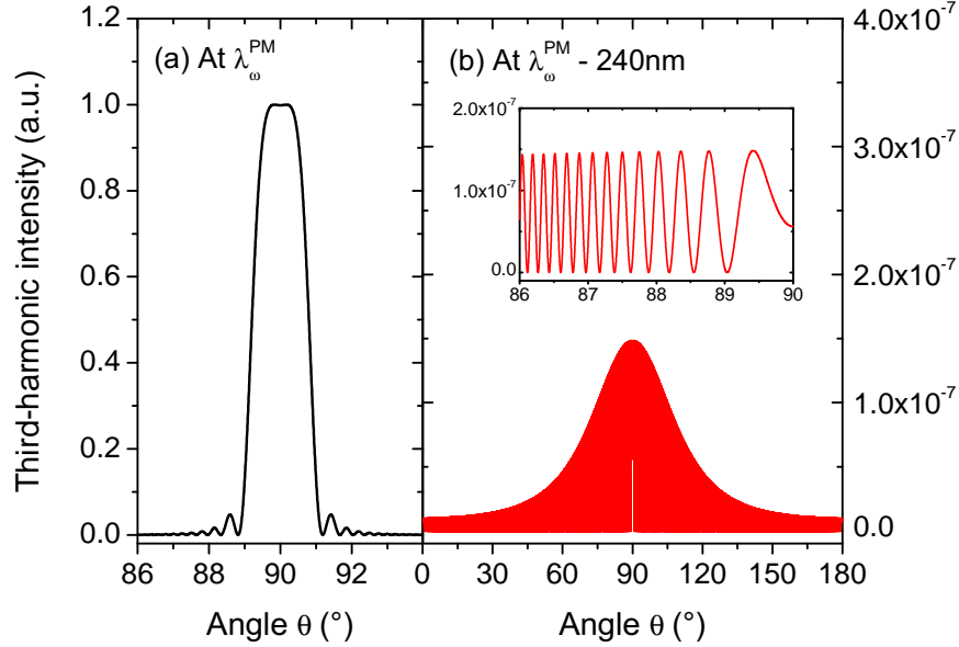
Figure 3.21 – THG angular spectrum. Calculations with monochromatic incoming fields at \lambda_{\omega}^{\text{PM}}(\theta = 90^{\circ}) = 1830 \text{ nm} (a) and \lambda_{\omega} = 1596 \text{ nm} = \lambda_{\omega}^{\text{PM}} - 240 \text{ nm} (b). The inset is a close-up view.
