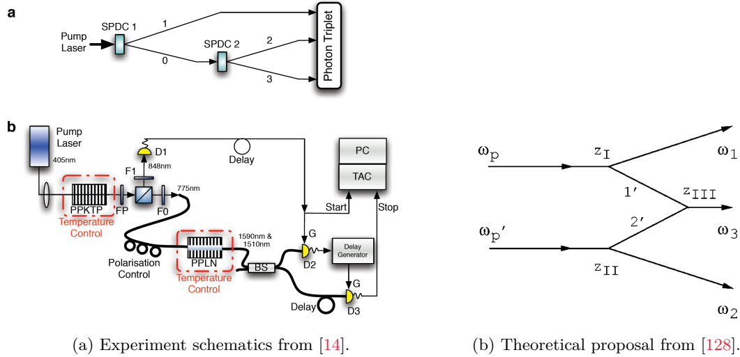
Figure 2.5 – Triplet photon generation from second-order interactions in cascade.
