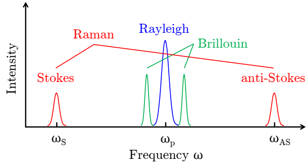
Figure 4.30 – Sketches of Raman and Brillouin scattering spectra.
