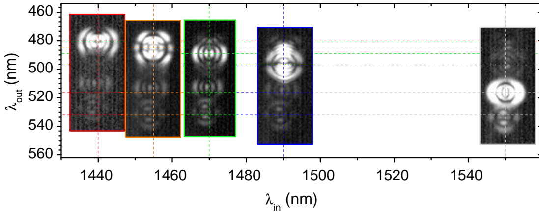
Figure 4.33 – Generated wavelengths in the visible range as a function of the input wavelengths (RedTide spectrometer), together with transverse clichés captured with a Edmund Optics camera, in a a = 2.19 \mu\text{m} fiber.
