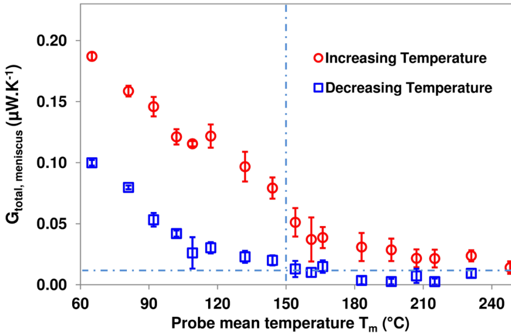
Figure 2.12. Total thermal conductance of the meniscus G_{total, meniscus} as a function of the Wollaston probe mean temperature T_m for the Ge sample ( T_a = 30 \text{ }^\circ\text{C} , RH = 40 \% ).
