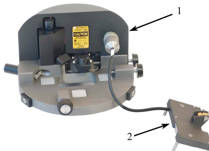
Figure A.2. Image of the 1- AFM head (universal head) and 2- probe adjustment unit (NTMDT/ User's manual).
