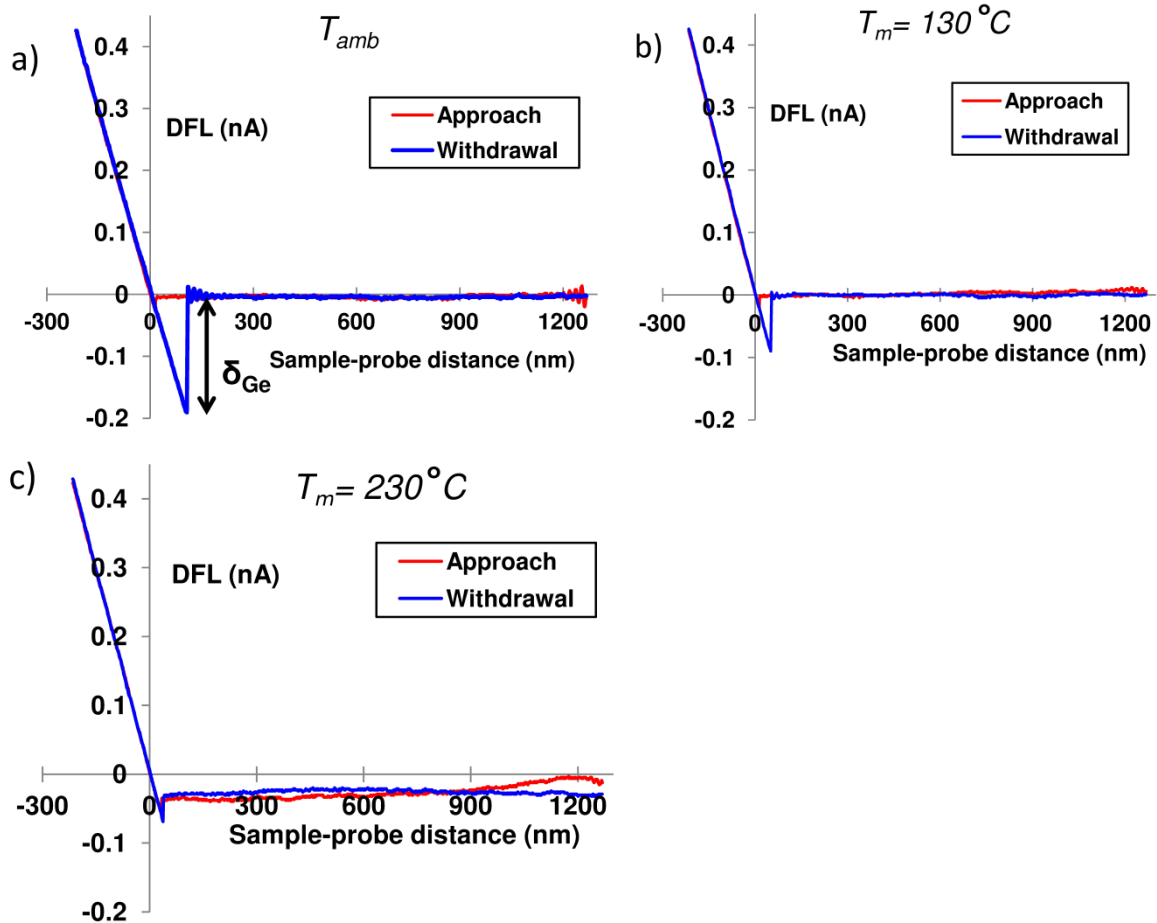
Figure 2.5. Spectroscopy curves performed on Germanium (Ge) for different probe mean temperature: (a) Ambient temperature, (b) T_m = 130\text{ }^{\circ}\text{C} and (c) T_m = 230\text{ }^{\circ}\text{C} .
