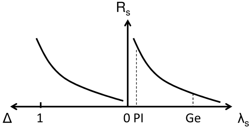
Figure 4.3. Schematic description of the variation of R_{sample} and \Delta as a function of \lambda_s .
