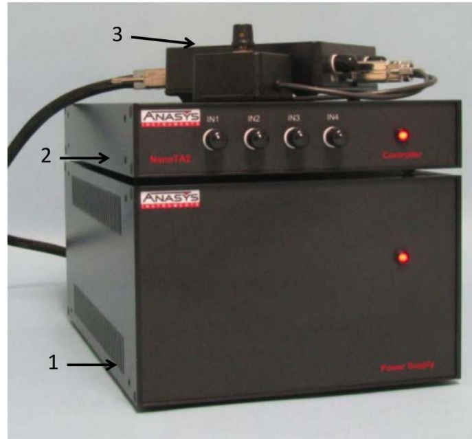
Figure A.6. The three parts of the NanoTA2: 1) Power supply, 2) Controller and 3) CAL Box.
