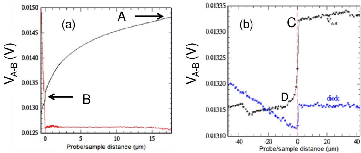
Figure 1.25. (a) Differential tension as a function of the probe/sample distance for a sample of Niobium ( \lambda= 59 \text{ W.m}^{-1}.\text{K}^{-1} ). A zoom at the contact zone is shown in Figure (b) [27].
