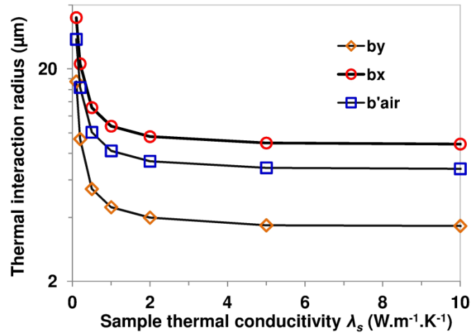
Figure 3.17. Variation of the thermal interaction radii b_x , b_y and b'_{air} as a function of the thermal conductivity \lambda_s .
