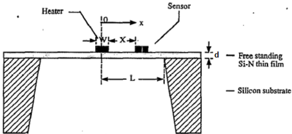
Figure 5.2. Schematic of the phase-shift method used by Zhang and Grigoropoulos [136].
