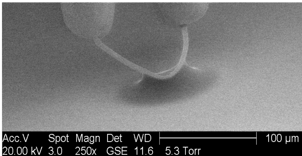
Figure 2.17. ESEM image of the water meniscus formed at the contact between Wollaston wire and germanium sample ( T_{substrate} \approx 2 °C, RH \approx 90 %).
