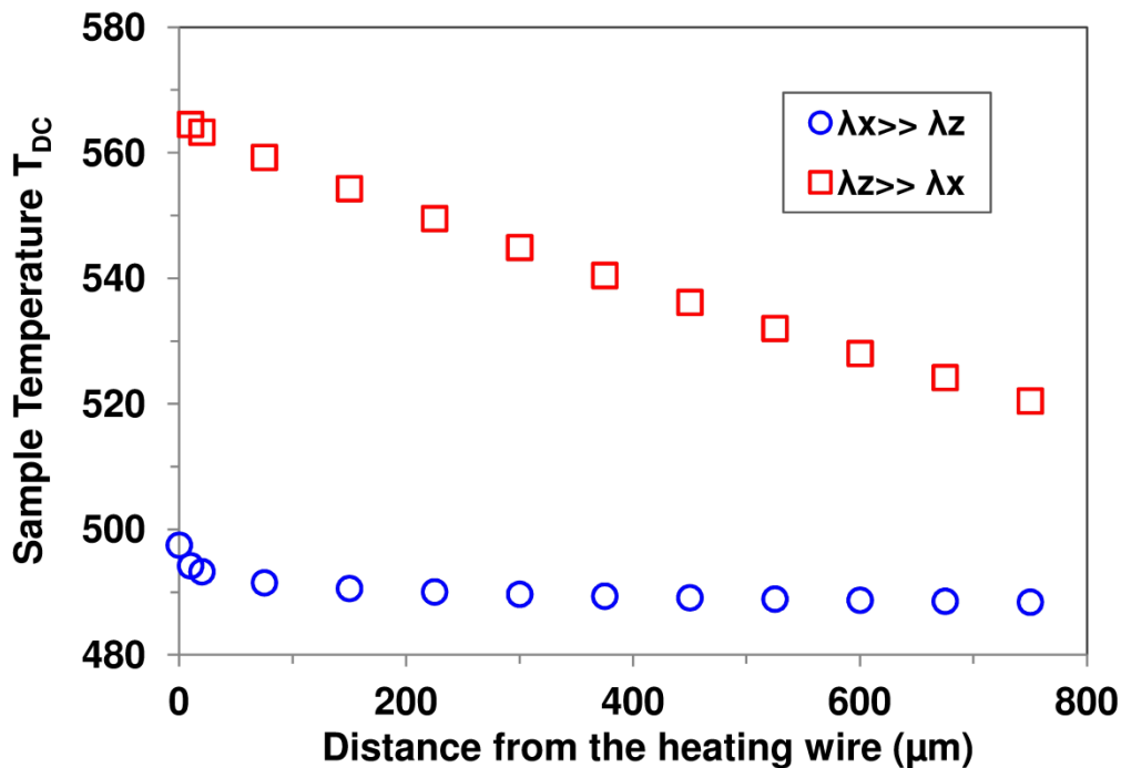
Figure 5.22. Simulated Variation of the sample temperature T_{DC} as a function of the distance from the heating wire for the two cases: \lambda_x \gg \lambda_z and \lambda_x \ll \lambda_z ( I_{ac}=60 \text{ mA} , \epsilon=1 , h=5 \text{ W.m}^{-2}.\text{K}^{-1} ).
