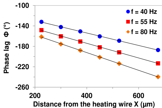
Figure 5.21. Experimental variations of the phase lag \phi as a function of the distance from the heating wire for I_{ac}=60 mA and for different frequencies.
