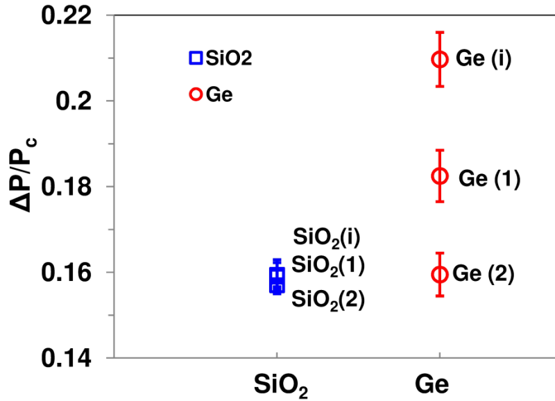
Figure 3.18. Variation of the thermal signal \Delta P/P_c for the different samples of different roughness parameters ( T_a = 25 °C, RH = 40 %).
