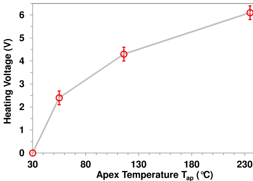
Figure 4.11. Heating Voltage (V) as a function of the apex temperature T_{ap} (°C).
