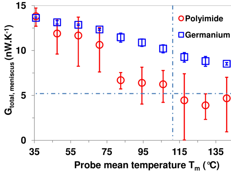
Figure 4.5. Variation of the total thermal conductance of water meniscus G_{total, meniscus} as function of the probe mean temperature T_m for the contact between KNT probe and samples of PI (red circles) and Ge (blue squares).
