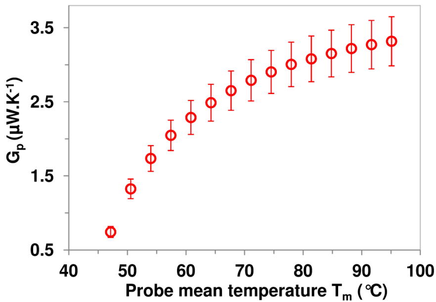
Figure 4.6. Thermal conductance of the probe as a function of the probe mean temperature T_m ( P=0.28 \text{ mbar} , T_a=30 \text{ }^\circ\text{C} ).
