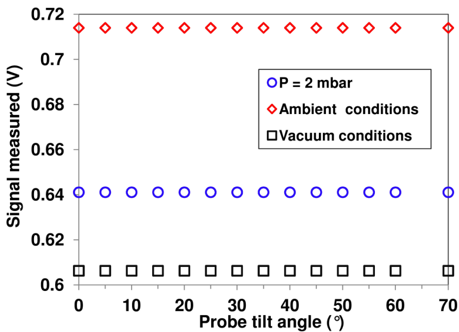
Figure 3.9. Voltage of the probe in different conditions for different tilts of the probe.
