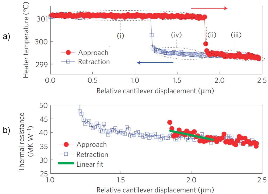
Figure 1.18. Approach and retraction curves between a flat-punch tip and taC sample a) Variation of the heater temperature b) Evaluation of the thermal resistance at the tip-sample contact ( P \approx 6 \times 10^{-6} mbar) [58].
