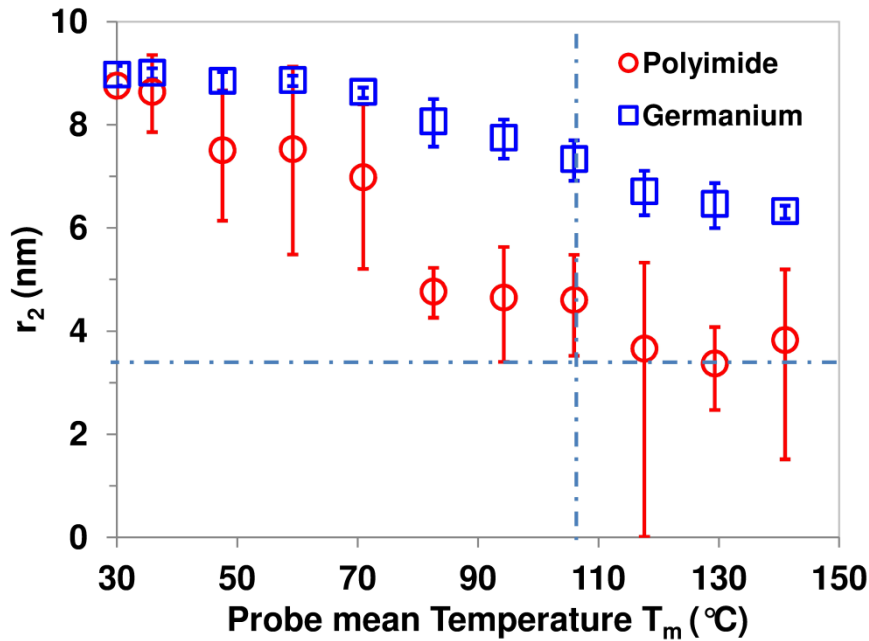
Figure 4.4. Variation of the larger radius r_2 of the meniscus as function of the probe mean temperature T_m for the contact between KNT probe and samples of PI (red circles) and Ge (blue squares).
