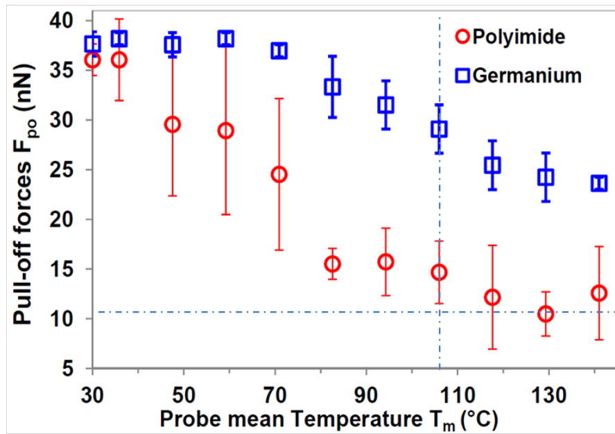
Figure 4.1. Variation of the pull-off forces as a function of the probe mean temperature for the contact between KNT probe and samples of PI (red circles) and Ge (blue squares).
