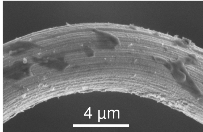
Figure 2.9. Scanning Electron Microscopy SEM image of a Wollaston wire probe apex.
