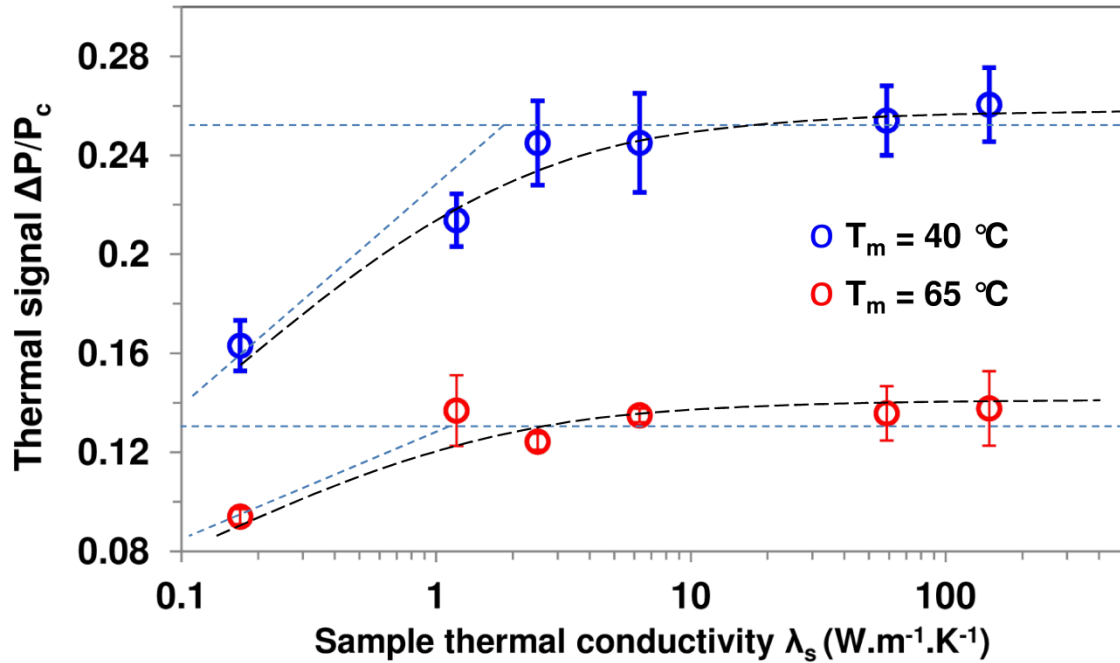
Figure 4.9. Thermal signal \Delta P/P_c as function of the sample thermal conductivity \lambda_s for T_m=40 °C (blue circles) and T_m=65 °C (red circles) ( T_a=30 °C, RH=40 %).
