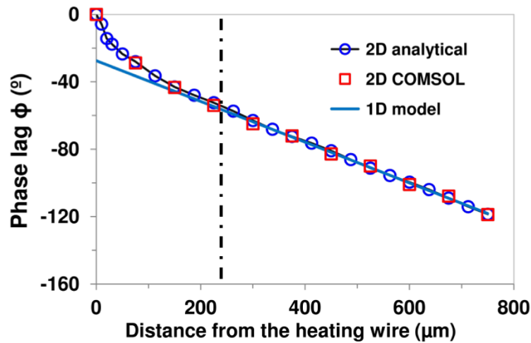
Figure 5.17. Comparison of the phase lag ( ^{\circ} ) between the analytical model, 2D numerical simulations and 1D approach ( I_{ac}=60 mA, \epsilon=1 and h=5 W.m -2 .K -1 ).
