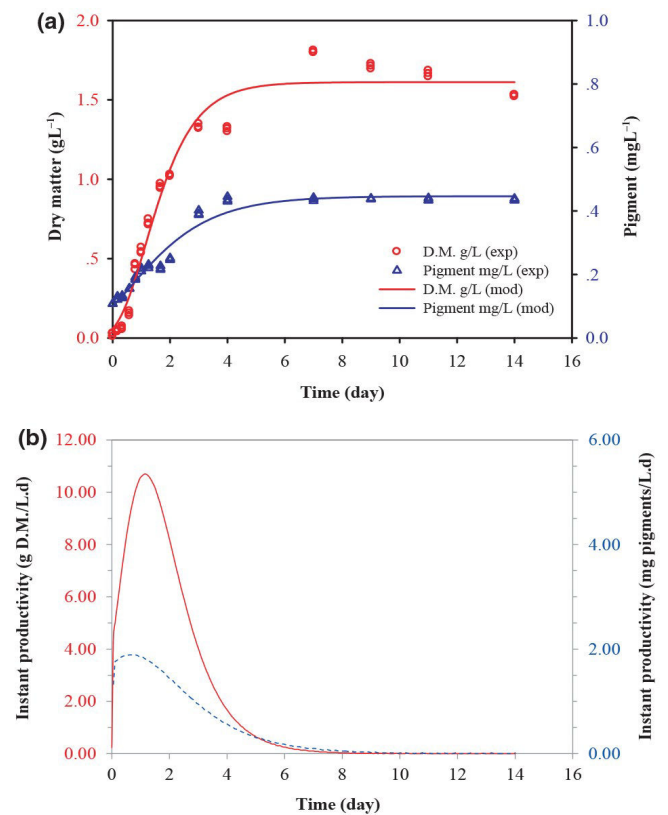
Fig. 5. Growth and pigment production by Arthrobacter arilaitensis Po102 cultivated in milk ingredient-based liquid medium. (a) Curves of dry matter and pigment production based on the experimental data and calculated using Gompertz model (○ = dry matter g L -1 from experimental data, — = dry matter g L -1 from calculating, ○ = pigment mg L -1 from experimental data, — = pigment mg L -1 from calculating). (b) Instant productivity of biomass and pigment calculated from the model curves (— = g dry matter L -1 day -1 , ---- = mg pigments L -1 day -1 ).
