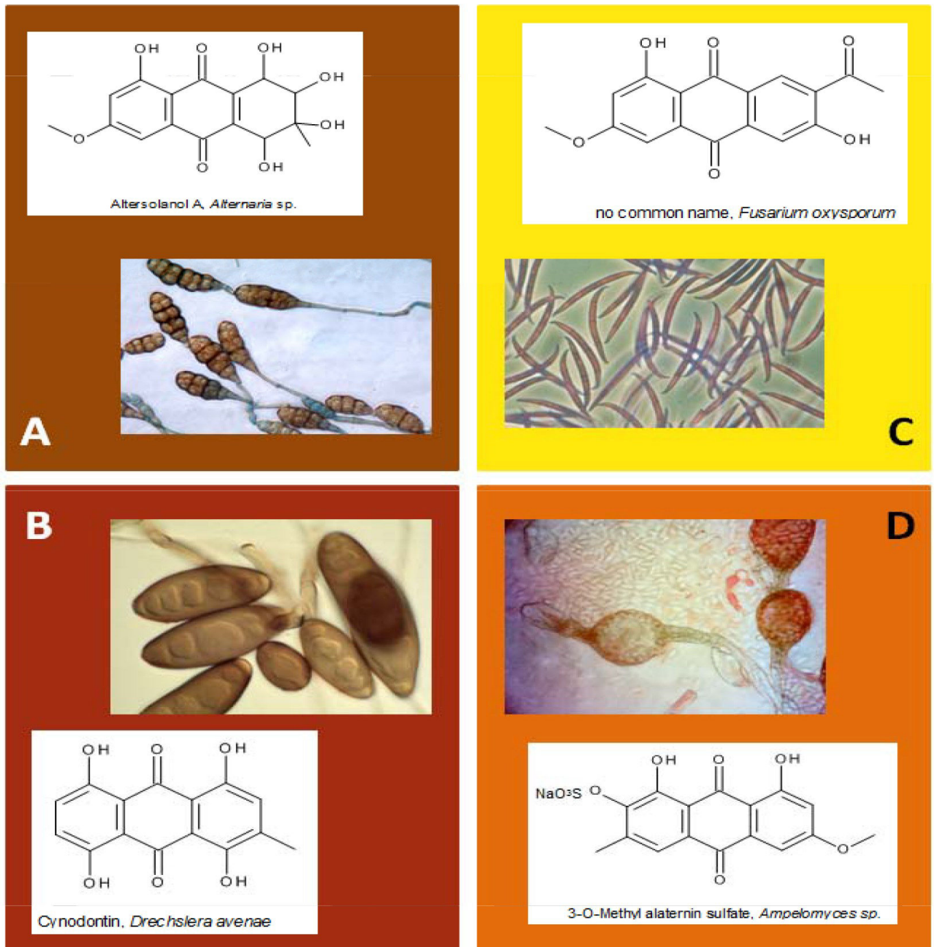
FIGURE 12.3 Some anthraquinones from fungal origin: (a) maroon, (b) bronze, (c) yellow, (d) red-orange.
