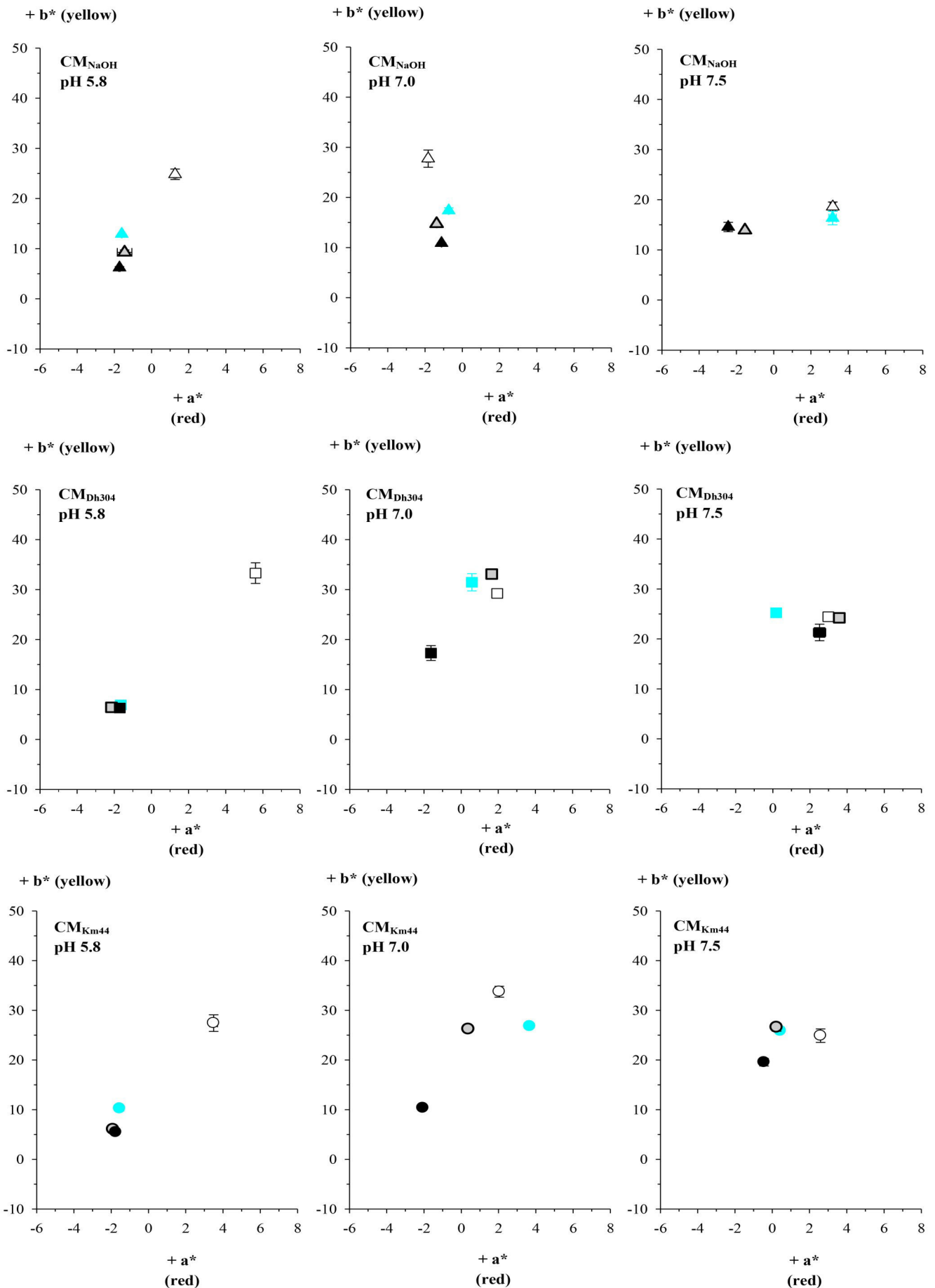
Fig. 1. Detailed positions of biofilms produced by Arthrobacter arilaitensis when projected in the CIE L^*a^*b^* colorimetric scale (bars indicate standard deviations). The concentration of additional NaCl (w/v) is presented as symbols following; \square = 0%, \blacksquare = 2%, \blacksquare = 4% and \blacksquare = 8%.
