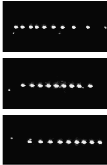
Fig. 4.15 Observation of a breathing mode: the displacement of the chain as a whole from the center with the inter-particles spacing increasing as one goes farther from the center of the array [38].
