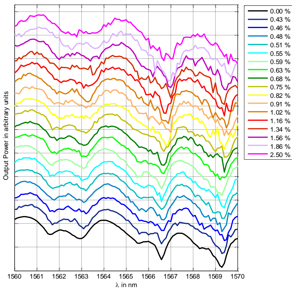
Fig. 3.21 The spectra of DI water and DI water containing 0.5\mu\text{m} polystyrene microspheres with different concentrations ranging from 2.5 % to 0.43 %. Note that the power reference has been changed for every curve in order to superpose them for better comparison.
