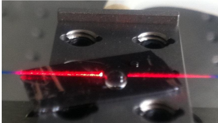
Fig. 5.11 A photograph for the droplet resonator on its substrate and the lensed fiber pair used to inject and collect the light.
