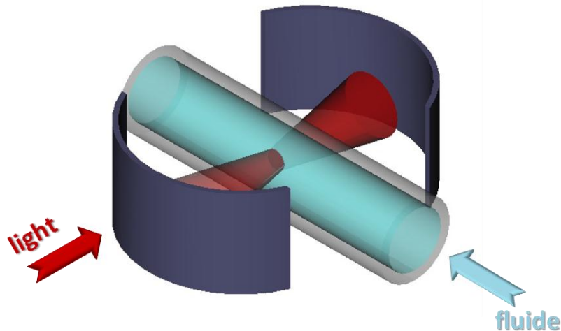
Fig. 2.16 Schematic diagram of the cylindrical Fabry-Pérot cavity with the micro tube inside.
