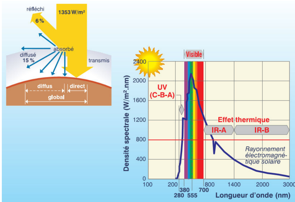
FIGURE 1.10 – Spectre du soleil (Herde and A.Liébard, 1996-2004)
