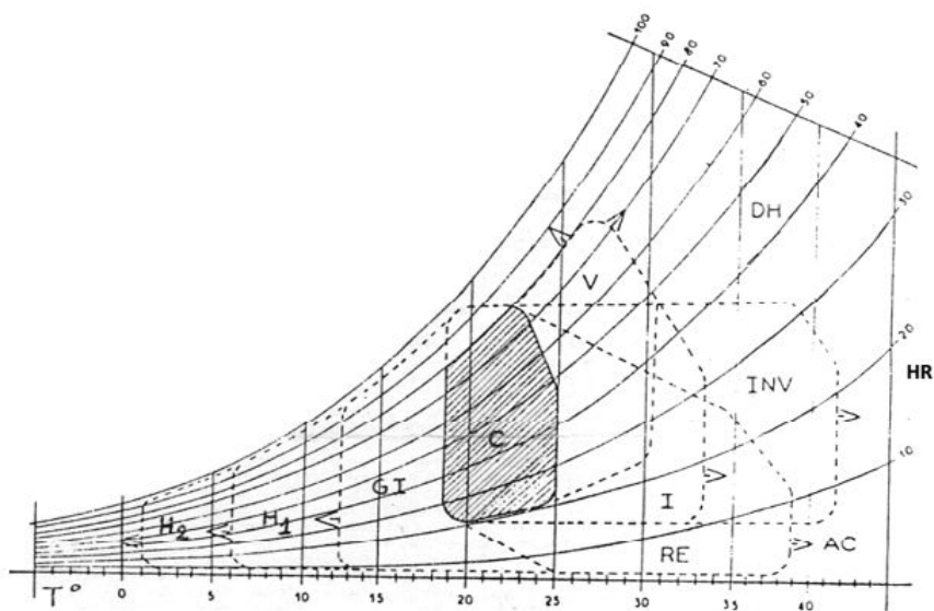
FIGURE 1.14 – Diagramme de Givoni
