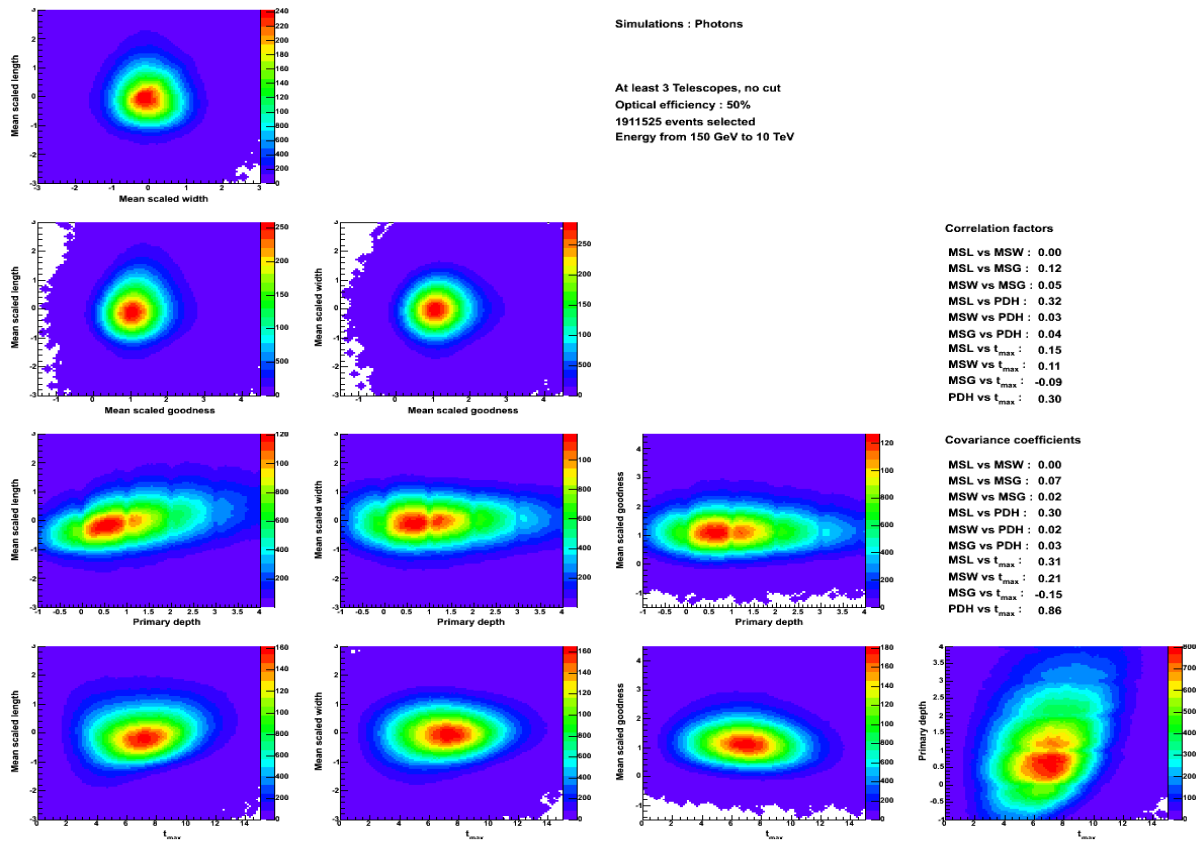
Figure 2.30: Correlations between the different discriminant variables for point-like gamma, using 3 telescopes for reconstruction. See figure 7.6 for comments.
