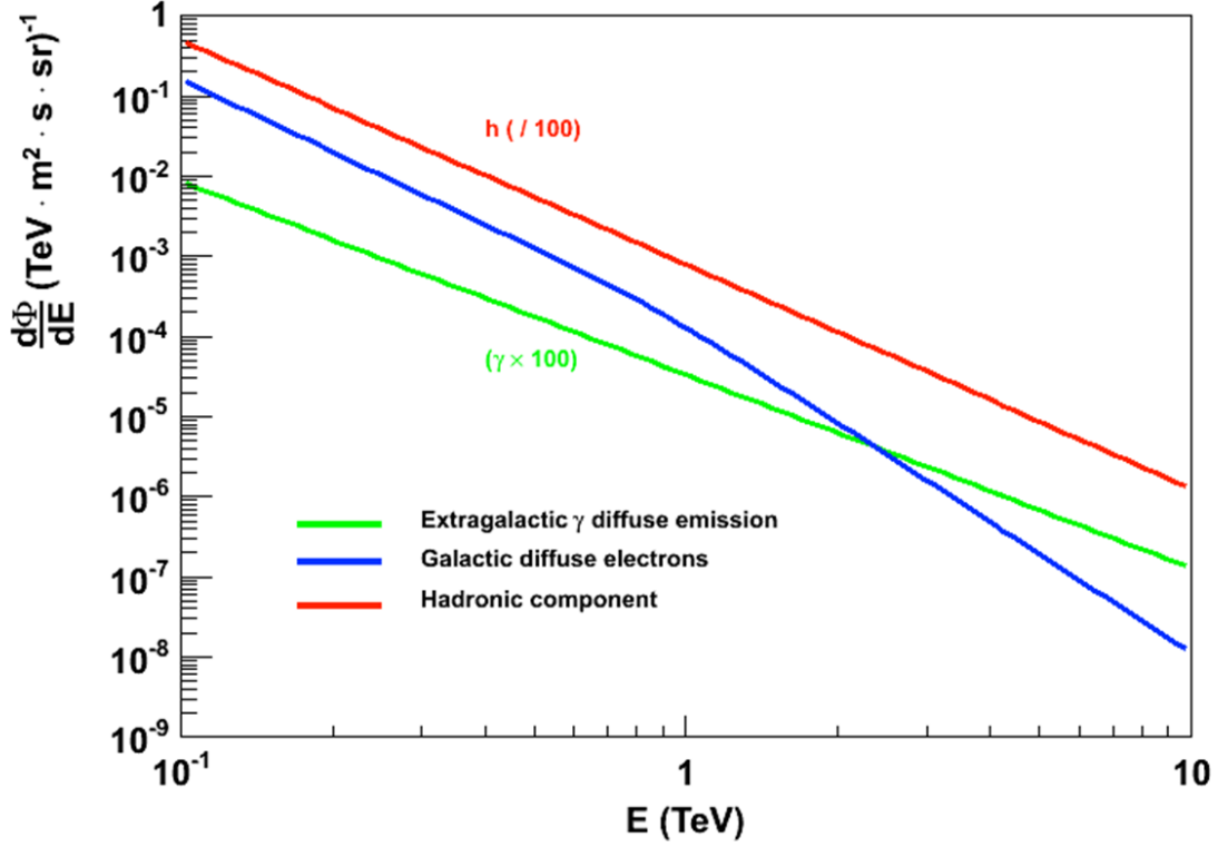
Figure 4.4: Extrapolation of the diffuse components to the energy domain of the HESS experiment. Red, green and blue curves represent the hadron, gamma and electron spectrum respectively. Hadron and gamma fluxes have been scaled.
