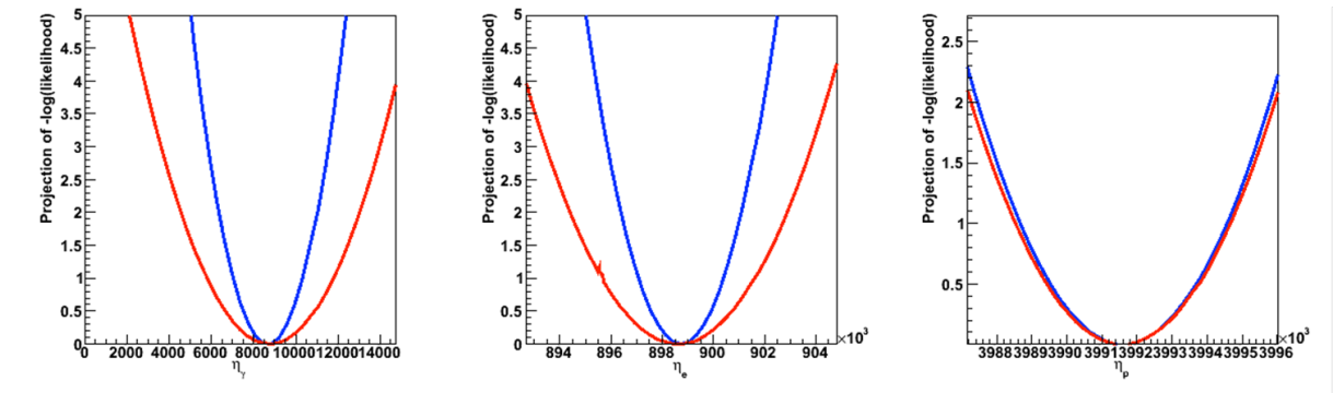
Figure 6.4: Evolution of the maximum likelihood value for the three fractions around the best-estimated value (in blue) and the profile likelihood (in red) if one parameter (fraction) is scanned and the others are free to vary around the best estimate value.
