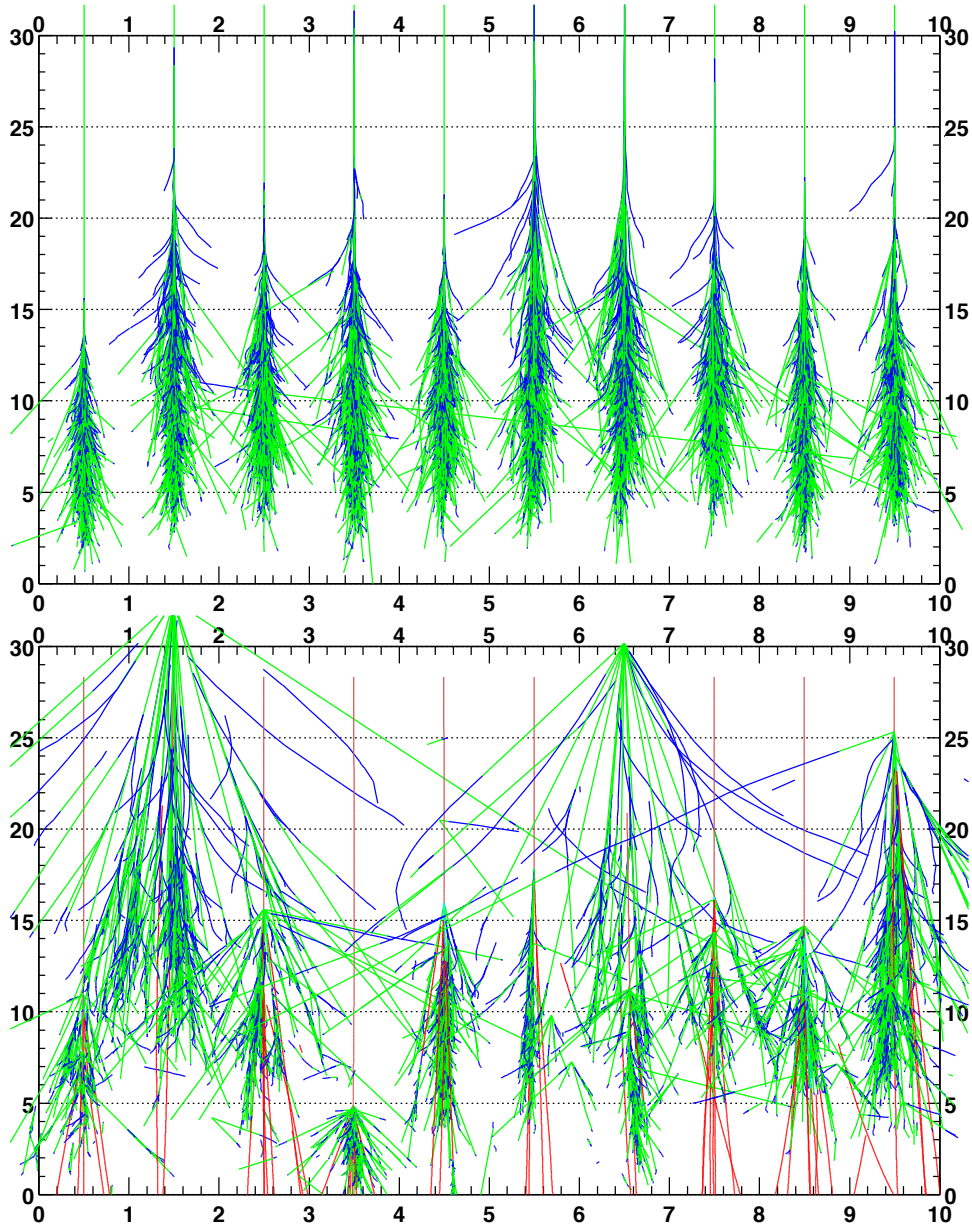
Figure 1.6: Comparison between ten electromagnetic (top) and hadronic (bottom) showers from 300 GeV primary particles. The electromagnetic showers have less fluctuations than hadronic ones and are much more similar. Both axes are given in kilometers. The vertical scale gives the altitude with respect to sea level. Taken from [14]
