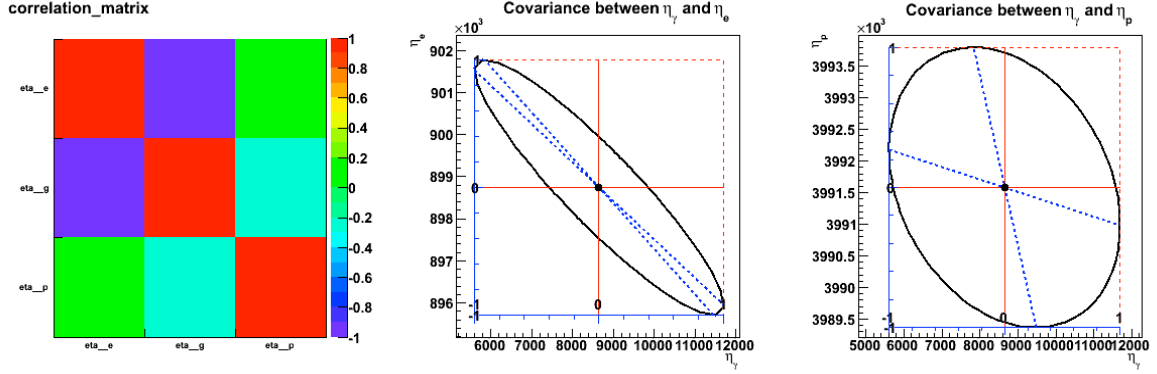
Figure 6.3: Representation of the correlation between the three free parameters of the fit (left plot). Covariance ellipses between electron and gamma fractions (center) and gamma and hadrons (right).
