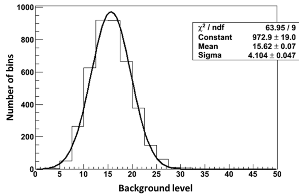
Figure 5.10: The distribution of the background level is fitted with a gaussian function. Its mean value is \mu = 15.62 , with a standard deviation \sigma = 4.1 .
