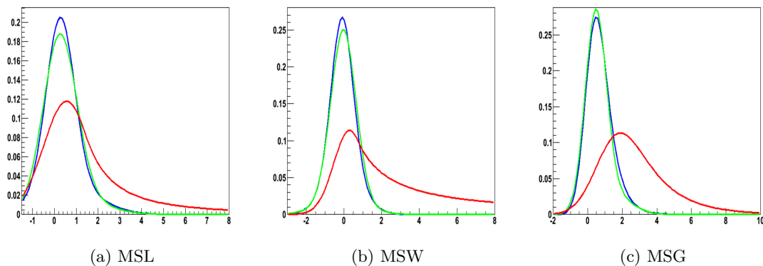
Figure 6.1: Above plots represent the PDF functions adjusted on simulated data for mean scaled length (left), mean scaled width (middle) and mean scaled goodness (right) discriminant variables. Protons are in red, electrons in blue are superimposed on the photons in green which can be difficultly distinguished. The functions used for the fit are given in appendix C.
