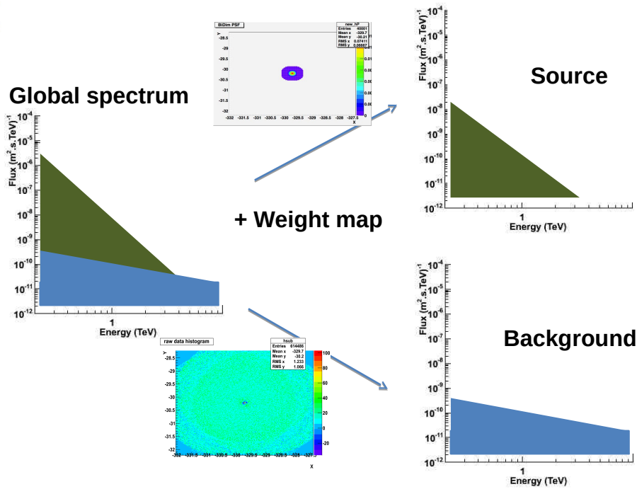
Figure 5.11: Diagram representing the way the global spectrum is separated into two spectra, one for the source and one for the diffuse emissions, using the weight map given by the source modelization.
