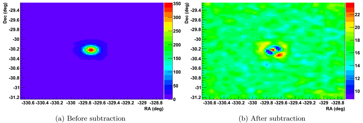
Figure 5.5: FOV of PKS2155-304 before (left) and after (right) subtraction of the convoluted PSF at the position of the source. The AGN can be seen in the left plot. On the right plot is the FOV after the subtraction. A residue of about 17% at the center of the source is noticed, as well as small depressions (3%) at the edge of the source.
