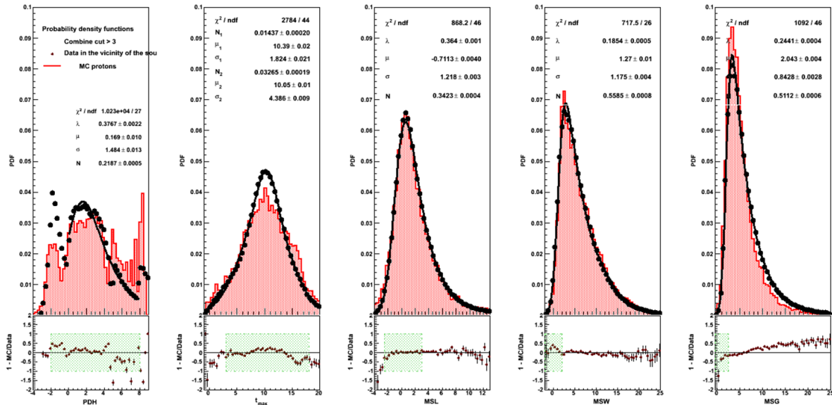
Figure 2.23: Histograms of the PDF extracted from data outside the source in black dots and those computed with the simulations in red. The ratio between both is represented under each plot. The functions in black are the fit of the data but were not used for the analysis. A lower cut of 3 in the CombineCut2 variable was applied to further purify the sample in protons. The green boxes correspond to the interval in which the plots for the signal are represented in figure 2.24. Neither the intervals of these plots nor the ones for the signal regions represent the data selection. The latter is explained in section 2.4 and tries to take into account as best as possible the intervals in which the ratios of these histograms and those in the signal region are close to 1.
