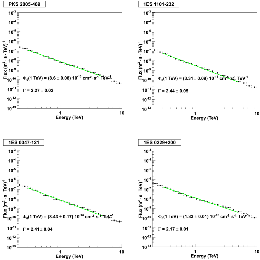
Figure 5.13: Energy spectra for the four selected weakly emitting AGNs, with a region of radius 0.3^\circ for the convoluted PSF fit. The flux at 1 TeV, \Phi_0(1 \text{ TeV}) , and spectral index \Gamma are given for each source after fitting the spectrum with a power law function between 0.3 and 5 TeV.
