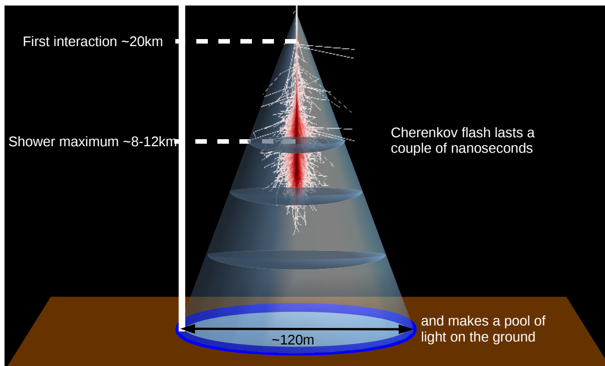
Figure 1.7: Maximum of shower development and first interaction point represented on a shower image. Credit: M. Daniel
