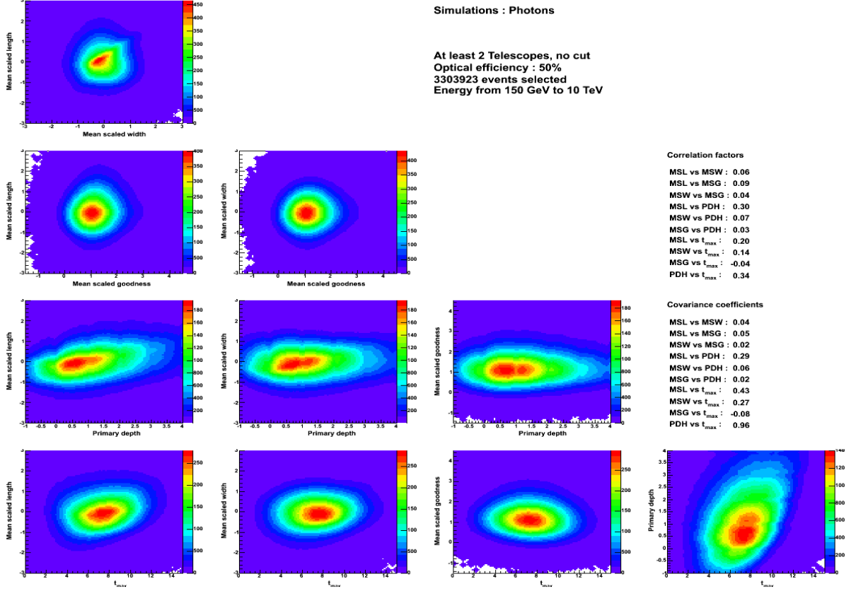
Figure 2.29: Correlation plots between the discriminant variables for point-like gamma. The strong correlation between MDH and PDH can be observed in the bottom right plot. The eliminated values of PDH can also be seen. Moreover, in the correlation plot of MSL against MSW, the effect of a bad reconstruction can be noticed as a small correlation. This disappears when including 3 telescopes for the reconstruction, as in figure 2.30.
