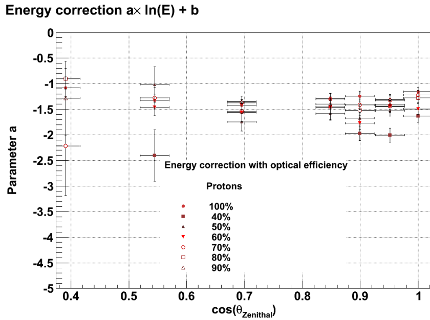
Figure D.9: Parameter a_e for each optical efficiency and zenith angle for simulated protons. See figure D.7 for comments.
