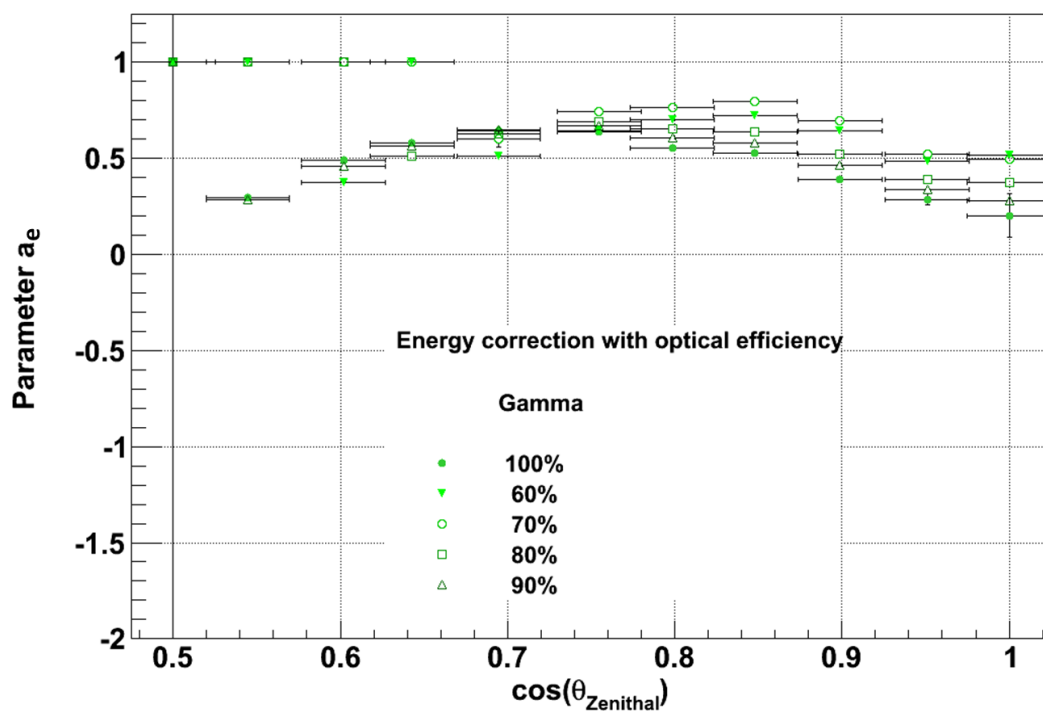
Figure 2.18: Parameter a_e for each optical efficiency and zenith angle for simulated point-like gamma. The values at 1 correspond to fits that did not converge. At high zenith angles, the optical efficiency doesn't influence the determination of the fit and t_{max} appears to follow the expected evolution as a function of the energy. However, when the zenith angle decreases, lower energies are included depending on the optical efficiency (which also influences the energy threshold) and a variation of the a_e parameter is seen. Thus, it seems that low energies introduce a divergence from the law 2.11.
