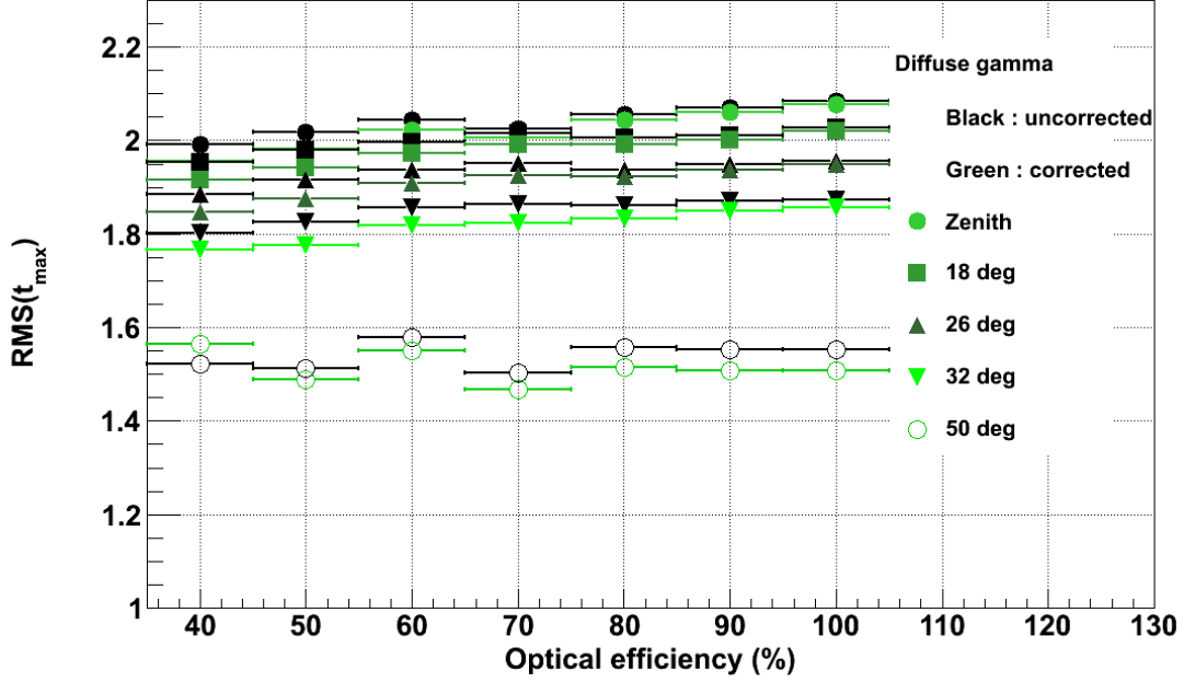
Figure 2.17: Effect of zenith correction on the rms of MDH for simulated diffuse gamma and all optical efficiencies. The correction does not seem to influence the width of the distribution. However, the evolution of the latter with the zenith angle will limit the effect of the correction. The narrower distributions, represented by a smaller rms for high zenith angles are explained by the fact that the energy threshold increases, so only showers with higher energies will trigger. These are known to have a better reconstruction and hence angular resolution.
