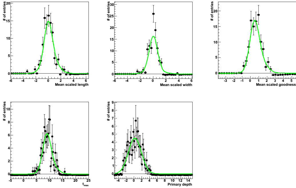
Figure 7.1: Gamma PDF (in green) for each discriminant variable, obtained when applying the sPlot technique on simulated data (in black).
