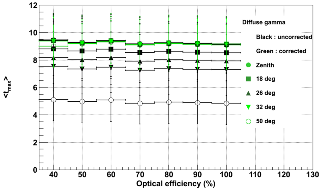
Figure 2.16: Effect of zenith correction on the mean value of MDH for simulated diffuse gamma and all optical efficiencies. Before correction (in black), the mean value of MDH is different for each zenith angle. After correction (in green) they are superimposed.
