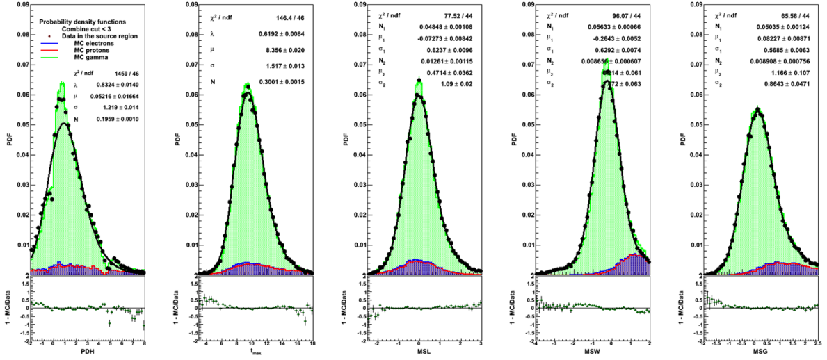
Figure 2.24: Histograms of the PDF extracted from data inside a radius of 0.3^\circ around the source in black dots and those computed with the simulations in green. The ratio between both PDF is represented under each plot. In red are the protons and blue, these added to electrons. The functions in black are the fit of the data but were not used for the analysis. An upper cut of 3 in the CombineCut2 variable was applied to purify the sample in gamma and electrons. The intervals do not correspond to the data selection. See comment in figure 2.23 and section 2.4 for more on it.
