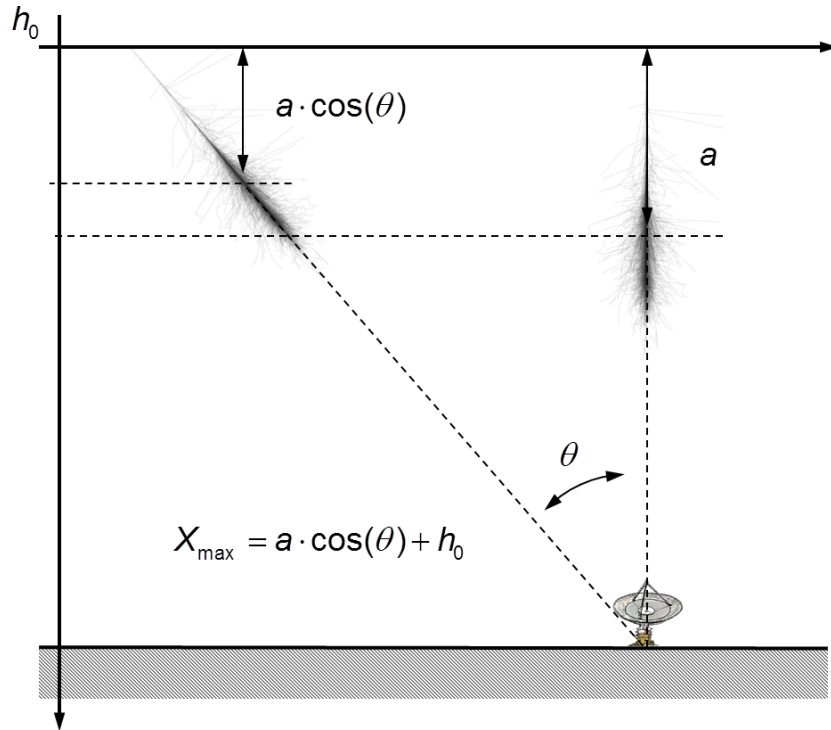
Figure 2.13: Zenithal angle dependency of MDH.
