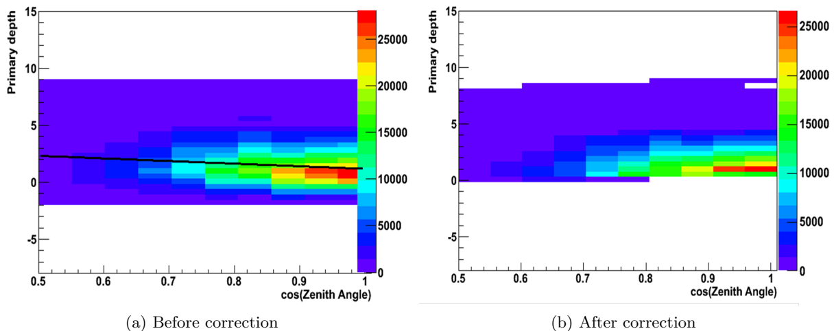
Figure 2.15: PDH as function of the zenith angle, before (left) and after (right) corrections for simulated point-like photons. The black line corresponds to the fit of the profile of the histogram.
