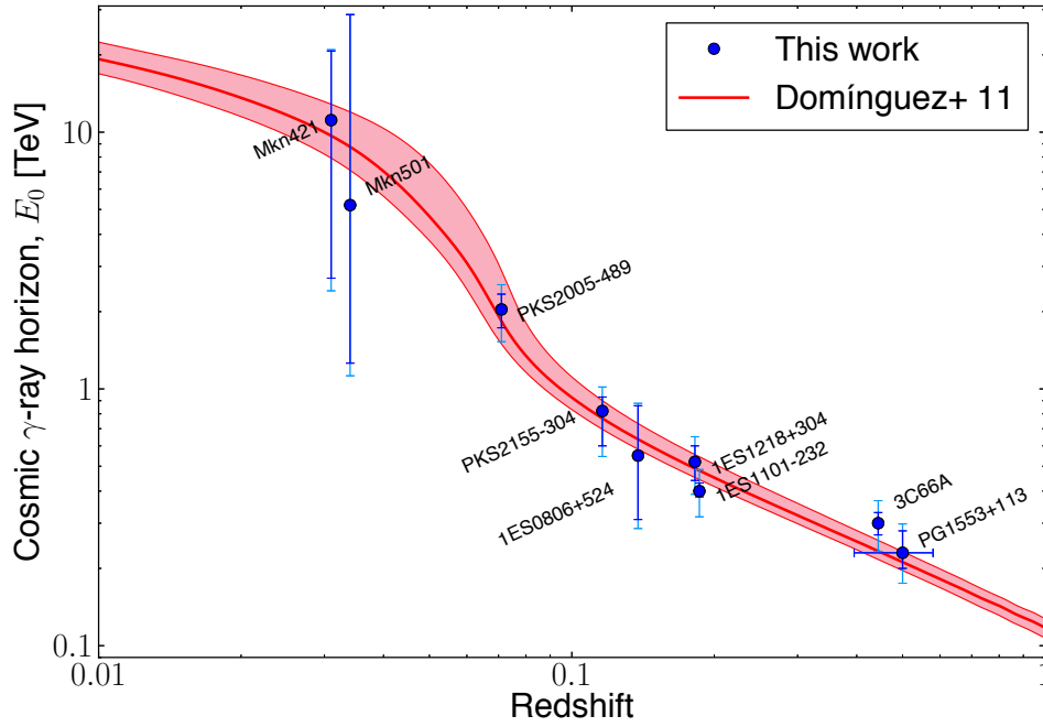
Figure 3.5: The gamma horizon in energy as a function of redshift, for different AGN. The results are compared to those from a previous publication by the same group. Taken from [43]
