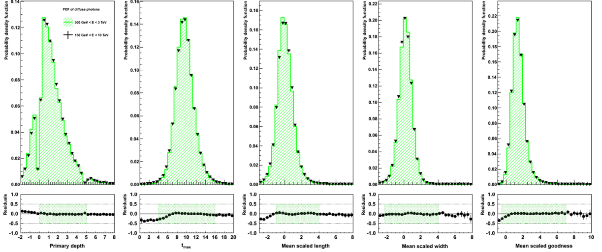
(a) PDF for diffuse gamma in different energy domains
