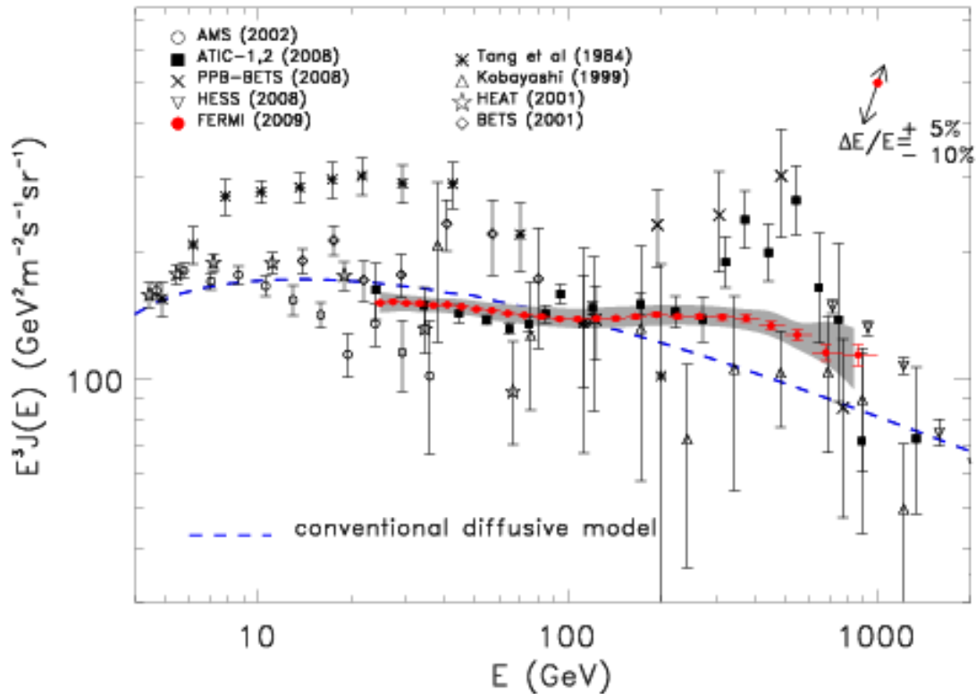
Figure 4.5: Electron total flux as seen by ATIC, PPB-BETS, H.E.S.S. and Fermi between \sim 10 and \sim 10^3 GeV. The first two experiments observed an anomaly invalidated later by the Fermi data. [72]
