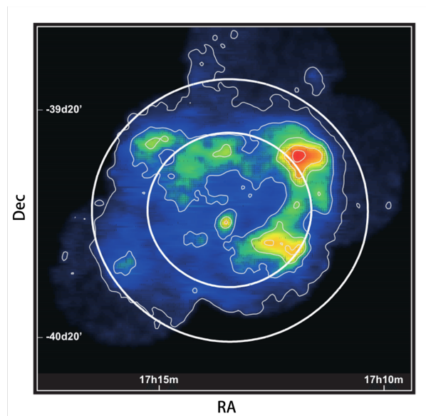
Figure 5.2: The supernova remnant RXJ1713.7-3946 is an extended source with a noticeable correlation between its emission in gamma-rays (H.E.S.S. map in full color scale) and X-rays (thin gray contours, corresponding to ASCA data in the 1-3 keV range [94]). The comparable angular resolution for both sets of telescopes makes the comparison easier. The superimposed thick white contours indicate the 94% and 98% levels of the detection efficiency weighted HESS exposure, given by the product of relative detection efficiency and the observation time. Credit [95].
