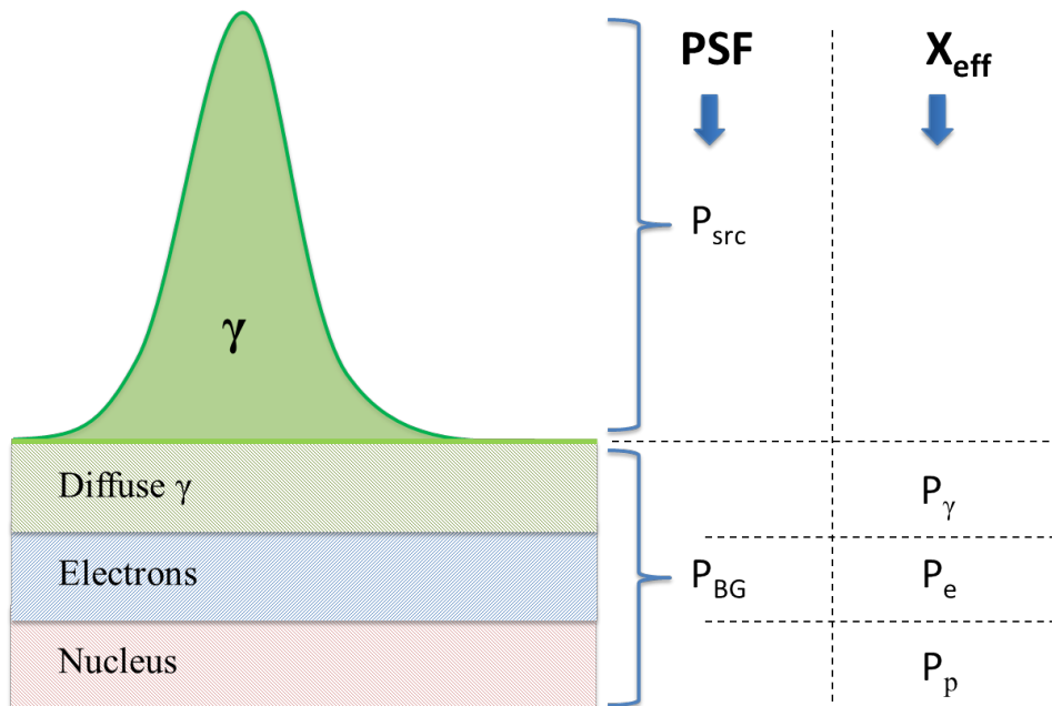
Figure 6.5: Diagram representing the way the probabilities are assigned to each component in the field of view.
