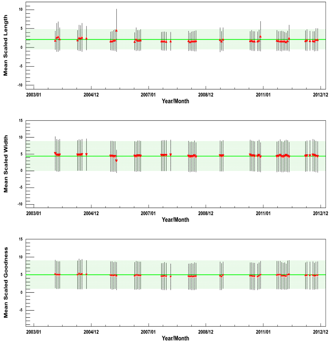
Figure 2.26: Time dependency of the discriminant variables MSL, MSW and MSG. See figure 2.25 for comments.
