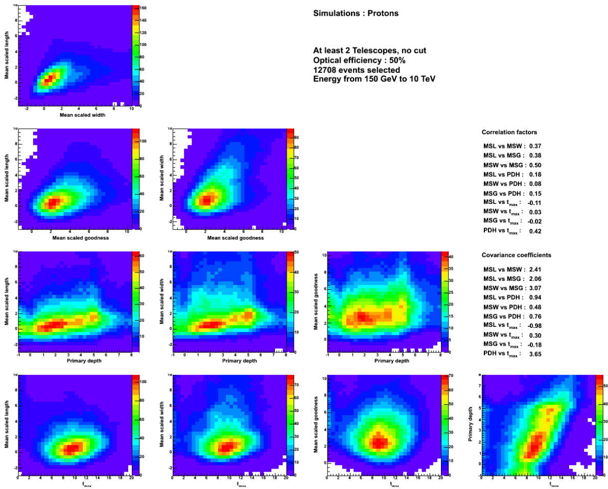
Figure E.3: Correlation plots for protons reconstructed with 2 telescopes.
