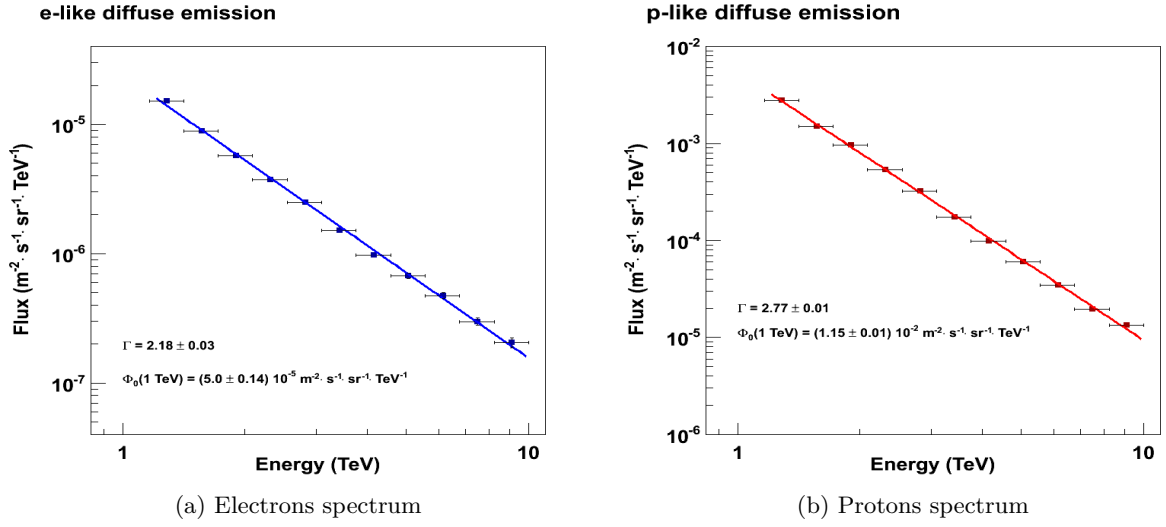
Figure 6.8: The spectra of the diffuse electrons and protons. The obtained values for the electrons' flux at 1 TeV is (4.995 \pm 0.138(\text{stat})) \cdot 10^{-5} \text{m}^{-2} \text{s}^{-1} \text{TeV}^{-1} \text{sr}^{-1} while its corresponding spectral index is \Gamma = 2.18 \pm 0.03(\text{stat}) . For protons, the flux at 1 TeV and spectral index are, respectively, (1.151 \pm 0.011(\text{stat})) \cdot 10^{-2} \text{m}^{-2} \text{s}^{-1} \text{TeV}^{-1} \text{sr}^{-1} and \Gamma = 2.77 \pm 0.01(\text{stat}) .
