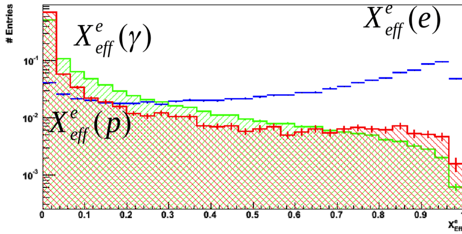
Figure 6.6: X_{eff}^e distributions for simulated gamma (green), electrons (blue) and protons (red).
