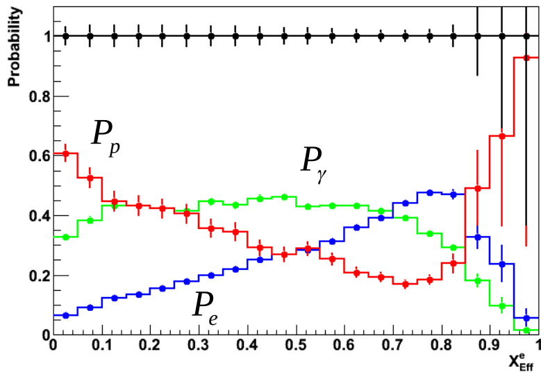
Figure 6.7: Distributions of the probabilities obtained using the X_{eff}^e estimator for simulated protons (red), electrons (blue) and gamma (green). Their total sum is shown in black.
