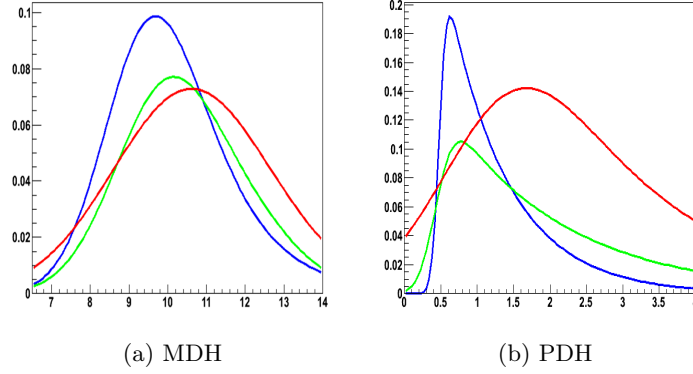
Figure 6.2: Plots represent the PDF functions adjusted on simulated data for the depth of the maximum of the shower expansion (left) and primary interaction position (right) discriminant variables. Protons are in red, electrons in blue and photons in green. The functions used for the fit are given in appendix C. As the three types of particles have different intervals for these two variables (see section 2.4), the smallest intervals were chosen for the representation.
