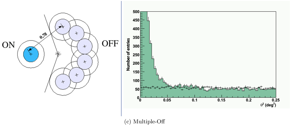
Figure 2.12: Examples of background subtraction techniques. Top: sky maps illustrating the ring-background (left) and template model (right) subtraction methods. Bottom: the multiple-off regions subtraction method shown on a sky map (left) along with the corresponding calculated \theta^2 for the Crab Nebulae where the estimated background can be seen.
