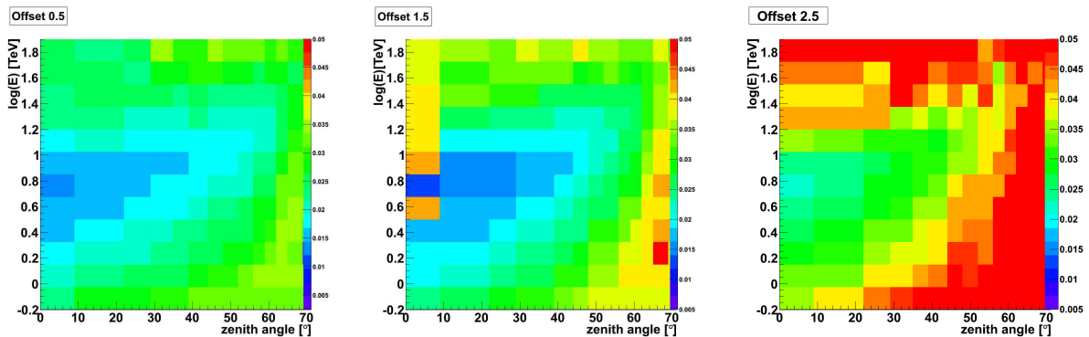
Figure 2.4: Color coded width of the PSF ( \sigma ) for all zenith angles and energies, and 3 off-axis angles: 0.5^\circ , 1.5^\circ and 2.5^\circ . It can be seen that at larger off-axis angles, the PSF broadens, only slightly for the first two but significantly for the last one, specially for high zenith angles and energies. At zenith angles above around 50^\circ , the angular resolution worsens rapidly (PSF becomes wider), while remaining relatively stable below that value. Concerning the energy, for values from around 1 TeV to 15 TeV, the angular resolution is the best, with a small improvement around 6 TeV. However, outside this region it decreases quickly. It can be noticed that for showers to be better reconstructed at higher zenith angles, they need higher energies as well, due to the energy threshold. Taken from [23].
