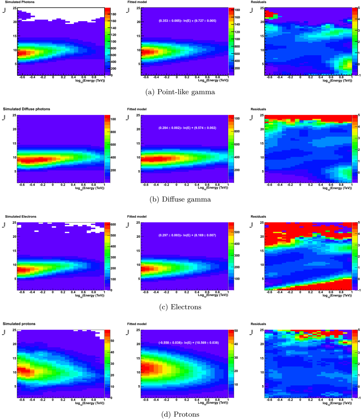
Figure 2.19: Distributions of MDH as a function of the energy for simulated point-like photons, diffuse photons, electrons and protons. For point-like gamma and electrons, the distributions correspond to a zenith angle of 0^\circ , whereas for diffuse gamma and protons, the shown plots were obtained for data including all zenith angles. On the left plots are distributions before the energy correction. The distributions are narrower around an inclined slope, which reflects the logarithmic dependency. The plot in the middle represent the model fitted on the simulations, which gives the value for parameter a_e . On the right plot is the residue after subtraction of the fitted model from the initial distribution. It can be seen that the model represent well the initial distributions, for in the area where there is data the residue is negligible.
