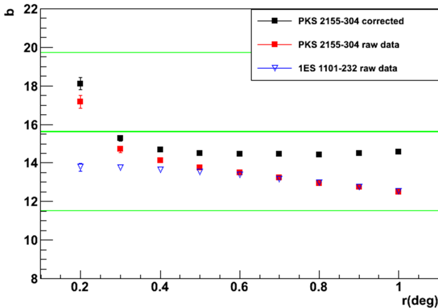
Figure 5.9: Background values resulting from the fit of PKS 2155-304 (squares) and 1ES 1101-232 (triangles) in their respective fields of view. The fit is performed on a circular region around the maximum of the source for nine different radii, from 0.2^\circ to 1^\circ with steps of 0.1^\circ . In the case of PKS 2155-304, the fit was tested on data both with (black) and without (red) acceptance correction. Its effect is to flatten the obtained background values above a radius of 0.5^\circ whereas the uncorrected ones decrease along with the detector's acceptance. The effect of the strong luminosity of PKS 2155-304 during its flare can be seen when taking small regions for the fit, as the source influences the background determination and the effect of the stable acceptance in the camera cannot be seen. However, for weak sources, this feature appears clearly. A systematic bias can be observed with respect to the computed average value of the background outside the source (green line), which is later discussed.
