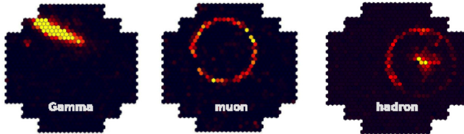
Figure 2.6: Examples of shower images induced by different particles. A primary gamma will generally produce an elliptical shape whereas a hadron's image will more complex, for hadronic showers are usually very irregular. The characteristic ring of a muon going through the camera is also shown.
