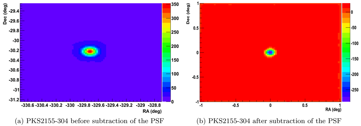
Figure 5.4: The FOV of PKS 2155 before (left) and after (right) subtraction of the PSF. The AGN can be seen in the left plot, while on the right one a clear depression appears, signifying that the PSF is two narrow compared to the source.
