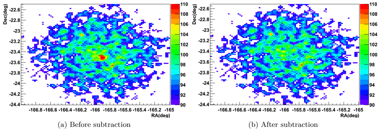
Figure 5.6: FOV of 1ES 1101-232 before (left) and after (right) subtraction of the convoluted PSF at the position of the source. The AGN can be seen in the left plot whereas on the right plot it has neatly been subtracted, leaving only background.
