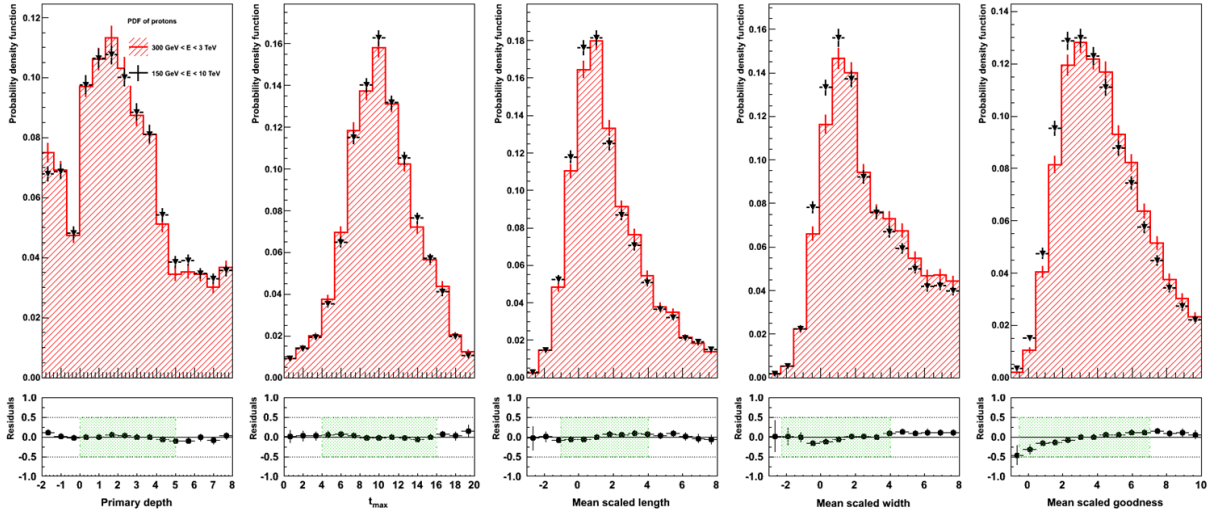
(b) PDF for protons in different energy domains
