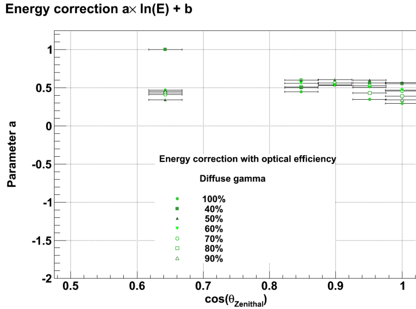
Figure D.7: Parameter a_e for each optical efficiency and zenith angle for simulated diffuse gamma. The values at 1 correspond to fits that did not converge. The evolution as a function of the zenith angle and optical efficiency are mainly due to effects of energy threshold. Indeed, as commented in section 2.1.5.3, for higher values of the zenith angle and optical efficiency, the energy threshold increases, thus excluding low energy showers and thus influencing the distribution of MDH as a function of the energy.
