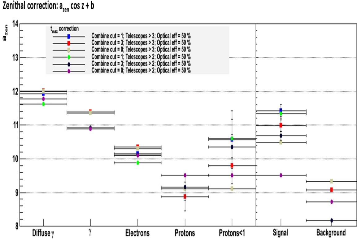
Figure 2.22: Zenith angle corrections for simulations (left) and data (right) with different cuts on the CombinedCut2 variable, written as CombinedCut2=1 and CombinedCut2=3 . These are upper cuts in the case of diffuse gamma, gamma and electron simulations, and were also applied on proton simulations, grouped under "protons<1" and the signal region. Concerning proton simulations and the background region, CombinedCut2=3 corresponds to a lower cut. The value of the correction with no cut on CombinedCut2 ( CombinedCut2=0 ) was also added. Simulations were taken for a 50% optical efficiency, which is the nearest to the computed efficiency in the data. Two telescope cuts were used for comparison. On the data inside the signal region, the looser the cut, the more background is included and the correction gets closer to that of protons and background. A hard cut will make the data dominated by point-like gamma, and the corrections between these simulations and the data in the signal region become comparable. Even the simulated protons' correction becomes closer to that of gamma.
