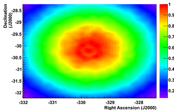
Figure 5.7: Sky map representing the acceptance of the instrument in the field of view of PKS 2155-304.
