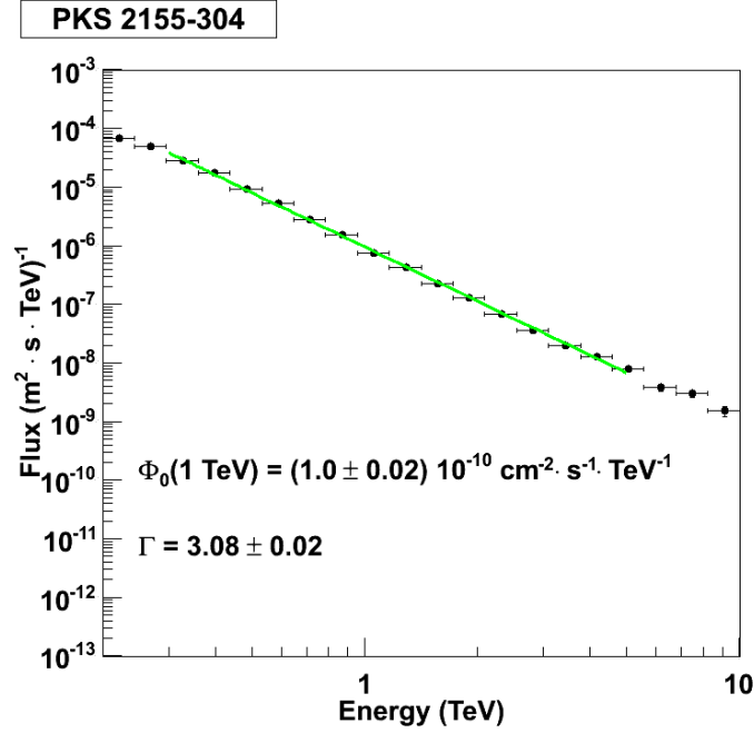
Figure 5.12: PKS 2155-304 spectrum fitted with a power law function between 0.3 and 5 TeV. A region of radius 0.8^\circ was used for the convoluted PSF fit.
