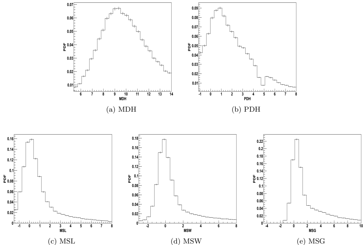
Figure 2.21: Distributions extracted from the data set inside a 0.3 degree radius. The PDF of point-like gamma can be seen, with a narrow peak, superimposed over the protons which create the wider asymmetric tail of the distribution.
