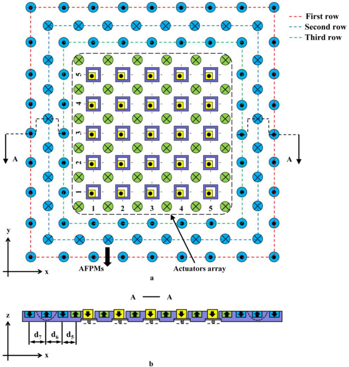
Fig II-4: Schematic layout of the digital actuators array
