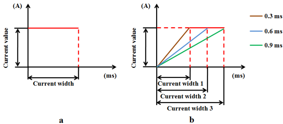
Fig III-20: Driving current type: a. rectangular shape current, b. trapezoidal shape
