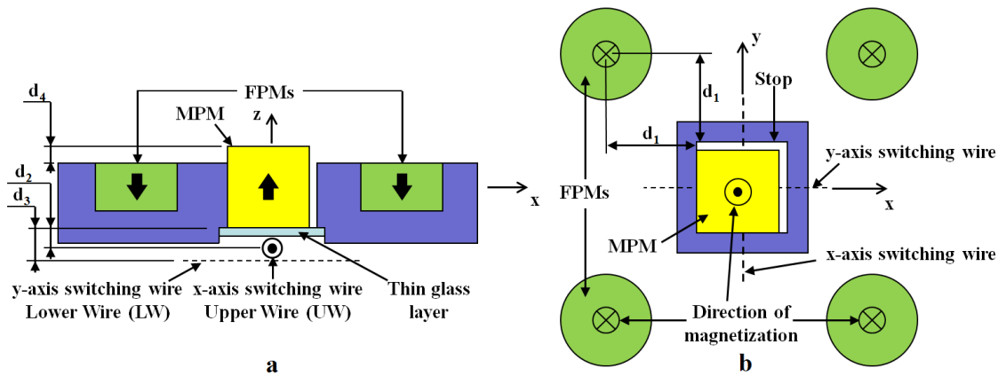
Fig II-1: a. Side view of the elementary digital actuator b. Top view of the elementary digital actuator
