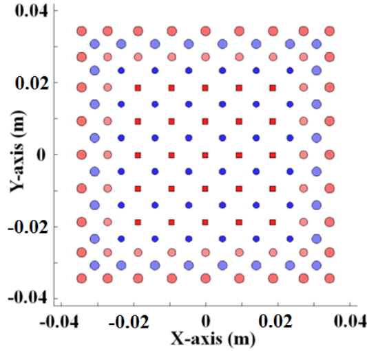
Fig IV-9: Geometry of the selected MO optimal solution
