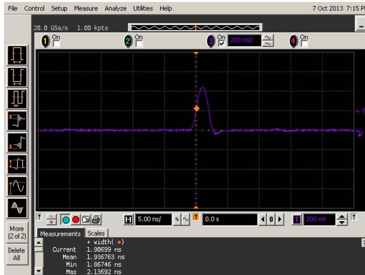
Figure 6.1: First-order fault injection attack — proof of concept.
