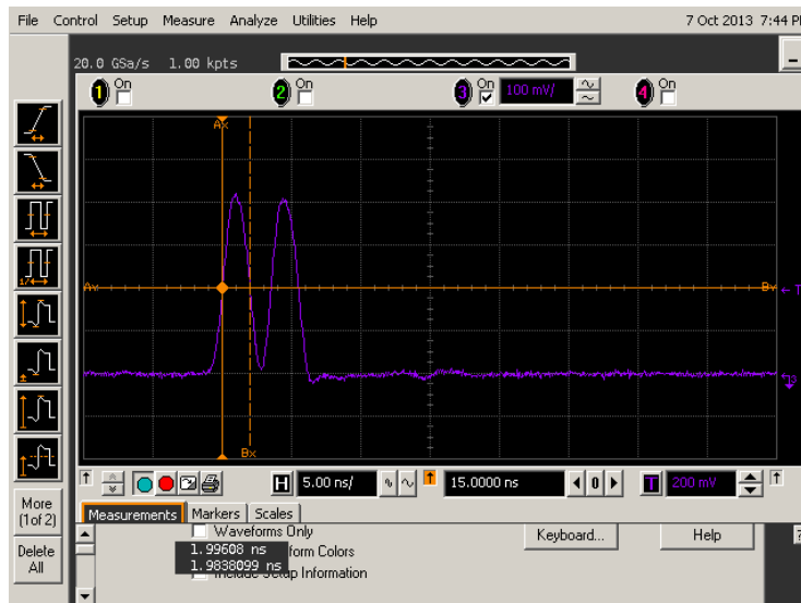
Figure 6.2: Second-order fault injection attack — proof of concept.
