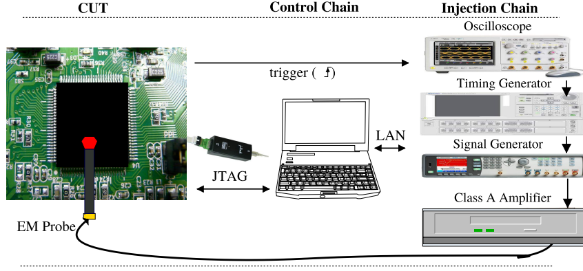
Figure 8.6: EMFI platform.
