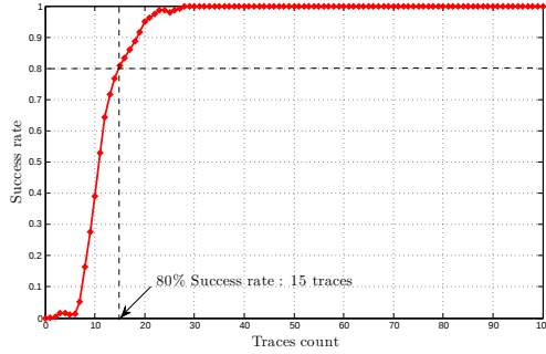
Figure 4.7: Attacking AES on the ATmega163 : success rates.
