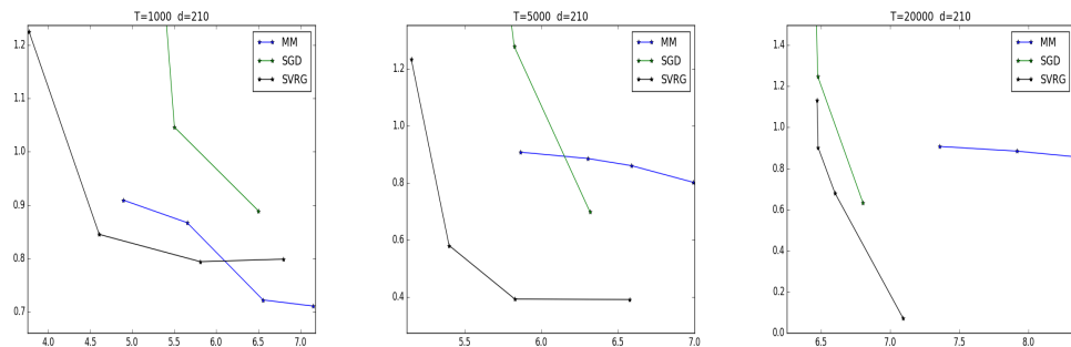
Figure VI.4 - \log(\varepsilon) as a function of the execution \log(t) for D = 210 and T = 1000 ( N/D = 2670 ) (left), T = 5000 ( N/D = 13300 ) (middle) and T = 20000 ( N/D = 53000 ) (right).
