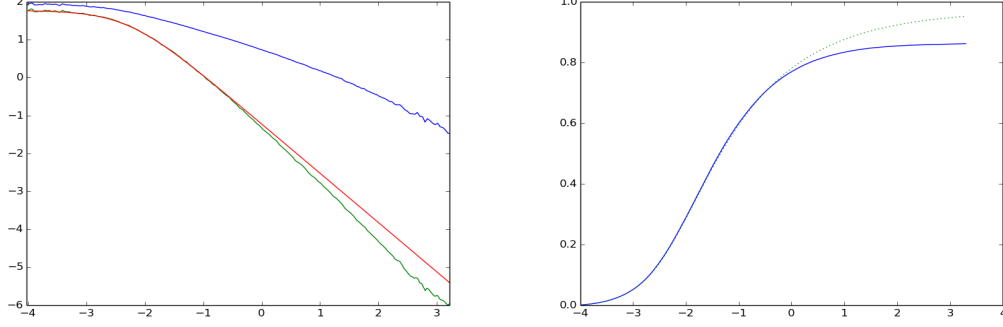
Figure V.1 - Left: Estimation of the conditional law g and kernel \phi in the case of a 1-dimensional Hawkes of size T = 10^7 seconds, with parameters (12). The estimation of g is performed using the procedure described in Appendix V.A using h_{min} = 1ms , h_{max} = 1000s and h_\delta = 0.05 , and kernel estimation is performed using algorithm of Section 9 with Gaussian quadrature followed by the change of variable (10) ( K = 200 , T_{min} = 1ms , T_{max} = 2000s and thus \delta = 0.077 ). The three curves correspond to \log_{10} - \log_{10} empirical conditional law (blue), theoretical kernel (red) and estimated kernel (green) for 200 quadrature points. Right: Cumulated theoretical kernel \int_0^t \phi(s) ds (green dots) and cumulated estimated kernel \int_0^t \tilde{\phi}(s) ds (blue) as a function of \log_{10}(t) .
