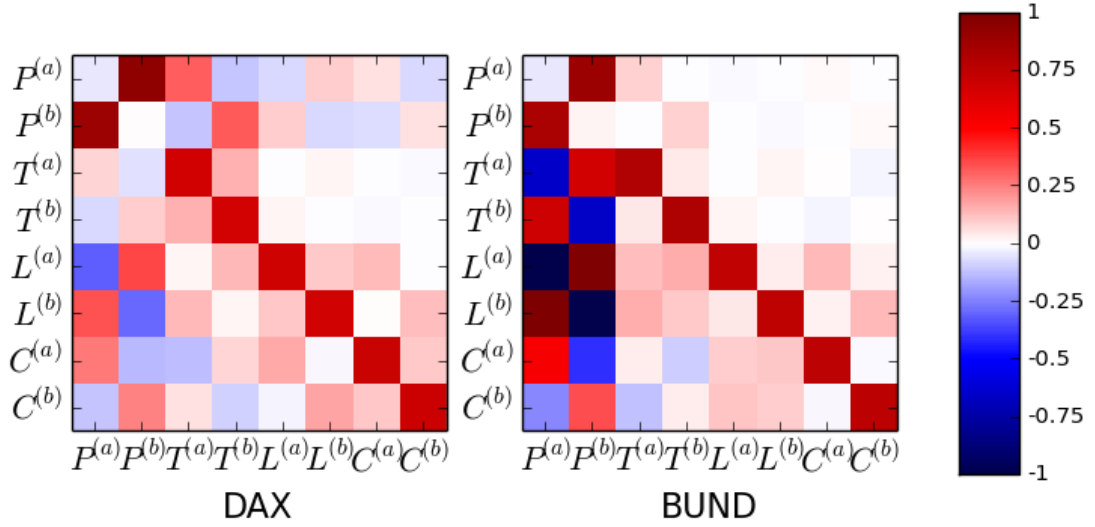
Figure V.4 – The matrix of estimated \|\phi^{ij}\| .
