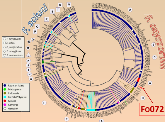
ML tree inferred from the EF1 \alpha gene sequence of Fusarium strains isolated from vanilla. F. oxysporum and F. solani are the most frequent species
