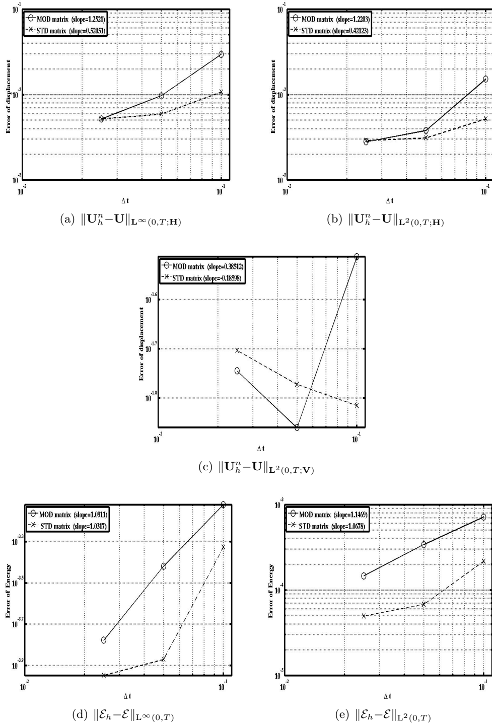
Figure 4.18: Comparison of the convergence curves obtained by the modified and standard mass matrices with square elements and \frac{\Delta x}{\Delta t} = 2 for 3D case by using the Newmark method II
