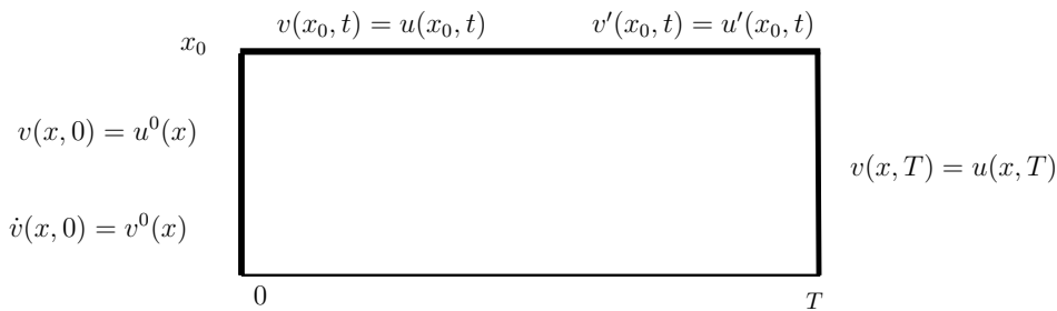
Figure 1.8: Initial and boundary conditions for v on the rectangle (0, x_0) \times (0, T) .
