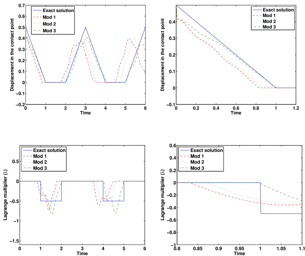
Figure 3.3: Comparison of the analytical solution (u, \lambda) and the approximate solutions (U_h^n, \lambda^n) by modified mass matrices in the contact node.
