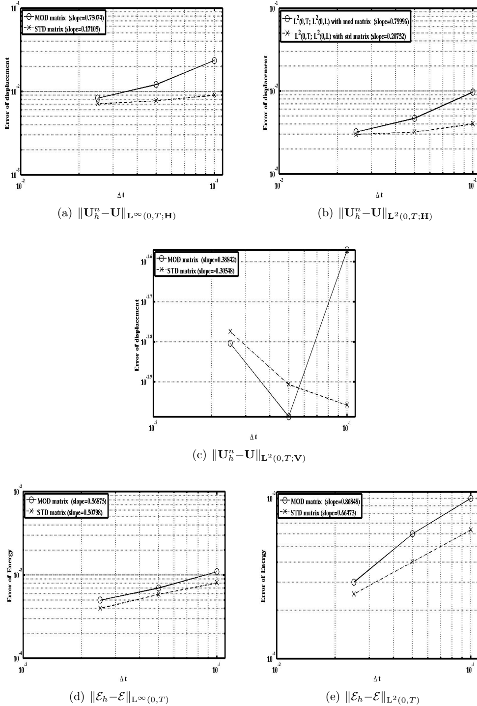
Figure 4.10: Comparison of the convergence curves obtained by the modified and standard mass matrices with square elements and \frac{\Delta x}{\Delta t} = 2 for 3D case by using the backward Euler method
