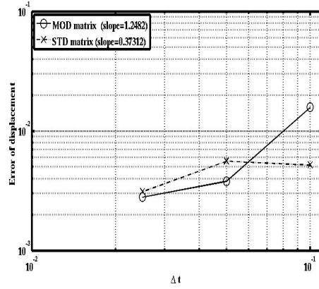
(b) \|\mathbf{U}_h^n - \mathbf{U}\|_{\mathbf{L}^2(0,T;\mathbf{H})}
