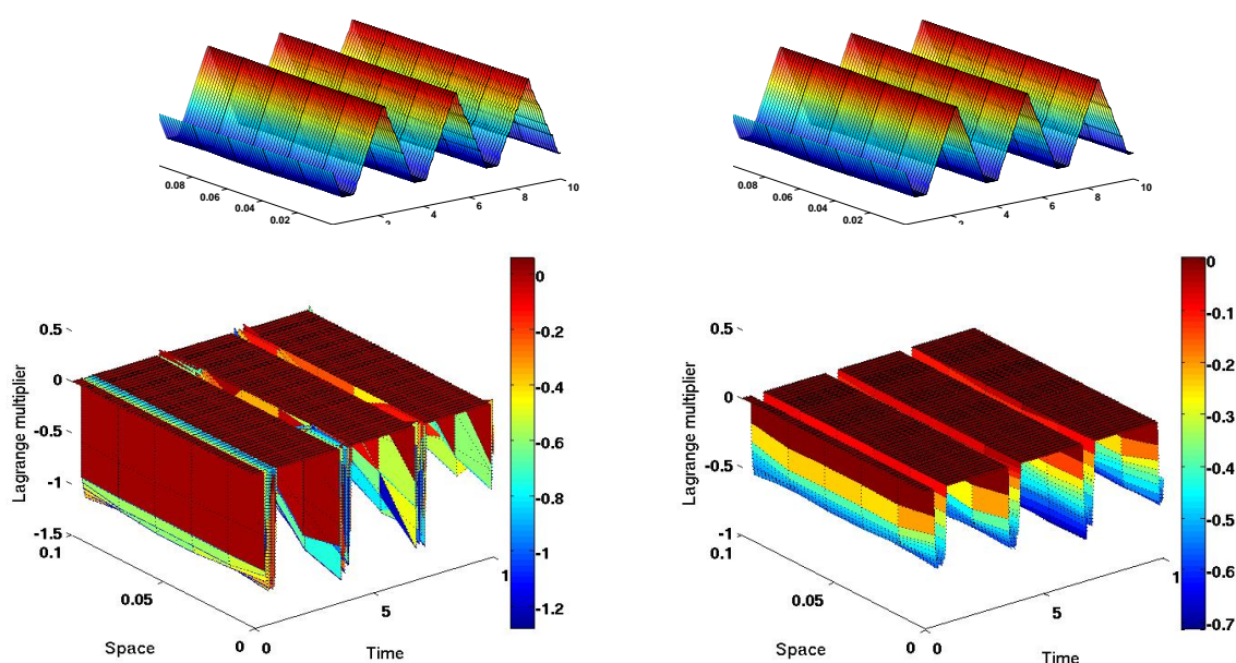
Figure 4.15: Approximated solutions obtained by using the standard (left) and modified (right) mass matrices in the contact node with the Newmark method II.
