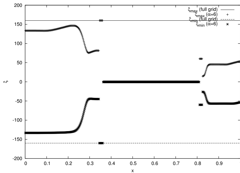
Figure IV.9: Test case 1, Kn_\infty = 10^{-5} : Maximum and minimum velocity in the local grids for \alpha = 6 (both criteria).
