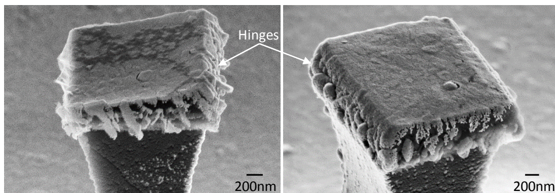
Figure 59: Soft/hard tweezers comprising a lower jaw in Co laminated with Ta after chemical etching of the sacrificial layer. Left: tweezer with a top jaw in NiFe laminated with Ta yielded good results. Right: tweezer with an upper jaw in CoFe (200 nm) were more prone to detach from their pillars.
