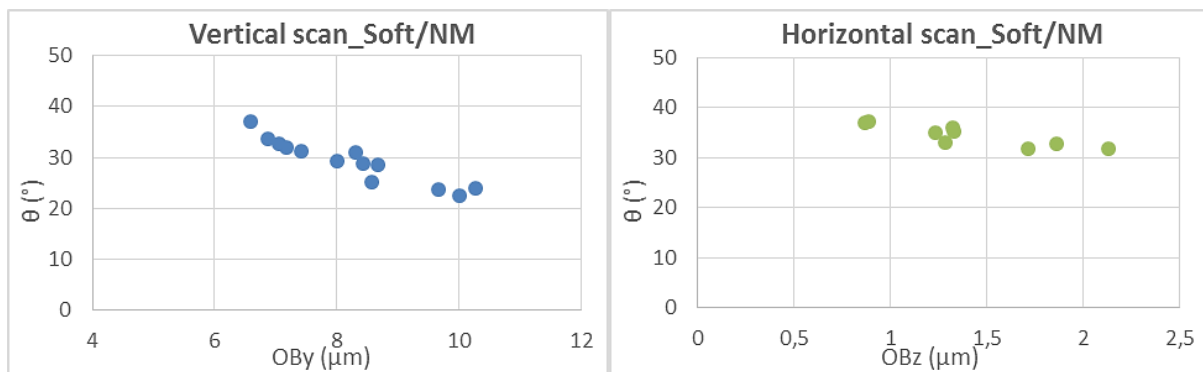
Figure 76: Relation between the angle \theta and the sphere center coordinates for the soft/non-magnetic tweezer. Left: the position of the sphere was moved along the y (vertical) direction at x = 1200 \text{ nm} and z = 1500 to 2000 \text{ nm} . Right: the position of the sphere varied along the z direction, laterally on the images, for x = 1200 \text{ nm} and y = 7500 to 7600 \text{ nm} . An offset of 13.8^\circ should be subtracted to the opening angle \theta to yield the angular displacement of the jaw.
