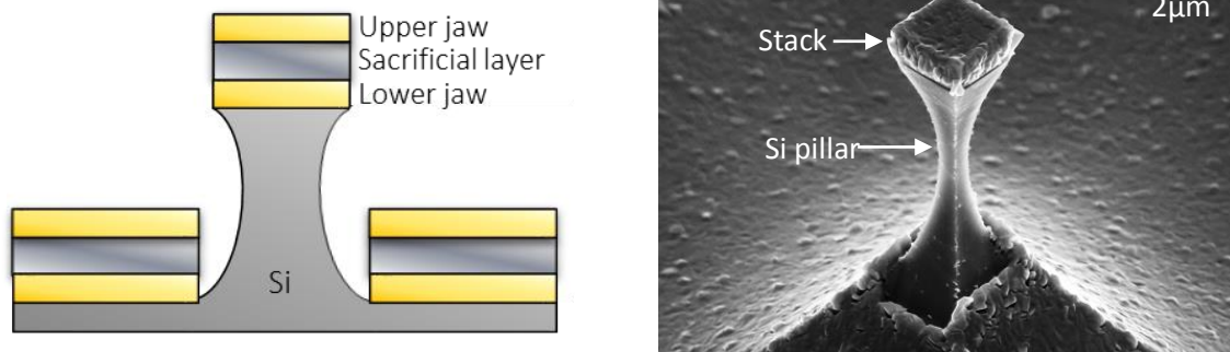
Figure 42: Example of stack with an upper jaw magnetically “soft” on top of a “hard” lower jaw, both separated by an Al sacrificial layer. The tweezers are located on top of the Si pillars.
