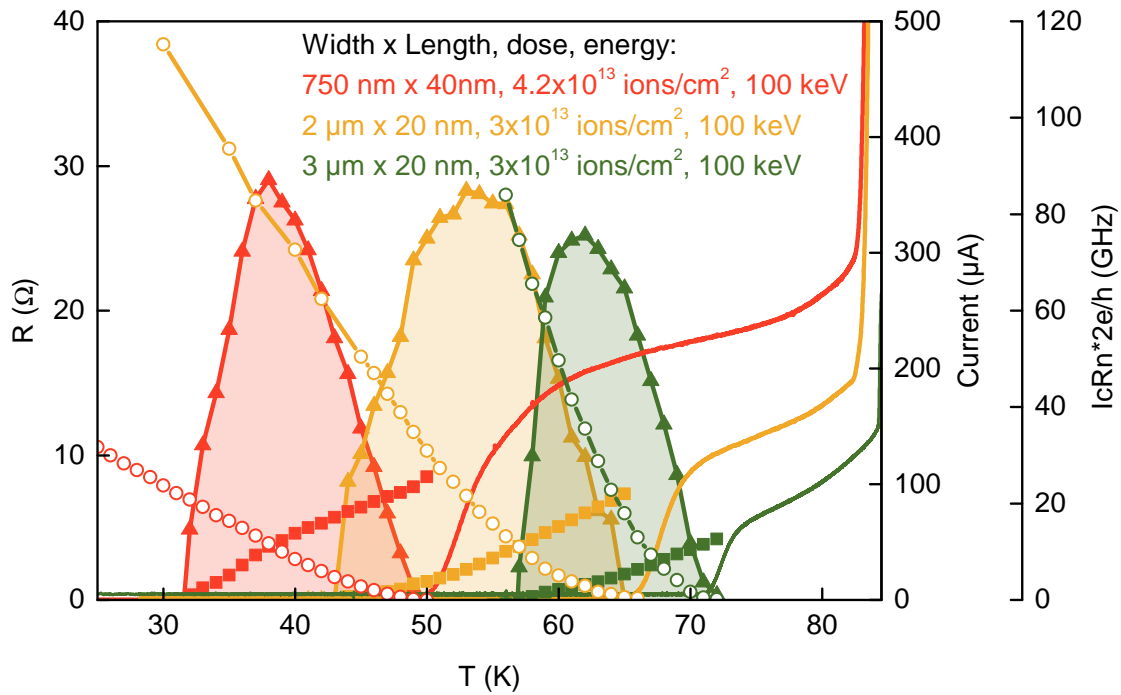
Figure 5.9: RT curves (plain lines), I_c(T) (circles), R_n(T) (squares) and f_c(T) (triangles) for three different junctions. The normal resistance has been calculated by derivation of the IV curves.
