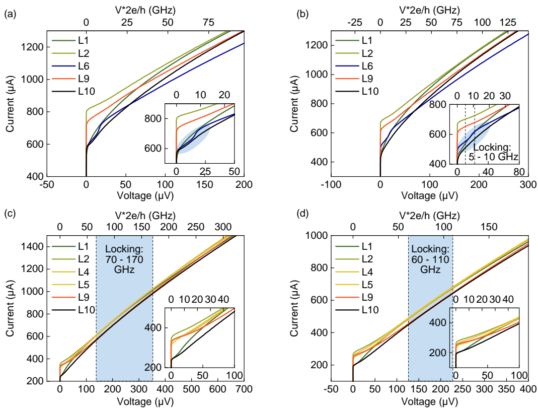
Figure 9.14: IV curves of several lines in the 10 \times 10 2D array, at 31 K (a), 33 K (b), 39 K (c) and 41 K (d). The locking phenomena are emphasized with the light blue shades. At 31 K and 33 K, L6 tends to phase lock with the previous lines, and at 39 K and 41 K, phase-locking happens in two separate groups of lines.
