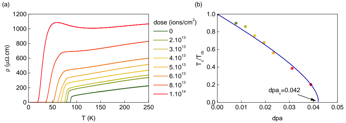
Figure 2.7: (a) Resistivity as a function of temperature of 70 nm thick \text{YBa}_2\text{Cu}_3\text{O}_7 films. The samples underwent an irradiation of \text{O}^+ ions at 110 keV and doses of (0, 2, 4, 5, 6, 8 and 10) \times 10^{13} ions.cm ^{-2} . (b) Evolution of T_c (normalized with T_{cb} ) as a function of the dpa. The plain line represents the fit with the Abrikosov-Gorkov depairing law with \text{dpa}_c = 0.042 .
