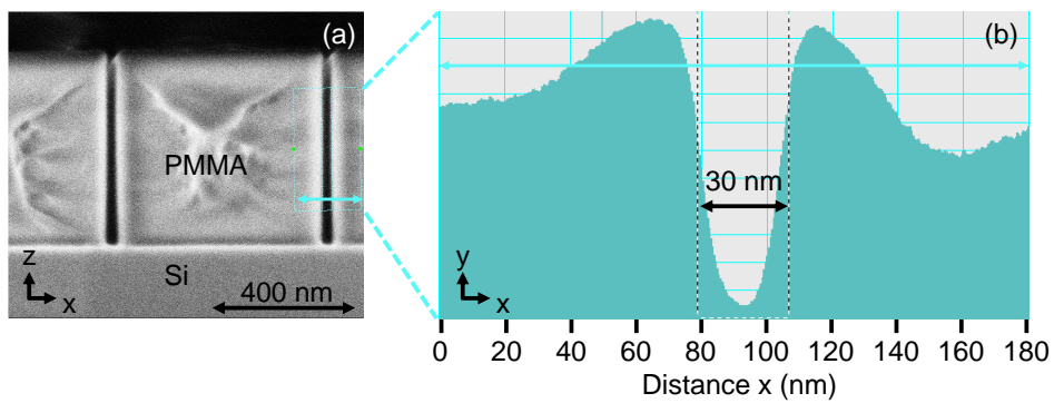
Figure 2.12: (a) SEM picture of two 30 nm slits taken in the (x, z) plane (same axes as in 2.4). The slit were e-beam lithographed and the sample was cleaved afterwards. (b) Histogram of the gray shades in the square rectangle around the right slit of (a). Courtesy of C. Ulysse and Thales Research and Technology.
