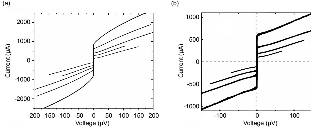
Figure 3.4: Typical IV curves of \text{YBa}_2\text{Cu}_3\text{O}_7 irradiated Josephson junctions, for various temperatures. (a) From top to bottom: T = 75.6, 76.9, 77.8, and 79.5 K [61]. (b) From top to bottom T = 40, 43.9, 46.3, and 48.5 K [36]. The IV curves in (b) correspond to the same junction whose RT curve is in figure 3.3 (b), with the 6 \times 10^{13} ions. \text{cm}^{-2} dose.
