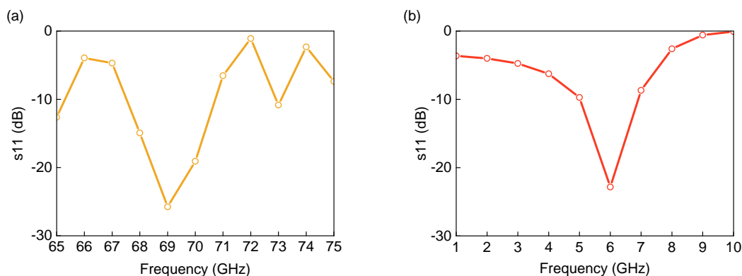
Figure 8.5: Reflection coefficients s_{11} of the 10\ \Omega lumped element as a function of frequency, around 70 GHz (a) and 6 GHz (b).
