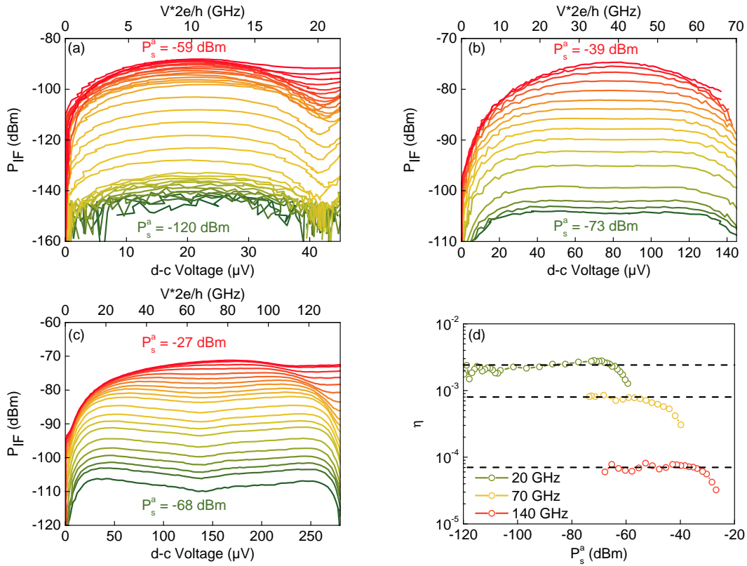
Figure 7.4: (a)-(c) Intermediate frequency power measured at T = 53 \text{ K} for three different LO frequencies, f_{LO} = 20 \text{ GHz} (a), f_{LO} = 70 \text{ GHz} (b) and f_{LO} = 140 \text{ GHz} (c). The signal power sent onto the antenna has been varied over several decades. (d) Conversion efficiency \eta = \frac{P_{IF}}{P_s^a} measured at V_{dc} * 2e/h = f_{LO}/2 , as a function of signal power. The horizontal black lines correspond to the ideal linear response of the mixer).
