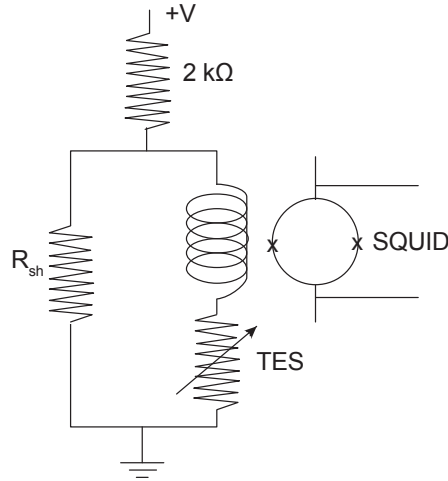
Figure 1.13: TES voltage bias circuit. The shunt impedance R_{sh} \sim 10 \text{ m}\Omega is much smaller than the TES impedance of about 1 \text{ }\Omega . Adapted from [205].
