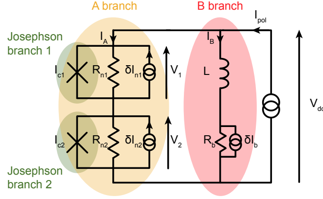
Figure 9.8: Two Josephson junctions in series (branch A), shunted by a LR circuit (branch B) that allows phase-locking.
