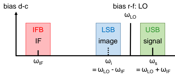
Figure 6.1: Spectral representation of the mixer operation. When biased in d-c and in r-f with a LO, it down-converts a signal at frequency \omega_s to an IF at \omega_{IF} . Upper-side band (USB) and lower-side band (LSB) are respectively the frequency bands above and below the LO frequency down-converted to the IF band (IFB). Their bandwidth is the same as the IFB. Then, the conversion phenomenon involves three frequencies: signal, IF, and image which is the symmetric of the signal with respect to \omega_{LO} . Here we arbitrarily chose to represent the signal at the USB.
