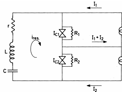
Figure 9.3: Two-junction cell coupled to a RLC resonant circuit [91].
