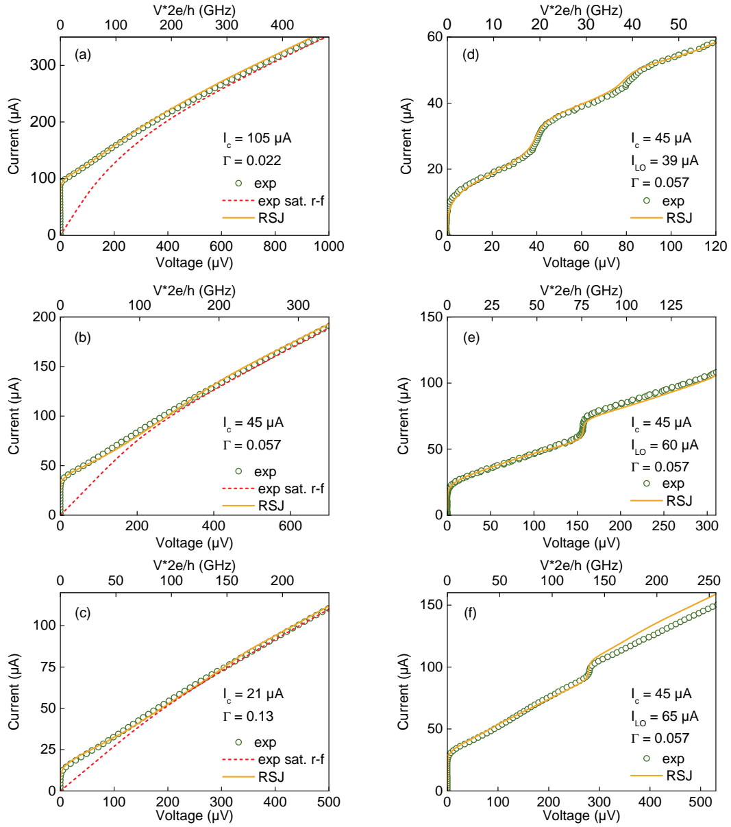
Figure 5.8: (a), (b), and (c) Current-voltage characteristics of the junction (open circles) measured at different temperatures 53 K, 58 K, and 62 K, respectively. Dashed lines correspond to the curve under strong microwave radiation and orange solid lines correspond to a fit using the RSJ model in which the non-linear resistance (i.e., dashed line) is introduced. The value of the fitting parameter I_c and the value of \Gamma = 2ek_bT/\hbar I_c used in the RSJ model are indicated on the graph. (d)–(f) Current voltage characteristics of the junction (open circles) measured at T = 58 K under LO radiation at 20 GHz, 70 GHz, and 140 GHz. Curves are fitted using the RSJ model (equation 5.12) including the non-linear resistance. The value of the fitting parameters I_c and I_{LO} and the value of \Gamma = 2ek_bT/\hbar I_c used in the RSJ model are indicated on the graph.
