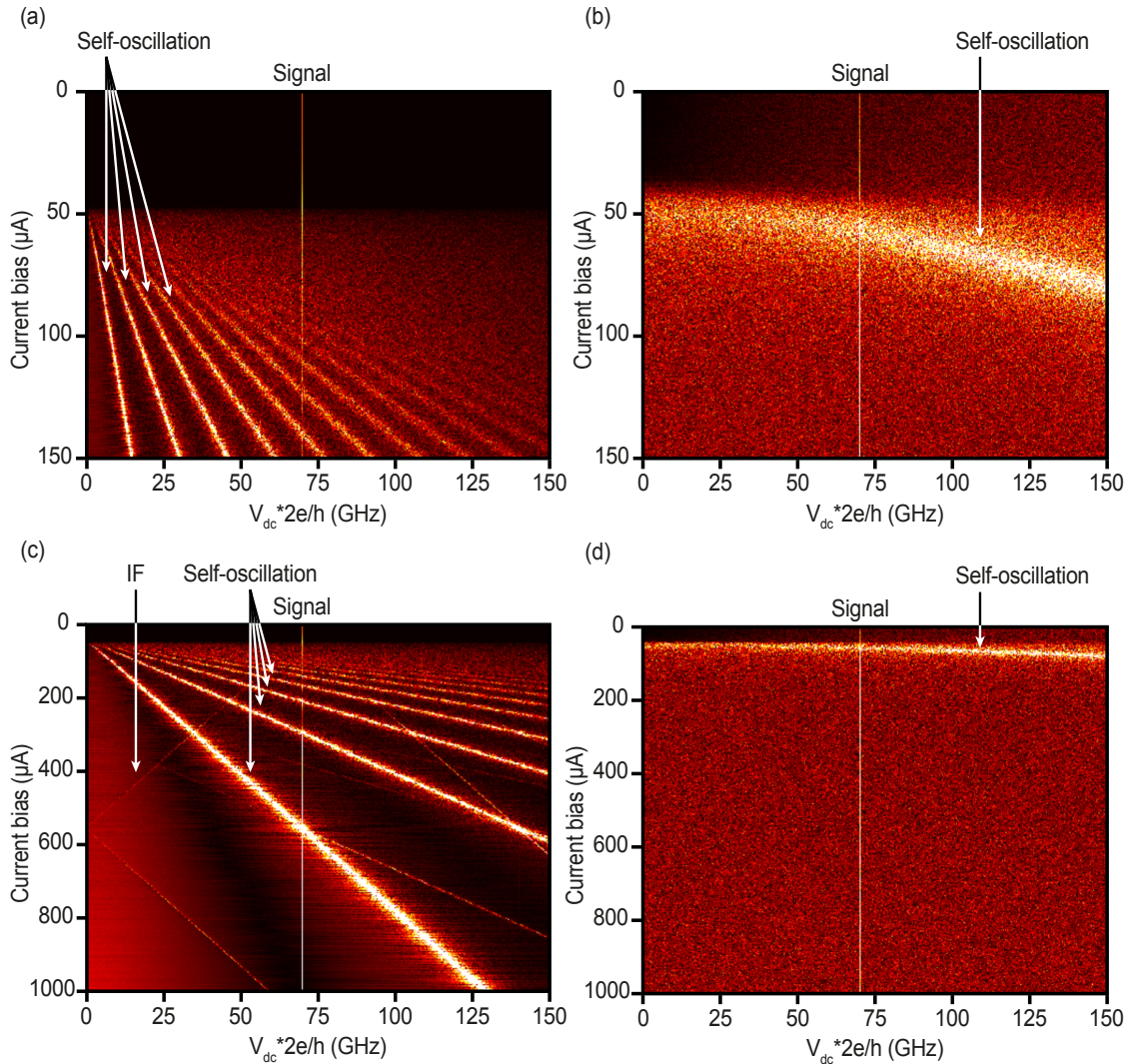
Figure 8.9: Simulated spectrum of the Josephson junction oscillation with (a,c) and without (b,d) an external LR shunting loop, as a function of the d-c current and voltage bias. The normal resistance is taken constant equal to 5 \Omega , and the critical current I_c = 50 \mu\text{A} . In the LR loop, L = 100 \text{ pH} and R_b = 0.5 \Omega .
