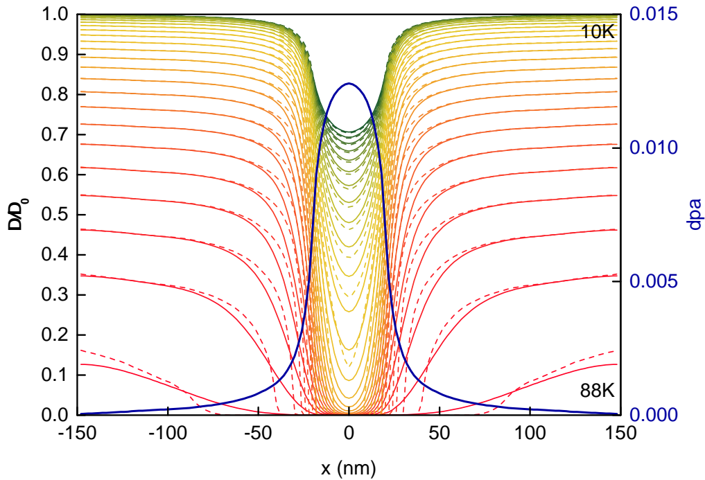
Figure 4.2: Normalized pair potential along the Josephson junction, every Kelvins from 10 to 88 K. The plain lines represent \Delta/\Delta_0 in the presence of proximity effects, and the dashed lines in their absence. The blue curve represents the dpa from which the pair breaking rate \Gamma(x) is calculated. It is a dpa obtained for an irradiation at 110 keV, a dose of 3.10^{13} ions.cm -2 , for a 40 nm long and 70 nm thick junction.
