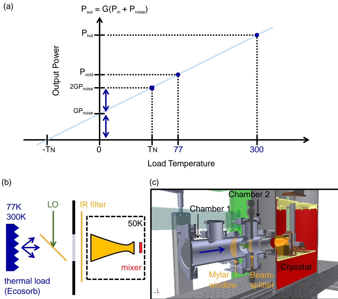
Figure 8.7: (a) Definition of the noise temperature T_N and Y factor. (b) Principle of the experiment. An thermal load radiates as a blackbody, with a power depending on its temperature. The mixing with LO enables to calibrate the detector. (c) Design of the experimental setup: two separated chambers allow to send a weak hot or cold load signal onto the mixer.
