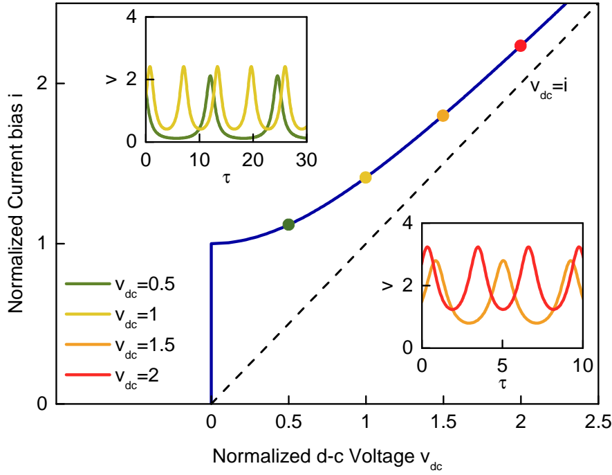
Figure 3.9: Simulation of a IV curve with no capacitance (pure RSJ model), and corresponding voltage temporal oscillations in normalized units, at different values of d-c voltage \langle v \rangle = v_{dc} . The oscillation period is given by 3.35. As the current bias increases, the oscillations have a sinus shape, and the average of the a-c Josephson effect is null, only leaving the d-c component: v_{dc} = i .
