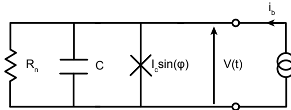
Figure 3.6: Equivalent circuit of an ideal weak-link Josephson junction: resistively and capacitively shunted junction (RCSJ) model.
