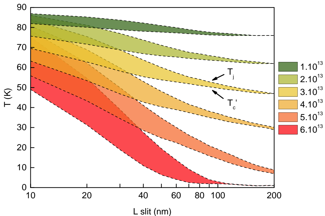
Figure 4.4: Josephson regime (colored areas) as a function of the length of the slit and for various irradiation doses. Each region spans between T'_c and T_j . The irradiation energy is 110 keV.
