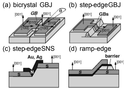
Figure 2.1: Categories of high- T_c Josephson junctions, taken from [113].
