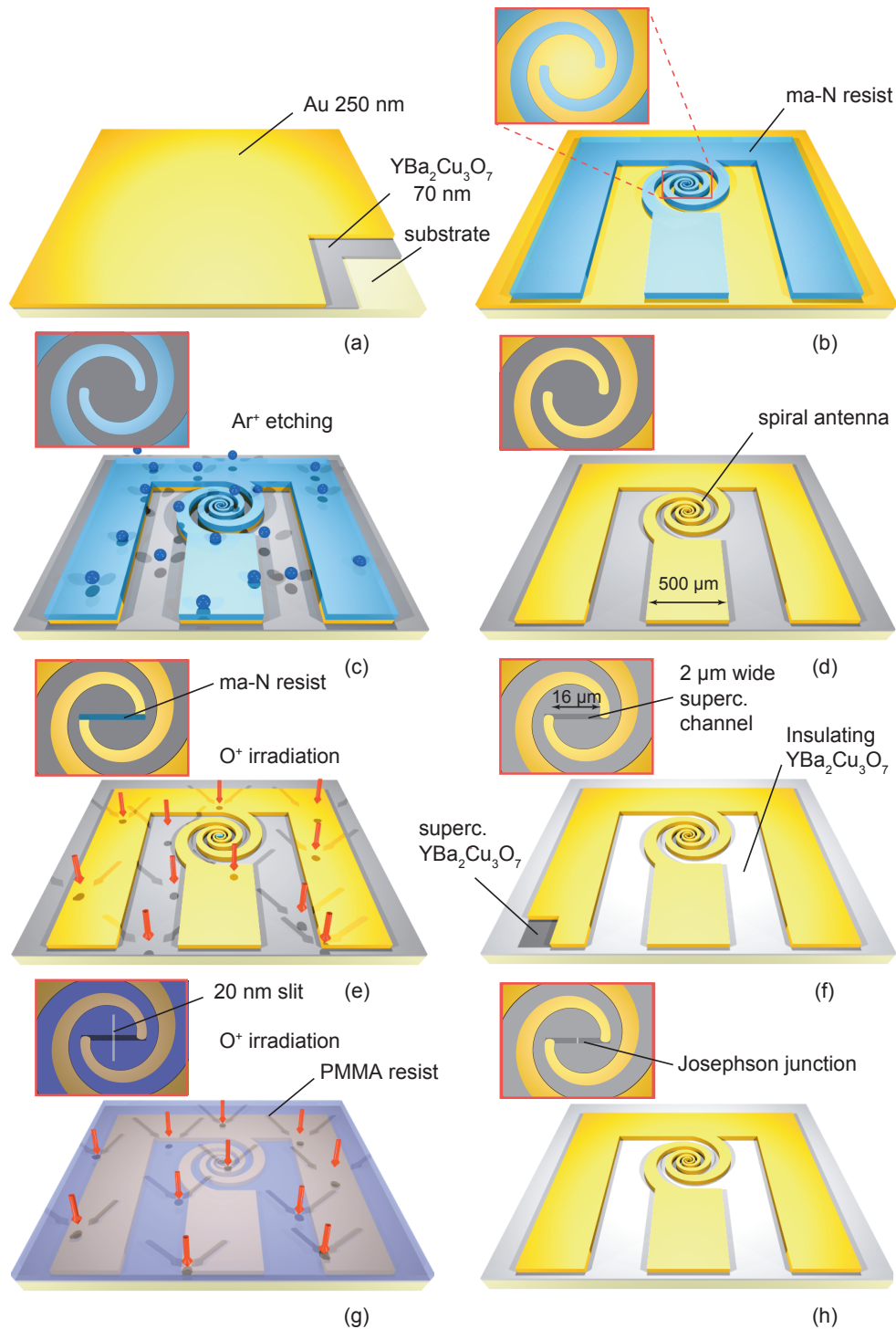
Figure 2.8: Illustration of the fabrication process steps: (a) 70 nm thick \text{YBa}_2\text{Cu}_3\text{O}_7 film grown on sapphire covered by an in situ 250 nm gold layer; (b) spiral antenna in the CPW transmission line defined in a 500 nm thick MAN-2405 negative e-beam resist; (c) 500 eV Ar ion-beam-etching of the gold layer; (d) gold antenna in the CPW transmission line on \text{YBa}_2\text{Cu}_3\text{O}_7 ; (e) high-dose 70 keV oxygen ion irradiation to create insulating regions in exposed \text{YBa}_2\text{Cu}_3\text{O}_7 . A 2 \mu\text{m} wide channel in the center of the antenna is protected by a 500 nm thick MAN-2405 resist mask; (f) patterned superconducting and insulating \text{YBa}_2\text{Cu}_3\text{O}_7 regions; (g) low-dose 110 keV oxygen ion irradiation of the Josephson junction patterned as a 20 nm-wide slit in a 500 nm thick PMMA resist; and (h) device after resist cleaning. From [135].
