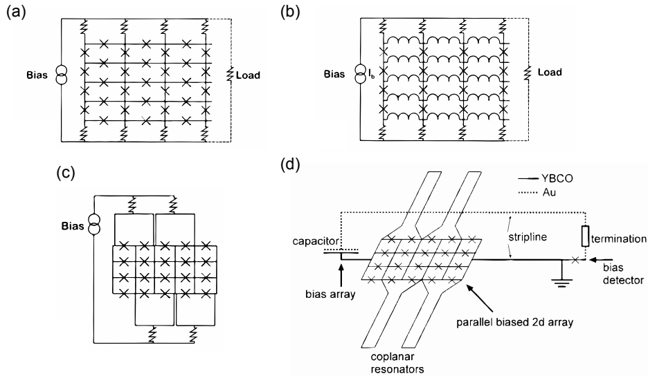
Figure 9.7: Different architectures for 2D arrays: (a) X-Y, (b) 2D shorted and (c)-(d) parallel biased. In (d), junctions are placed in resonators, favoring synchronization [64, 38].
