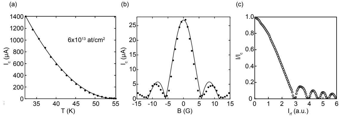
Figure 3.5: (a) Variation of the critical current with temperature, following a quadratic law, and (b) Modulation of the critical current with an external magnetic field, following a sinc function. Adapted from [36]. (c) Modulation of the critical current with an external r-f field, following a Bessel function. Adapted from [136].
