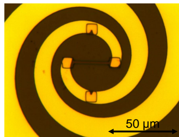
Figure 2.10: Optical photo of a MAN-2405 micro bridge (750 nm wide, 15 \mu\text{m} long) at the center of a spiral antenna.
