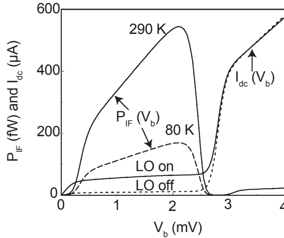
Figure 1.14: Simulations of IV curves and IF response of a niobium SIS mixer. Adapted from [205].
