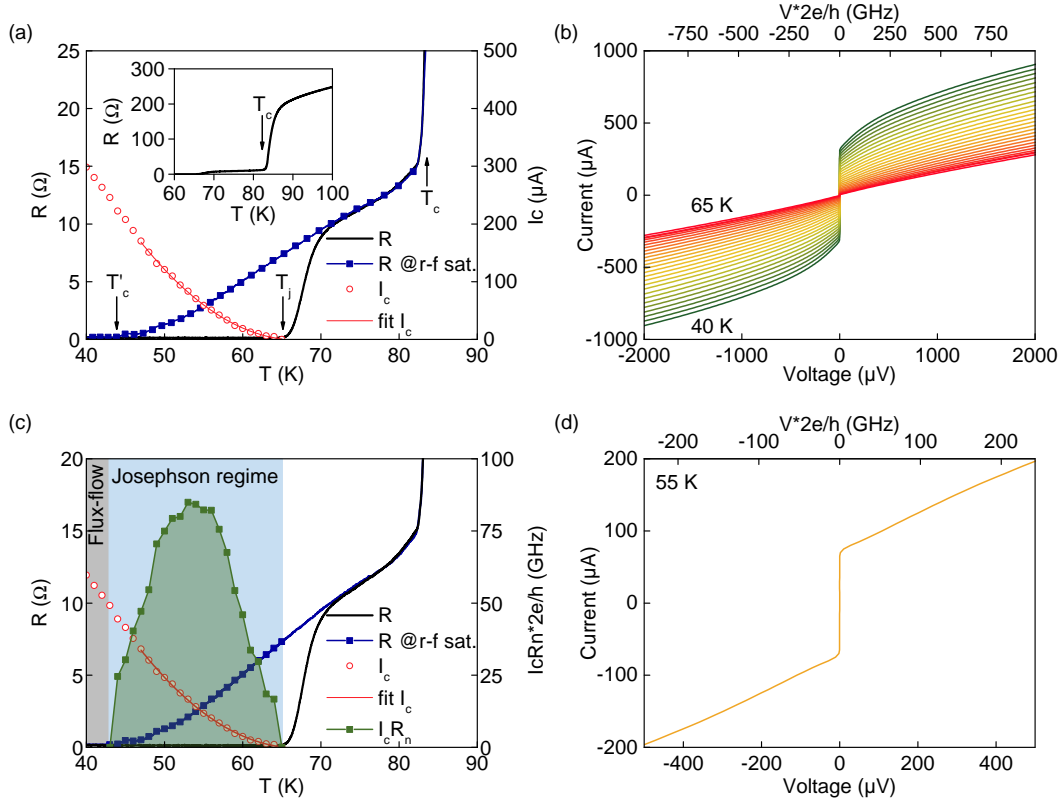
Figure 5.3: d-c and a-c characterization of the junction. (a) Resistance R and critical current I_c , as a function of temperature. The normal resistance R_n , blue curve, is obtained from the RT curve recorded when the junction is saturated with microwaves. Three temperatures T_c , T_j , and T_c' are indicated on the graph. Inset: RT curve at larger scale. (b) IV curves at each K , between 40 and 65 K. (c) I_c R_n product in frequency unit superimposed to the previous curves. (d) IV curve at T = 55 K, i.e. in the Josephson regime.
