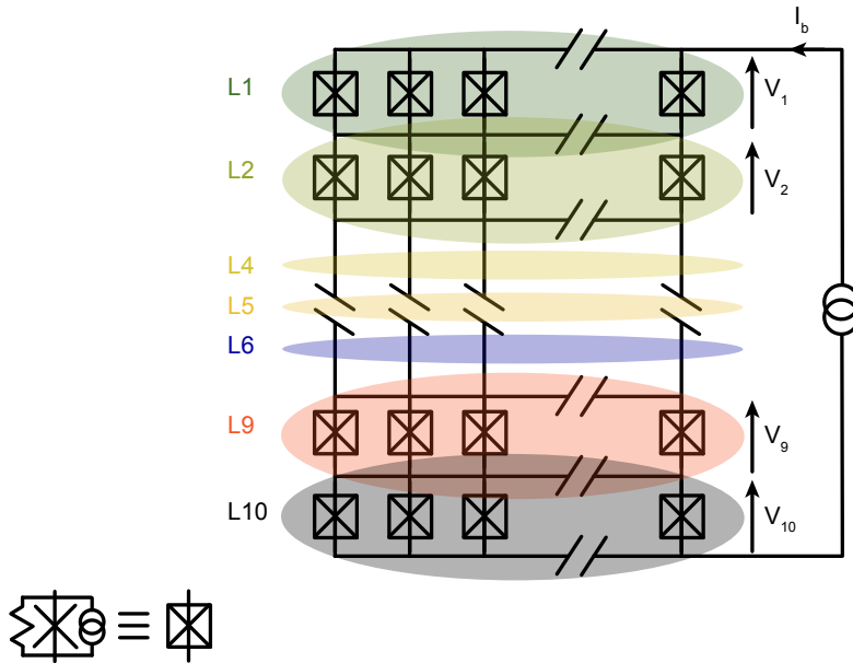
Figure 9.13: Circuit of the 10 \times 10 2D array. When current biased top to bottom, the voltages across each line can be read independently.
