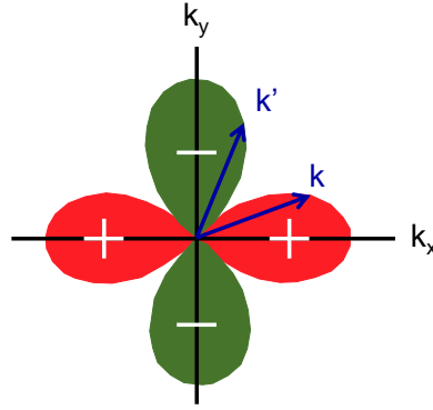
Figure 2.6: The d-wave symmetry of the superconducting wave function in YBa 2 Cu 3 O 7 . A scattering event can induce a phase jump from \mathbf{k} to \mathbf{k}' , which breaks the Cooper pair.
