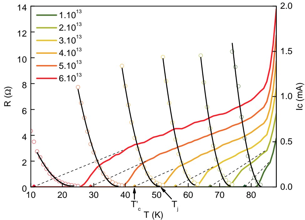
Figure 4.3: Color lines: Simulated normal resistance as a function of the temperature, for various irradiation doses. We take \Delta < 0.1k_bT as the criterion for a resistive region inside the junction. Then we calculate the resistance with equations 2.7 and 2.8 of chapter 2. Circles points: critical current I_c as a function of temperature. Black lines: square fits of I_c(T) .
