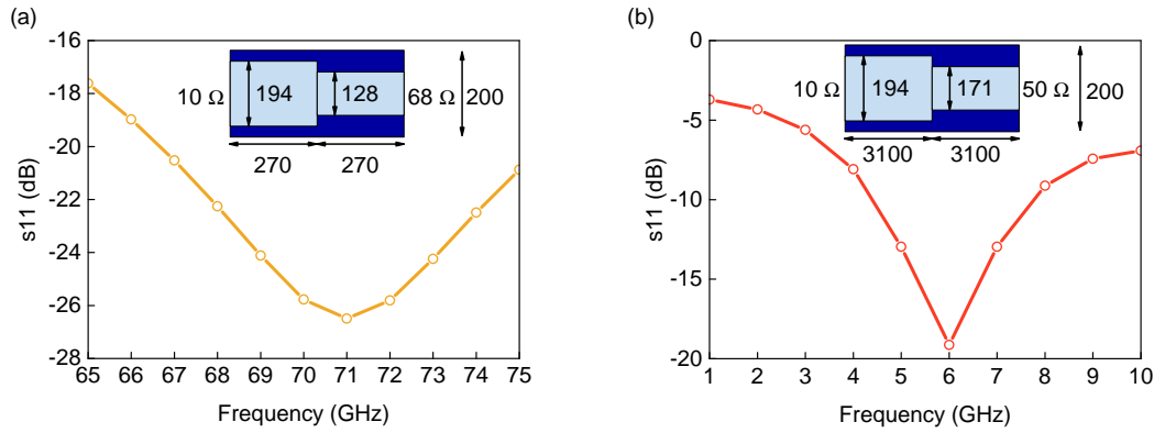
Figure 8.3: Reflection coefficients s_{11} of the 10 \Omega lumped element, as a function of frequency when connected to the Chebyshev filters whose characteristics are summarized on the sketches. The dimensions are in \mu\text{m} .
