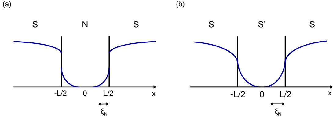
Figure 4.1: Schematic of the pair condensation amplitude in a SNS (a) and in a SS'S (b) junction. The different materials in contact at the interfaces of the SNS junction induces a discontinuity, and the amplitude decreases exponentially over a shorter length \xi_N than in the SS'S case, where there is no discontinuity.
