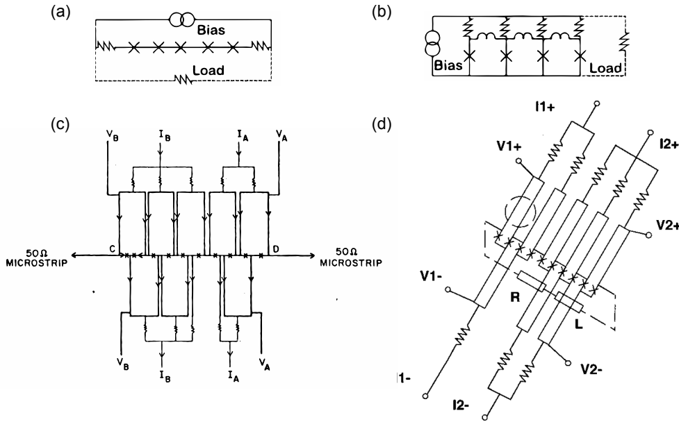
Figure 9.5: Different architectures for 1D arrays: (a) 1D series, (b) 1D parallel and (c)-(d) d-c-parallel/a-c-series array. In (d), junctions are placed in half-wavelength resonators, favoring synchronization [64, 119, 99].
