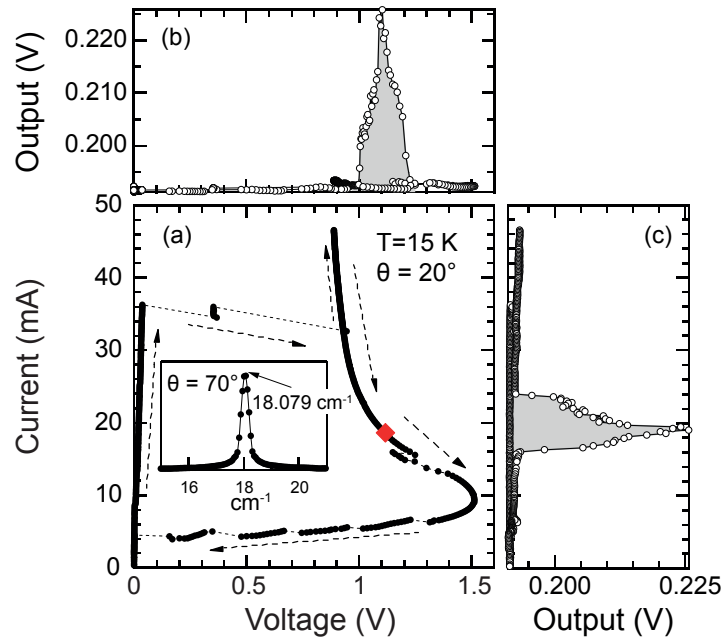
Figure 1.8: IV curve (a) and detected emission with a Si-composite bolometer (b),(c). The inset of figure (a) is the spectrum obtained by Fourier-transform infrared spectroscopy, at the bias point indicated by a red square. \theta is the angle between the c -axis of the Bi2212 crystal and the Si bolometer. Adapted from [103].
