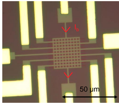
Figure 9.12: Photograph of the 10x10 2D shorted array.
