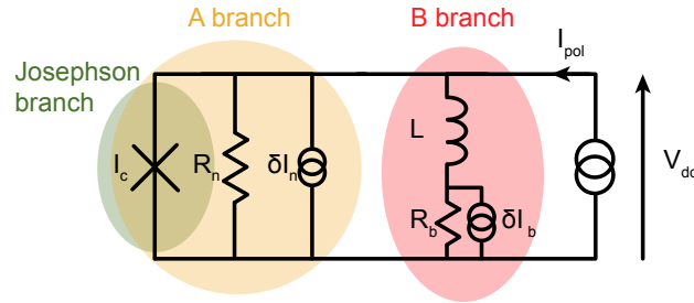
Figure 8.8: RSJ model of a Josephson junction, externally shunted by an inductive ( L ) and resistive R_b loop in parallel.
