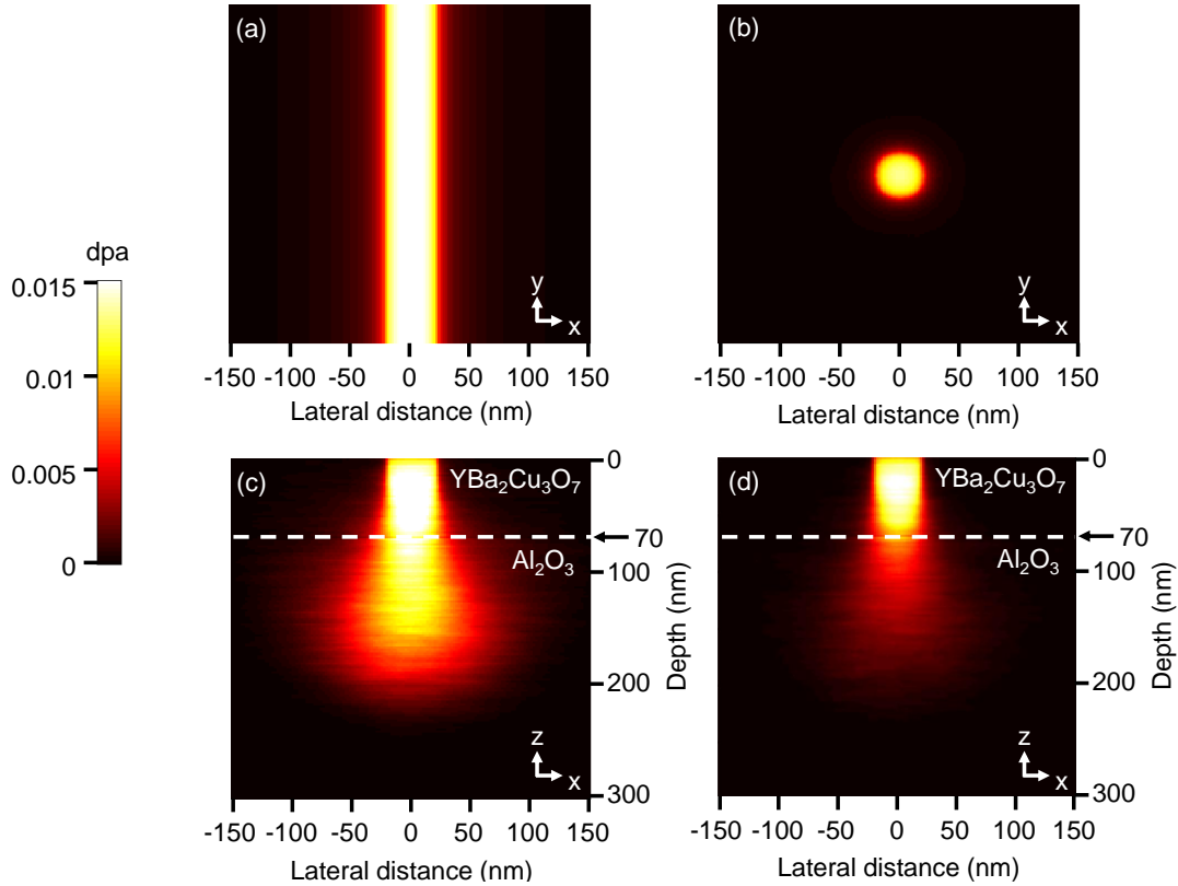
Figure 2.4: Simulated dpa for implanted ions at 110 keV and 5.10^{13} ions. \text{cm}^{-2} . (a) \text{dpa}(x,y,z < 70 \text{ nm}) in the (x,y) plane for a 40 nm slit and (b) for a 40 nm hole in diameter. (c) simulated \text{dpa}(x, |y| < 2 \text{ nm}, z) in the (x,z) plane of the slit, and (d) for the hole.
