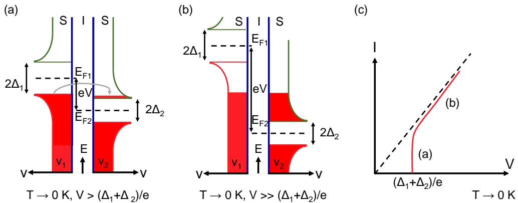
Figure 3.1: (a) and (b): semi-conductor model of the quasiparticle tunneling effect in a SIS junction. The DOS \nu_1 and \nu_2 of each superconducting reservoir is given by the BCS theory (equations 3.2). (c): corresponding quasiparticle branch in the IV characteristics. The vertical part of the branch corresponds to situation (a), and the linear part corresponds to situation (b).
