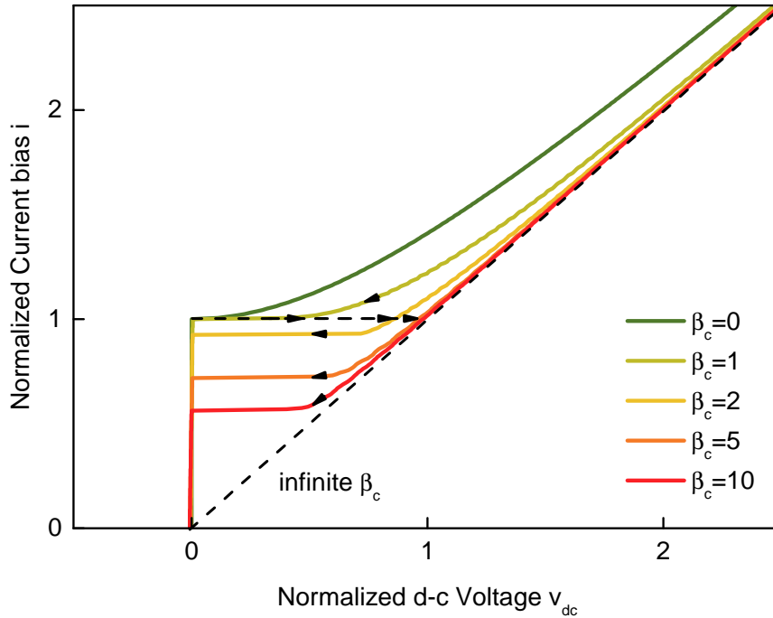
Figure 3.8: Simulations of IV curves in the RCSJ model, for various values of the McCumber parameter. For \beta_c = 0 the curve is not hysteretic: the path is the same when i increases or decreases. For \beta_c > 1 , the curves are hysteretic and when i increases, a switching occurs from i = 1 (at the critical current) to a position indicated by dashed arrows. When i decreases the path is indicated by arrows on the curves. Adapted from [163].
