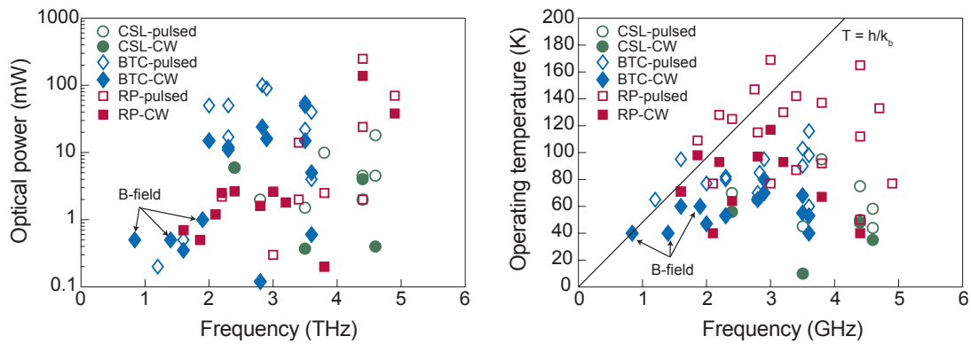
Figure 1.9: Reported peak performances of QCL (a) and maximum operating temperatures (b). Various structures are compared: chirped superlattices (CSL), bound to continuum (BTC), and resonant phonon (RP). Adapted from [197].
