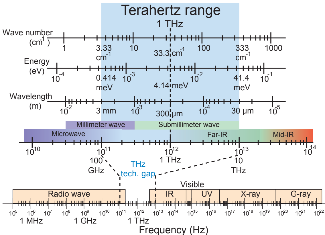
Figure 1.1: Terahertz band in the electromagnetic spectrum. Adapted from [124].
