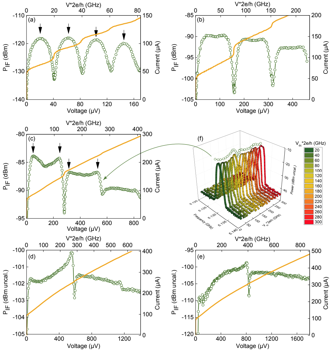
Figure 7.3: (a)–(e) Output power at the IF (left scale) and d-c current (right scale) as a function of voltage measured at T = 53 K for five different LO frequencies, f_{LO} = 20 GHz (a), f_{LO} = 70 GHz (b), f_{LO} = 140 GHz (c), f_{LO} = 280 GHz (d), f_{LO} = 410 GHz (e). The IF frequency is about 6 GHz. For the three lowest frequencies (panels (a)–(c)), the power of the signal has been set to approximately one thousandth of the LO power. For the two highest frequencies (d) and (e), the signal power is of the same order as that for the LO. (f) Recorded spectrum showing the IF peak, whose power varies with d-c voltage V_{dc} . The LO and signal excitations are set around 140 GHz, producing an IF beating at f_{IF} = 5.13 GHz. The power decreases at V_{dc} \frac{2e}{h} = 140 GHz, corresponding to the first Shapiro step on the IV curve of (c).
