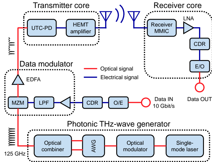
Figure 1.4: Block diagram of the 120-GHz-band wireless link system. Adapted from [93, 146].
