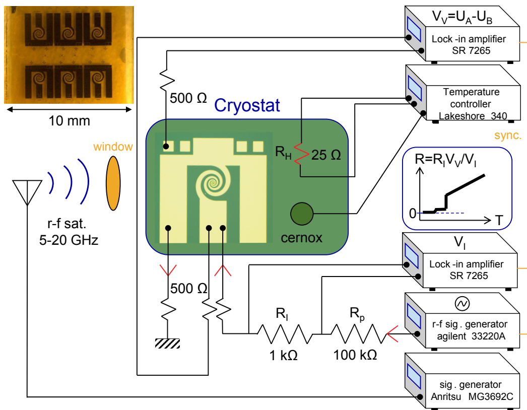
Figure 5.1: Schematic of the a-c measurement setup of the RT curves. Inset: photograph of a fabricated electronic chip, on which there are six mixers.
