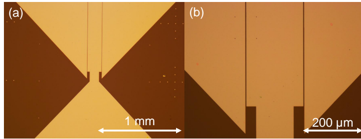
Figure 8.6: (a) Photo of the optimized design. (b), Photo, showing the detail of the Chebysev adaptation.
