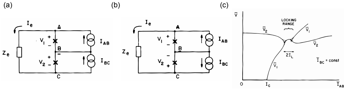
Figure 9.2: Two-junction cell, biased in series (a), and in parallel (b). (c) Evidence of synchronization on the IV curves. Adapted from [100].
