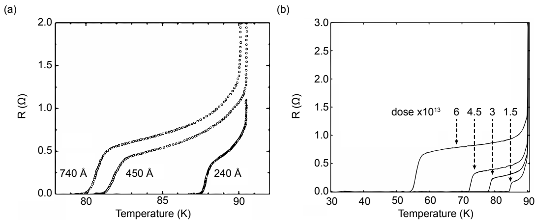
Figure 3.3: RT curves of ion irradiated \text{YBa}_2\text{Cu}_3\text{O}_7 Josephson junctions. (a) Junctions with various lengths, irradiated at the same dose (and with \text{Ne}^+ at 200 \text{ keV} ) [105]. (b) Junctions of the same length ( 20 \text{ nm} ), irradiated from right to left at doses 1.5 \times 10^{13} , 3 \times 10^{13} , 4.5 \times 10^{13} , and 6 \times 10^{13} \text{ ions.cm}^{-2} (oxygen ions, at 100 \text{ keV} ) [36].
