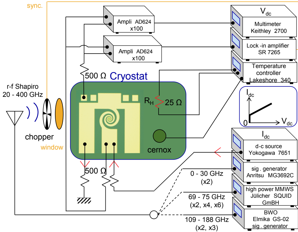
Figure 5.2: Schematic of the d-c measurement setup of the IV curves.
