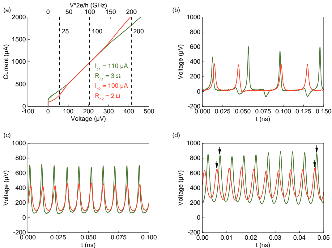
Figure 9.10: (a) Simulated IV curves of two junctions in series, shunted by the LR branch, as in figure 9.8. (b), (c) and (d) voltage as a function of time for both junctions, at 25, 100 and 200 GHz respectively. I_{c1} = 110 \mu\text{A} , R_{n1} = 3 \Omega , I_{c2} = 100 \mu\text{A} and R_{n2} = 2 \Omega . The simulation temperature is T = 50 \text{ K} , L = 20 \text{ pH} and R_b = 0.5 \Omega .
