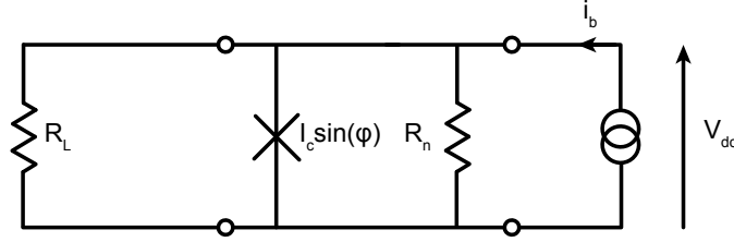
Figure 9.1: A current biased RSJ coupled to a load R_L .
