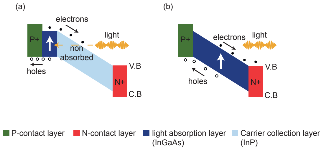
Figure 1.7: Band diagram of a UTC-PD (a) and a PIN PD (b). Adapted from [146].
