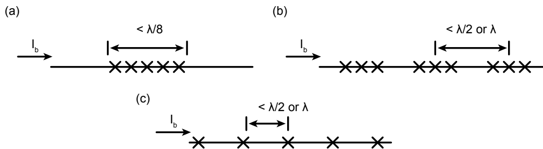
Figure 9.4: Different categories of arrays, depending on the space between the junctions. (a) Lumped, (b) quasilumped and (c) distributed arrays. \lambda is the radiation's effective wavelength, see equation 9.9. Adapted from [90].
