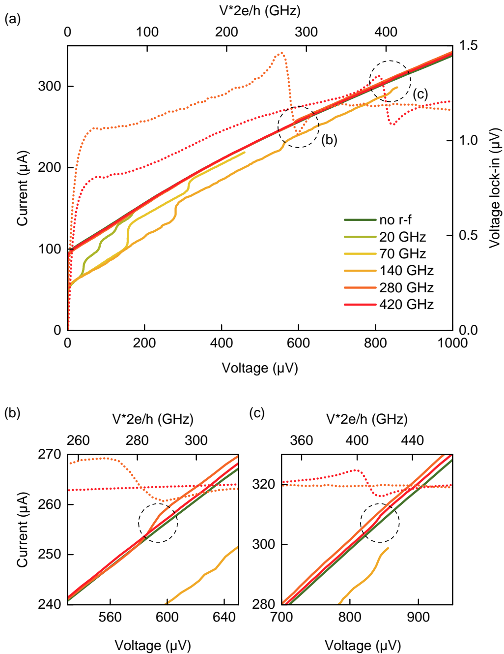
Figure 5.4: Evidence of Shapiro steps on the IV curves of the Josephson junction, at T = 53 K. (a), plain lines: IV curves of the Josephson junction under high frequency illumination. Shapiro steps appear at harmonics of the r-f frequency excitation. Dotted lines: lock-in response when the incoming r-f field at 280 and 420 GHz is chopped, showing important variations at the steps positions. (b) and (c), zoom on the IV curves around 280 and 420 GHz respectively.
