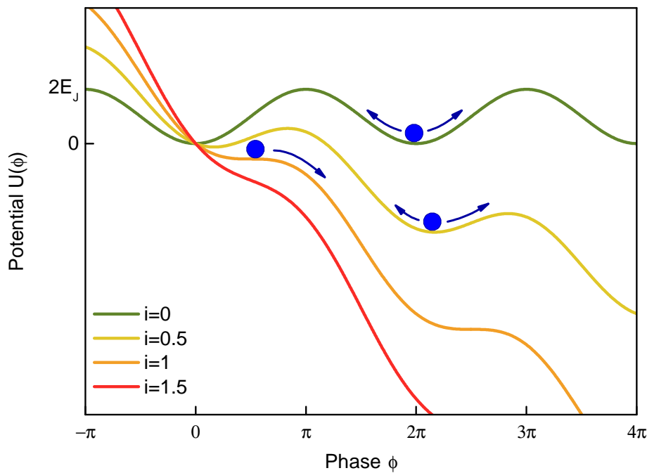
Figure 3.7: Analog system to the RCSJ model: a particle of mass \beta_c moves along a washboard potential. The current i tilts the overall slope, and motions the particle at a velocity \dot{\phi} = v , where v is the voltage across the junction. When i > 1 , the particle moves freely on the washboard and \langle v \rangle \equiv v_{dc} \neq 0 . Adapted from [163].
