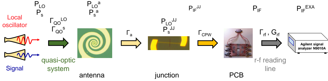
Figure 7.2: Representation of power losses ( \Gamma_{QO}^{LO} , \Gamma_{QO}^S , \Gamma_a , \Gamma_{CPW} , \Gamma_{rf} ) and gain ( G_{rf} ) in the heterodyne mixing setup.
