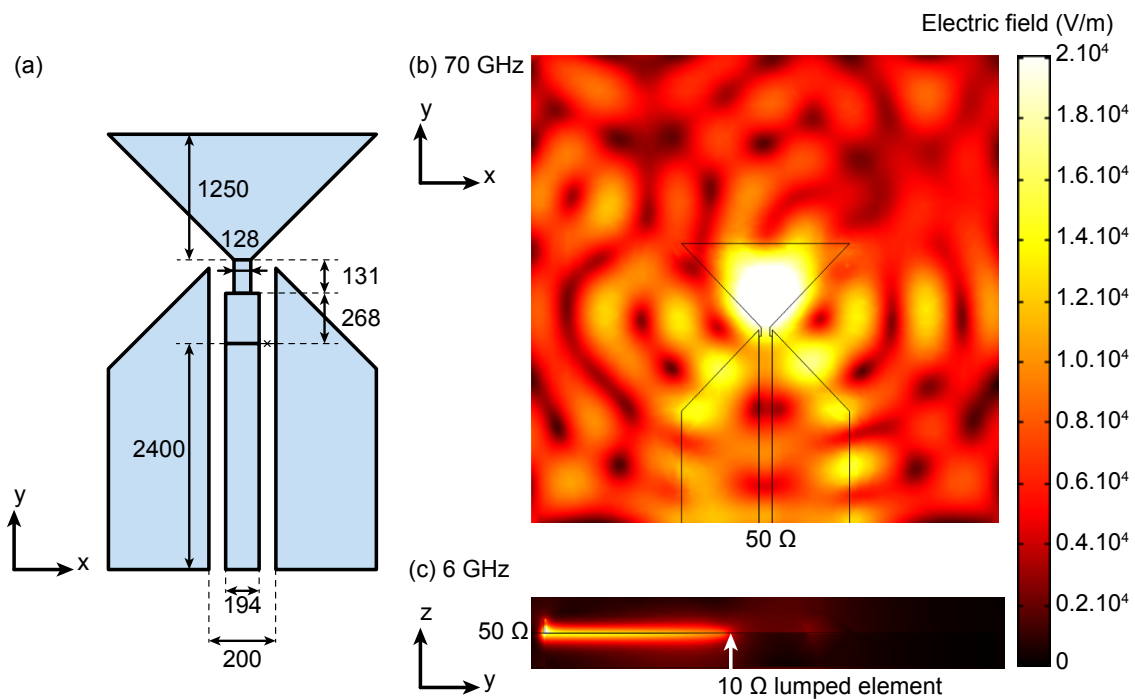
Figure 8.4: (a) Characteristic dimensions in \mu\text{m} of the optimized design (not to scale). (b) and (c) Electric field amplitude when the structure is excited at 1\ \text{V/m} by the 10\ \Omega lumped element at the Josephson junction's place (indicated by a cross in (a)) at 70 GHz (b) and 6 GHz (c).
