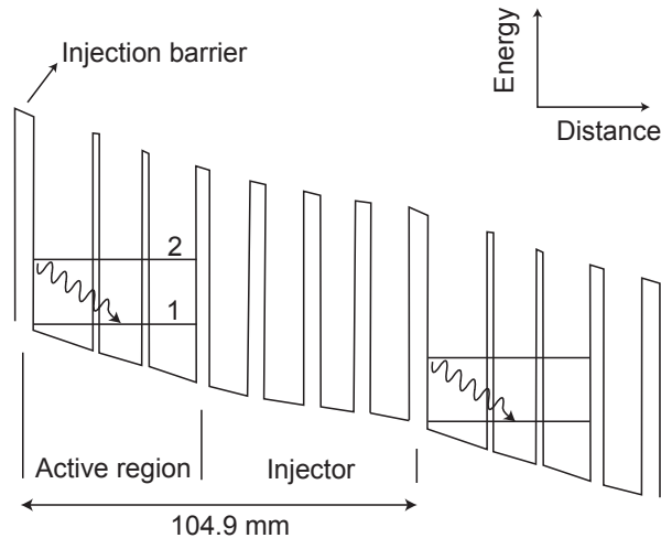
Figure 1.10: Simplified conduction band of a QCL. Electrons are injected through the AlGaAs injection barrier into the upper lasing level of the active region (GaAs). Transition to the lower lasing level results in the emission of a THz photon. Due to the applied electric field, the band diagram is tilted and electrons escape to the subsequent injector band. Adapted from [75, 77].
