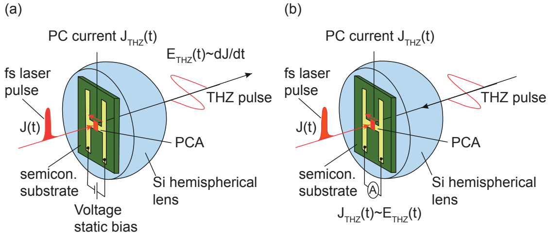
Figure 1.5: THz pulse emission (a) and detection (b) with a photoconductive antenna. Adapted from [173].
