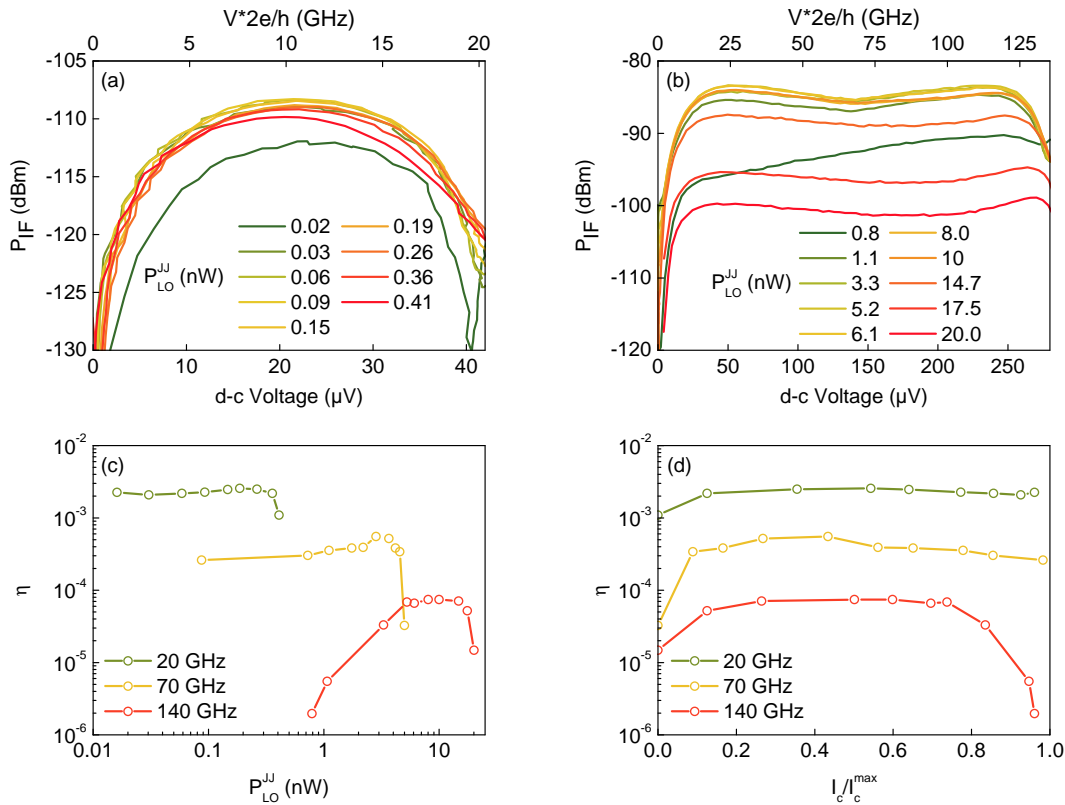
Figure 7.5: (a) and (b) Power in dBm at IF measured at T = 53 K for different values of the LO power received by the junction. The LO frequency is 20 GHz on panel (a) and 140 GHz on panel (b). (c) Conversion efficiency taken at V_{dc} * 2e/h = f_{LO}/2 as a function of LO power coupled to the junction. (d) Conversion efficiency taken at V_{dc} * 2e/h = f_{LO}/2 as a function of critical current reduction for the three LO frequencies.
