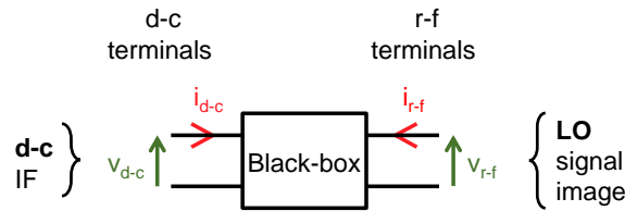
Figure 6.2: The mixer considered in circuit theory as a black-box with four ports: two for the d-c current and voltage, and two for the r-f current and voltage. As the LO is much stronger than any other power at r-f frequencies, one can consider that i_{rf} = i_{LO} , and v_{rf} = v_{LO} .
