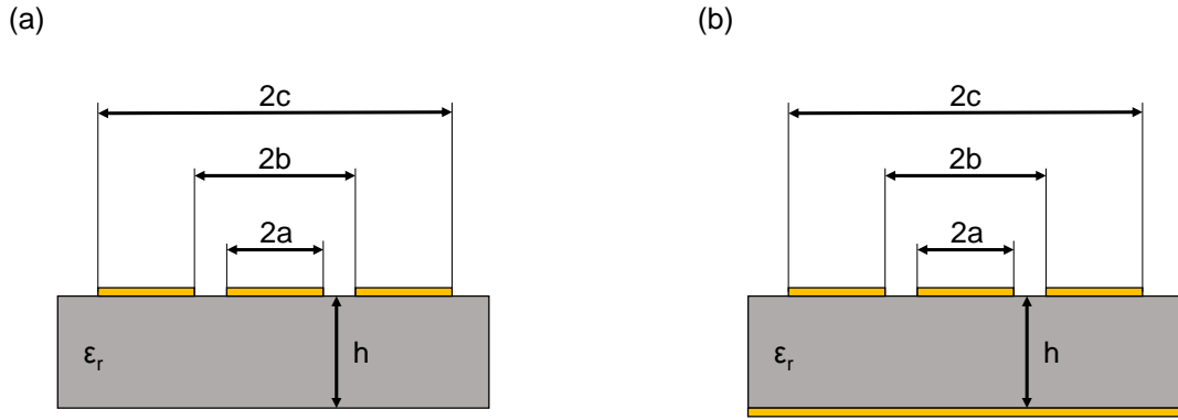
Figure E.1: (a) coplanar waveguide and (b) conductor-backed coplanar waveguide.
