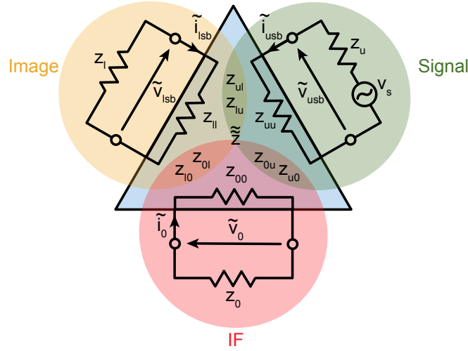
Figure 6.3: Schematic vision of the mixer (blue triangle) connected to the external circuitry, once d-c and LO biased. The signal is taken at the USB. Depending on the frequency, different load impedances are presented at the mixer terminals: z_u , z_0 and z_l respectively at the USB, IFB and LSB. The diagonal terms of the impedance matrix 6.14 can be viewed as impedances directly connected to the external ones, whereas the off-diagonal ones enable energy transfers between the three frequency bands.
