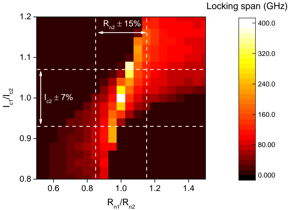
Figure 9.11: Locking span at 50 K, in color scale, when I_{c1} and R_{n1} vary. The parameters of the second junction are fixed: I_{c2} = 100 \mu\text{A} and R_{n2} = 2 \Omega . The LR shunt branch is the same as in figure 9.10, i.e. L = 20 \text{ pH} and R_b = 0.5 \Omega .
