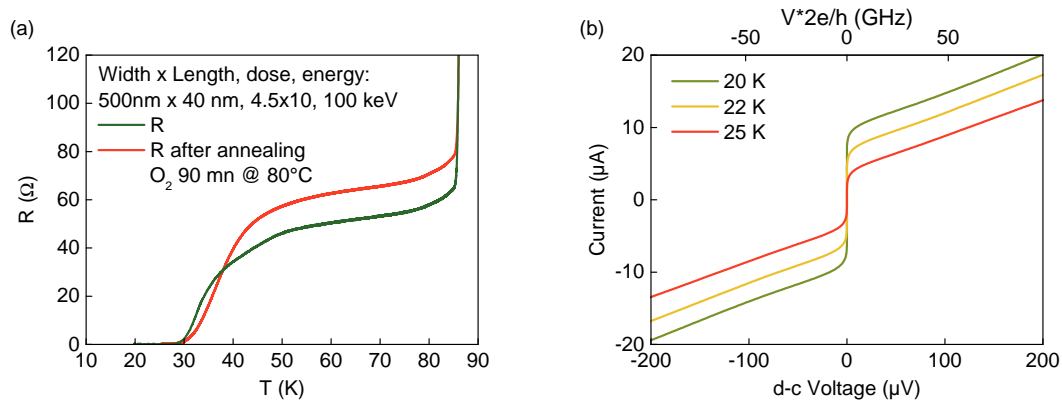
Figure 5.10: (a) RT curves before (green line) and after (red line) annealing of a 500 nm wide junctions. (b) IV curves of the junction at 20 K, 22 K and 25 K.
