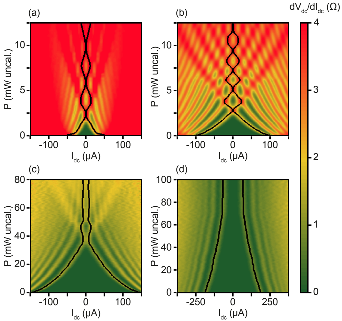
Figure 5.5: Differential resistance of junction (color scale) under a 20 GHz illumination, as a function of current bias and r-f power for different temperatures: (a) T = 56 K; (b) T = 53 K; (c) T = 42 K; (d) T = 35 K. The critical current ( n = 0 step) as a function of r-f power is shown in full back line. Complete oscillations of the current height of the Shapiro steps can be seen only in the Josephson regime T_c^! < T < T_j (panels (a)–(c)). In the flux flow regime, the critical current is never reduced to zero (panel (d)).
