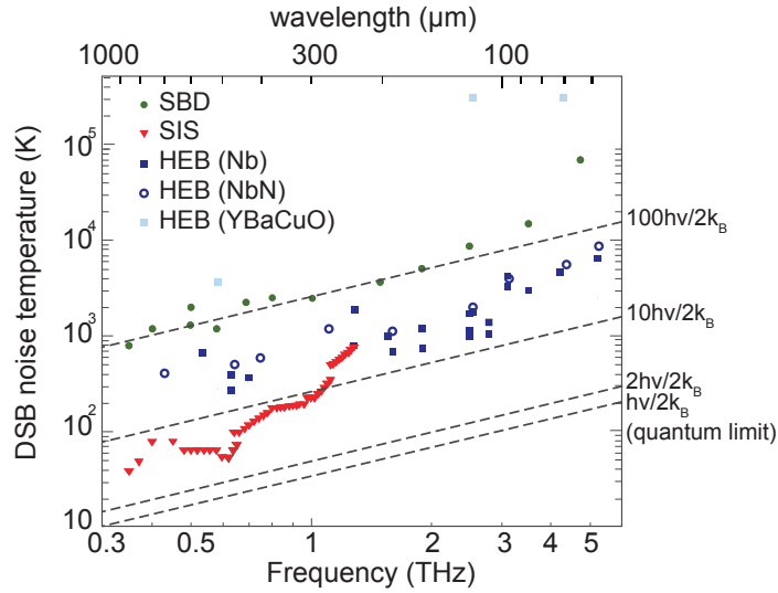
Figure 1.15: Comparison of DSB noise temperatures of the different mixer technology. Adapted from [173].
