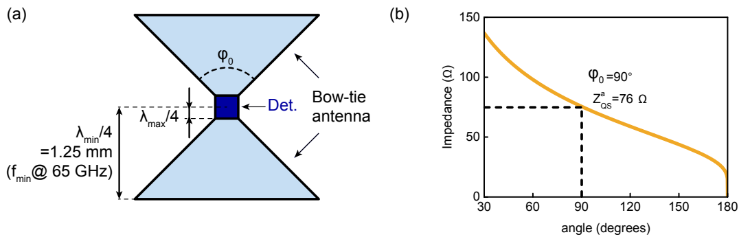
Figure 8.1: (a) Sketch of a bow-tie antenna, a detector being placed at its center. The minimum and maximum length of the arms determine the operating frequency band. (b) QS impedance of the bow-tie as a function of its angle \phi_0 .
