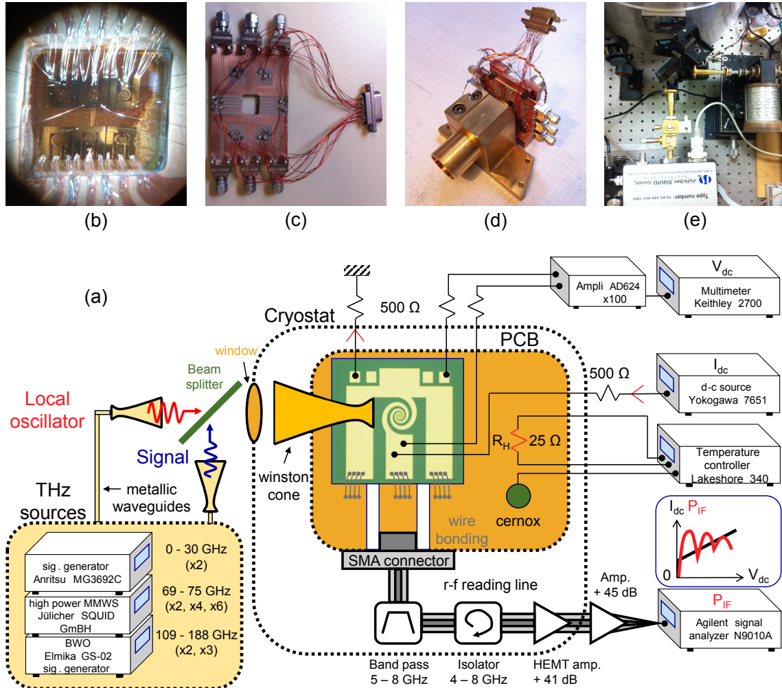
Figure 7.1: (a) Schematic of the experimental setup to test heterodyne detection of the Josephson mixer. Junction is embedded in a spiral antenna at the center of a CPW transmission line. It is d-c biased and the microwave line reads the intermediate frequency between 4 and 8 GHz. LO and the signal are sent from outside the cryostat through a window (mylar 50 \mu\text{m} ), guided through a quasi-optic setup onto the antenna. (b) Picture of the electronic chip, wire-bonded in d-c and in r-f onto the PCB. Many wires are required to connect the r-f line, in order to minimize their inductive effect. (c) Photograph of the homemade PCB. (d) Photograph of the whole cryogenic quasi-optic system: PCB and chip are glued to a copper plate and placed in front of the Winston cone. The whole mount is then placed on the 4 K stage of the cryostat, the copper plate being thermally decoupled. (e) Picture of the local oscillator and signal sources, placed in front of the cryostat window and coupled with a beam splitter.
