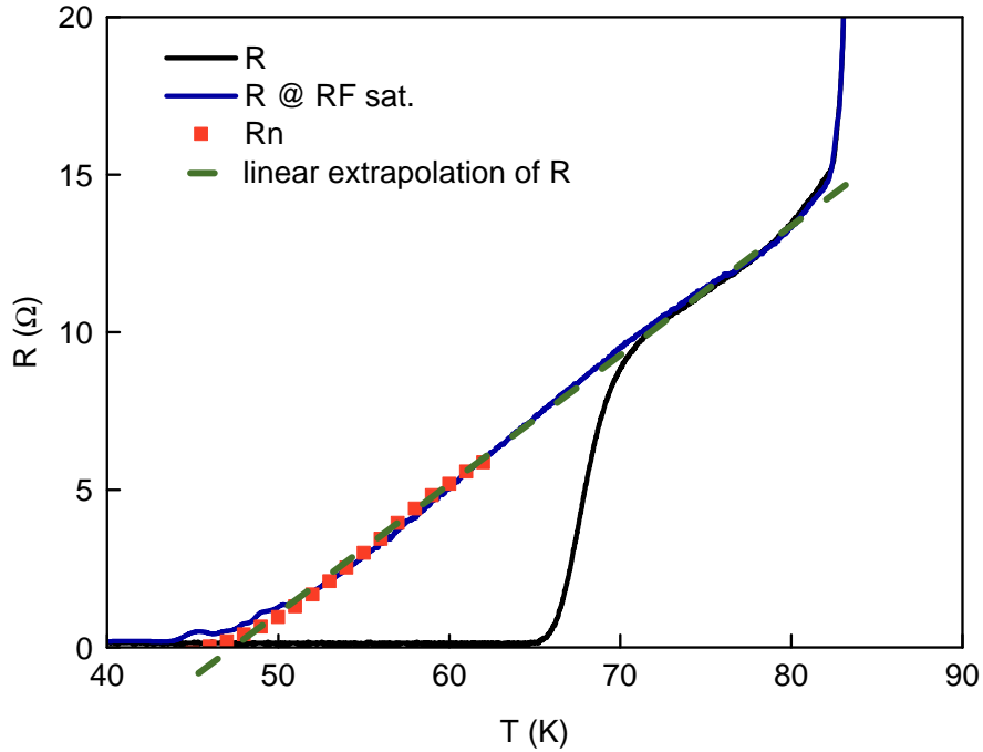
Figure 5.7: Three different methods to extract the normal state resistance R_n . Resistance measured when the junction is saturated with r-f (blue curve), linear extrapolation of the normal state resistance (dashed green line), and obtained from the derivative of IV curves (red squares).
