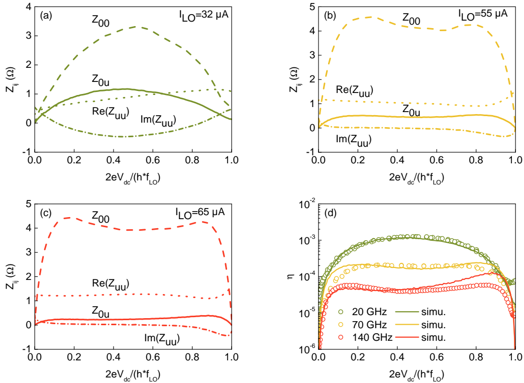
Figure 7.6: Main elements of the impedance matrix as a function of normalized voltage calculated at T = 58 K for f_{LO} = 20 GHz (panel a), f_{LO} = 70 GHz (panel b) and f_{LO} = 140 GHz (panel c). For all the curves, I_c = 45 \mu A and \Gamma = 0.057 . The value of I_{LO} is indicated on each panel. (d) Comparison between experimental (circles) and theoretical (full lines) conversion efficiency \eta calculated for the three LO frequencies.
