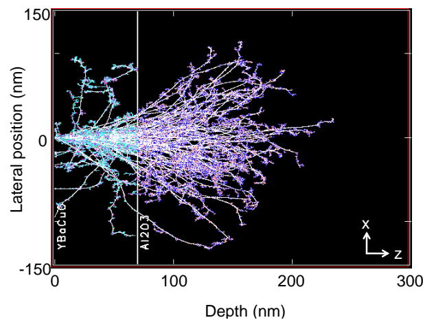
Figure 2.2: Simulation of 100 O^+ ions implanted at 110 keV in a 70 nm YBa_2Cu_3O_7 film, projected in the (x, z) plane. The trajectories of implanted ions are white, the recoil oxygen atoms are blue and the recoil copper atoms are violet. In Al_2O_3 the recoil oxygen atoms and aluminum are respectively violet and orange.
