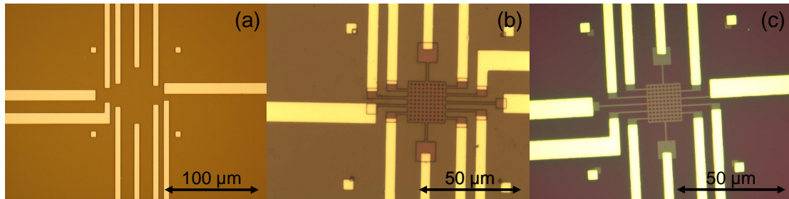
Figure B.1: (a) Optical photo of d-c Au contacts on \text{YBa}_2\text{Cu}_3\text{O}_7 , after the IBE. (b) Optical photo of the same contacts connected to a design of a 10 \times 10 2D array, after the second e -beam lithography. (c) Optical photo of the same design after the third e -beam lithography. The slits (brown thin lines inside the square matrix) appear on the PMMA.
