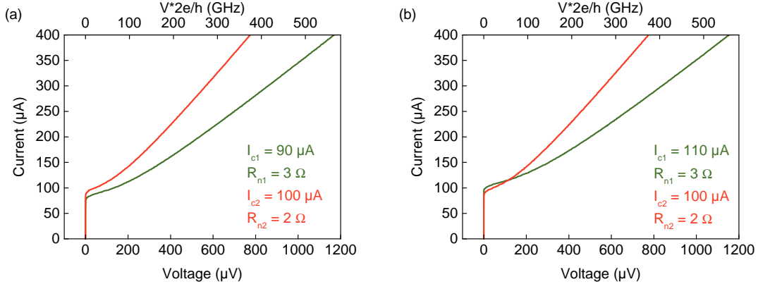
Figure 9.9: IV characteristics of series junctions without a feedback loop Depending on their I_c and R_n , the curves never cross (a) or cross only once (b).
