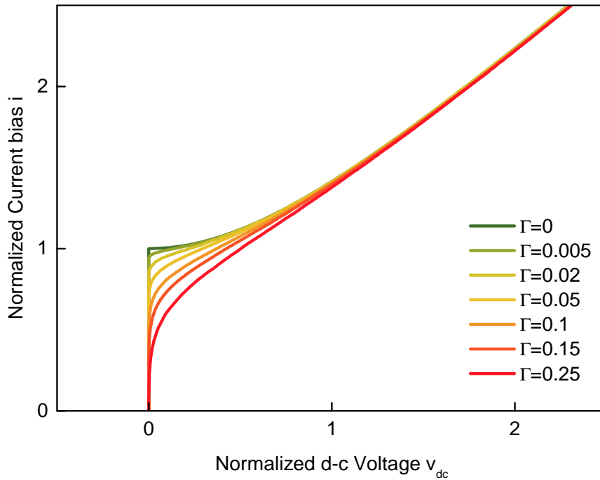
Figure 3.10: IV curves in the RSJ model (zero capacitance), in the presence of noise, for several values of normalized temperature.
