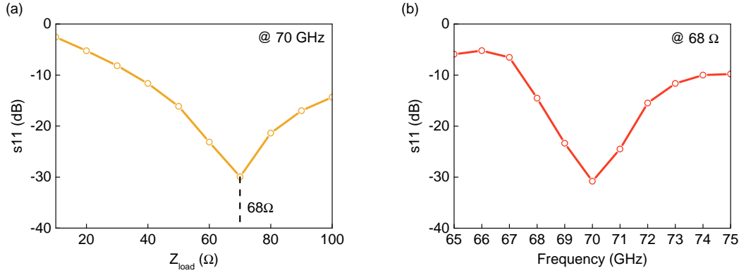
Figure 8.2: (a) reflection coefficient s_{11} of the antenna, at 70 GHz, as a function of the lumped element impedance, reaching a minimum at 68 \Omega . (b) s_{11} as a function of frequency when the lumped element impedance is fixed at 68 \Omega .
