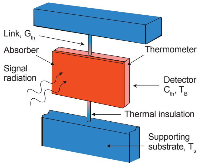
Figure 1.12: Schematic diagram of a thermal detector. Adapted from [173].
