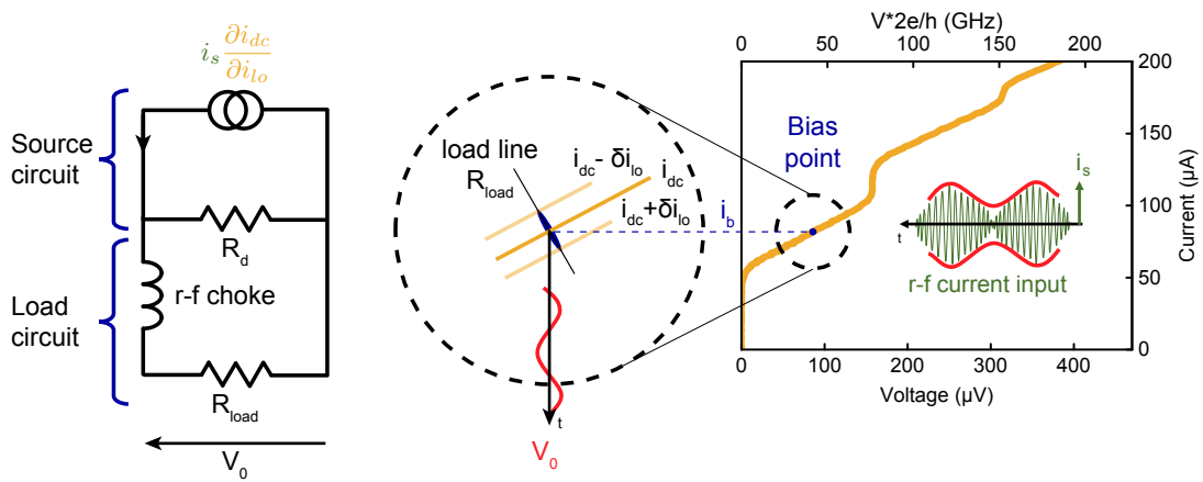
Figure 6.4: Effect of the LO on the IV curve of a Josephson junction, and equivalent circuit at the IFB.
