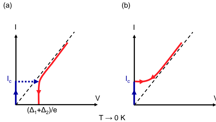
Figure 3.2: Schematic current-voltage curves of a tunnel (a) and a weak-link (b) Josephson junction. The quasiparticle branch is in red and the Josephson branch is in blue, signature of a supercurrent that flows at V = 0 up to the critical current I_c . In a tunnel junction there is no quasiparticle tunneling below the gap while in a weak-link junction a current exists even at low voltages.
