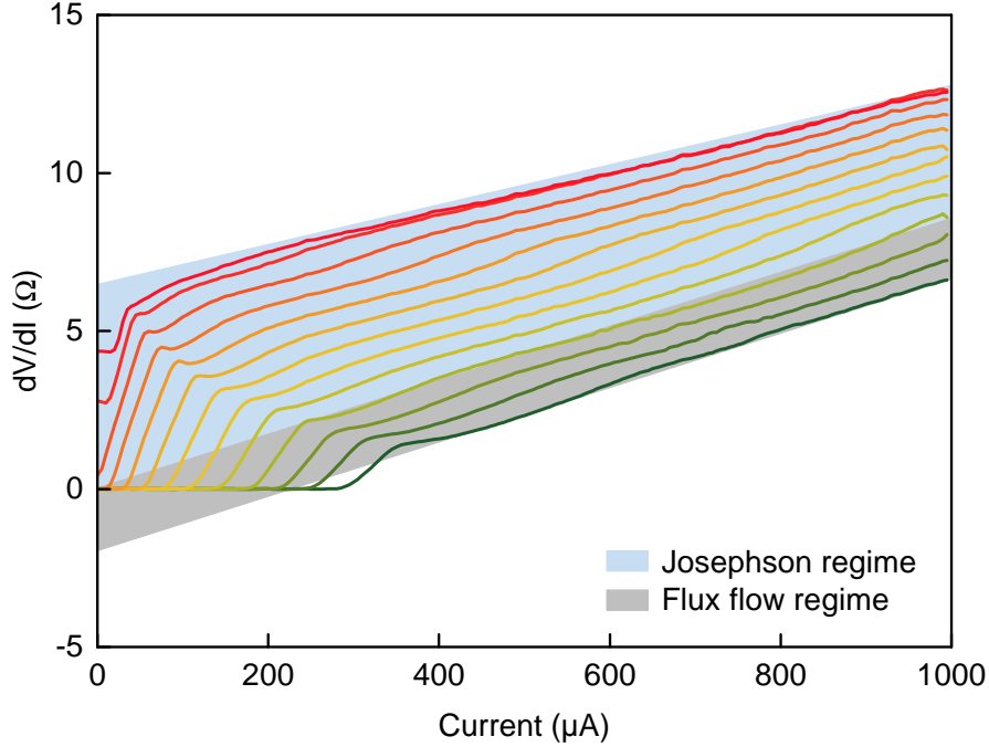
Figure 5.6: Numerical derivation of IV curves presented in 5.3 (b), dV_{dc}/dI as a function of current bias. The linear extrapolation to I = 0 gives the normal resistance R_n . Below 46 K it gives a negative resistance and we enter the flux flow regime.
