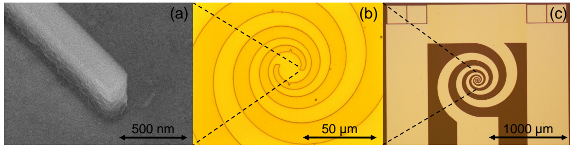
Figure 2.9: (a) SEM picture (taken with a tilted angle of 30^\circ ) of a MAN-2505 resist line patterned with e-beam lithography, on a gold layer. (b) Optical photo of a MAN-2405 spiral design (dark yellow areas) on a gold layer. (c) Optical photo of such a spiral embedded in a microwave transmission line after the ion beam etching.
