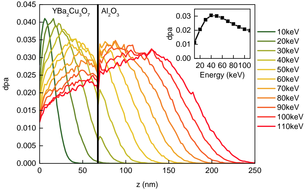
Figure 2.3: Simulations of the plain sheet \text{dpa}_{ps} as a function of the depth z . Inset: simulation of the total plain sheet \text{dpa}_{ps} for z < 70 . The dose is 5 \cdot 10^{13} ions. \text{cm}^{-2} . The simulated sample is a \text{YBa}_2\text{Cu}_3\text{O}_7 layer on top of the \text{Al}_2\text{O}_3 substrate, as in figure 2.2.
