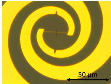
Figure 2.11: Optical photo of a 40 nm slit patterned in the PMMA, prior to the second ion implantation.
