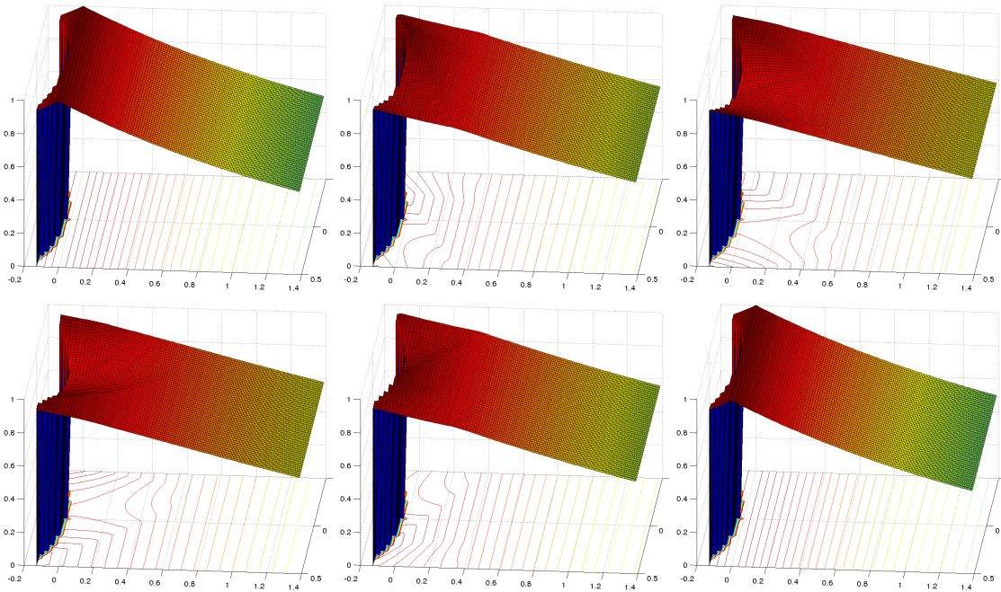
Figure 8.3: Mean rate of injectivity on SL_2(\mathbf{R}) on the fundamental domain \mathcal{D} (more precisely, \mathcal{D} = \{z \in \mathbf{C} \mid |z| > 1, \text{Im } z > 0, -1/2 < \text{Re } z < 1/2\} ) of the modular surface, for various angles in T^1\mathcal{D} ( 0, \pi/10, \pi/5, 3\pi/10, 2\pi/5, \pi/2 ).
