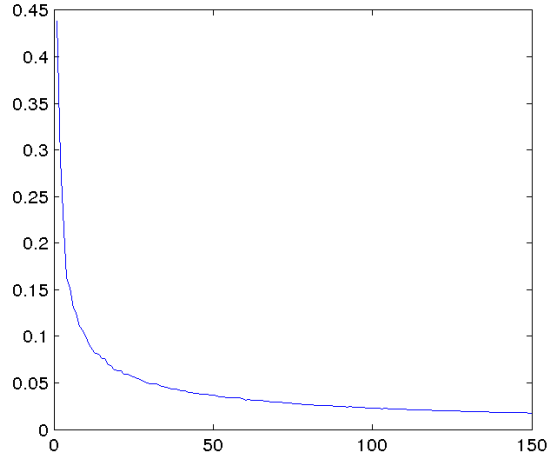
Figure 11.2: Simulation of the degree of recurrence D((f_5)_N) depending on N , on the grids E_N with N = 128k , k = 1, \dots, 150 .
