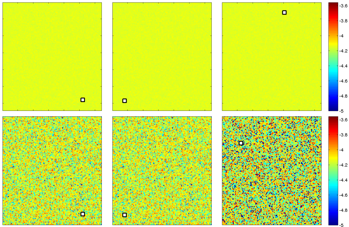
Figure 12.12: Simulations of invariant measures \mu_x^{(h_3)N} on the grid E_N , with N = 2^{23} + 1 (top) and N = 2^{23} + 17 (bottom), and x a random point of \mathbb{T}^2 , represented by the black and white box. The behaviour observed on the three top pictures is the most frequent (for 17 over the 20 orders N = 2^{23} + i , i = 0, \dots, 19 , all the 100 random draws we have made gave a measure very close to Leb), but seldom we also observe measures further from Lebesgue measure, like what happens for N = 2^{23} + 17 (bottom), where 99 over the 100 random draws of x produce a measure identical to the two first pictures, and the other random draw gives a measure a bit more singular with respect to Lebesgue measure (bottom right).
