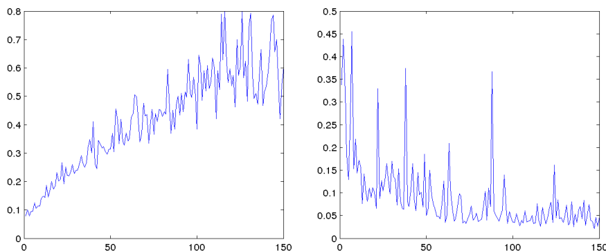
Figure 5.8: Distance between Lebesgue measure and the measure \mu_{\mathbb{T}^2}^{(f_i)_N} depending on N for f_3 (left) and f_4 (right), on the grids E_N with N = 128k , k = 1, \dots, 150 .
