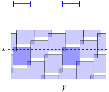
Figure 8.19: First case of Lemma 8.52, in the case \ell = 3 : the set W^{k+1} + \tilde{\Lambda}_{k+1} auto-intersects.
