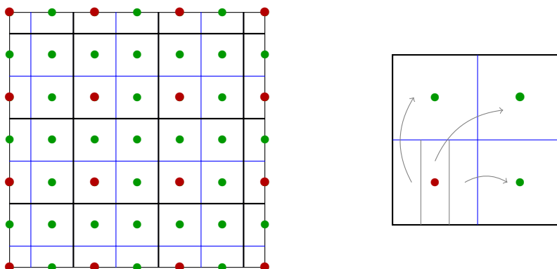
Figure 5.3: Construction 7 of Lemma 5.32 for two grids of orders 3 and 6 and zoom around a point of a grid of order 3
