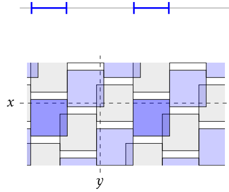
Figure 8.20: Second case of Lemma 8.52, in the case \ell = 3 : two distinct vertical translates of W^{k+1} + \tilde{\Lambda}_{k+1} intersect (the first translate contains the dark blue thickening of W^k + \tilde{\Lambda}_k , the second is represented in grey).
