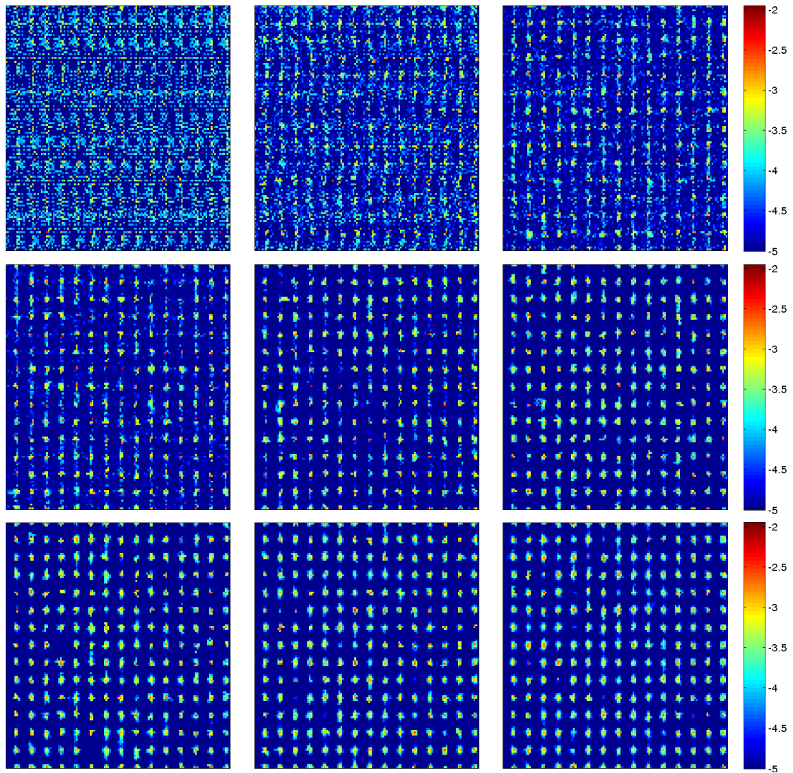
Figure 4.5: Simulations of \mu_{\mathbb{T}^2}^{(f_2)^N} on grids E_N , with N = 2^k , k = 7, \dots, 15 (from left to right and top to bottom).
