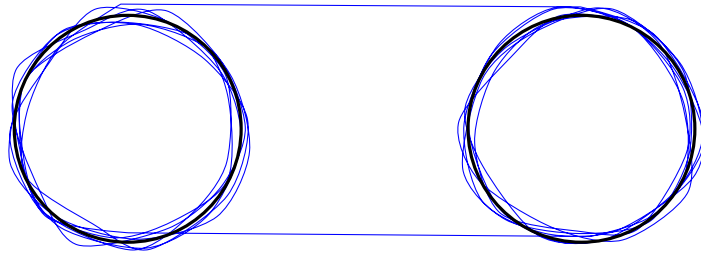
Figure 5.5: Construction of Lemma 5.46: the measure carried by the blue cycle is close to a convex combination of the measures carried by the black cycles
