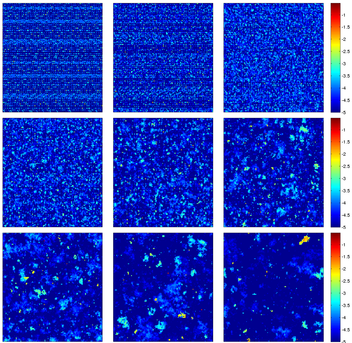
Figure 5.9: Simulations of invariant measures \mu_{\mathbb{T}^2}^{(f_3)_N} on the grids E_N , with N = 2^k , k = 7, \dots, 15 (from left to right and top to bottom).
