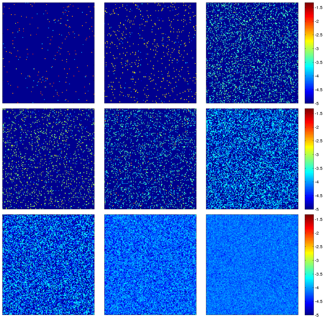
Figure 12.16: Simulations of invariant measures \mu_{\mathbb{T}^2}^{(f_6)_N} on the grids E_N , with N = 2^k , k = 7, \dots, 15 (from left to right and top to bottom).
