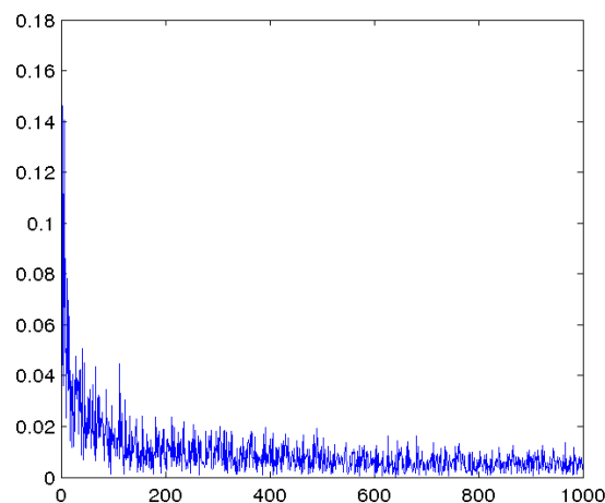
Figure 11.6: Simulation of the degree of recurrence D((f_5)_N) of the expanding map N , depending on N , on the grids E_N with N = 128k , k = 1, \dots, 1\,000 .
