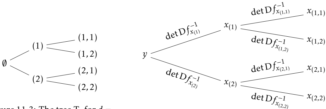
Figure 11.3: The tree T_2 for d = 2 .
