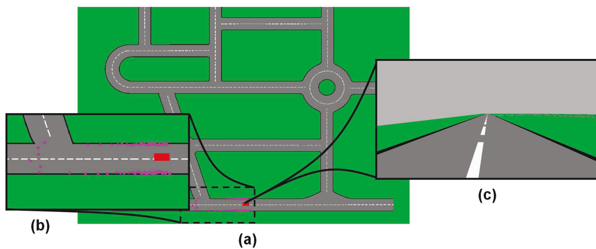
Figure 3.12 – Simulation platform (with a simulated urban environment, vehicle and sensors) to validate the proposed navigation approach in the car-like robot in red (a). The simulated laser scanner measurements are illustrated in pink (b), as well as the image view from a simulated monocular camera with the same parameters of the real one (c).
