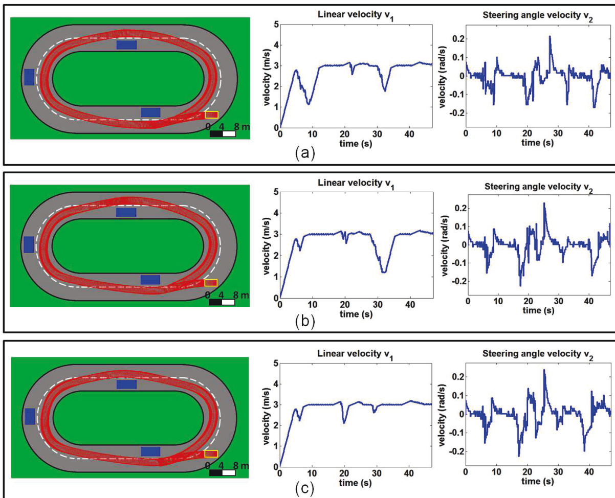
Figure 5.6 – Tuning process for the gains associated with the IDWA, where: (a) \alpha_1 = \alpha_2 = 0.1, \beta = 1.0, \text{ and } \gamma = 1.0 ; (b) \alpha_1 = \alpha_2 = 0.1, \beta = 1.0, \text{ and } \gamma = 3.0 ; and (c) \alpha_1 = \alpha_2 = 0.1, \beta = 2.0, \text{ and } \gamma = 3.0 . The car initial pose is represented in yellow, the obstacles are in blue, and in red are the car instantaneous positions for a clockwise movement.
