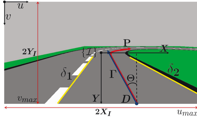
Figure 4.10 – Image frame \{\mathcal{I}\} representation for the camera frame \{\mathcal{C}\} . The road lane center P (in red) is related to the boundaries \delta_1 and \delta_2 (in yellow). Its tangent \Gamma (in blue), at the point D and angle offset \Theta from \Gamma to the axis -Y , defines the image features X , Y , and \Theta .
