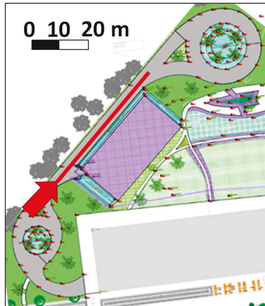
Figure 5.10 – Robot course (red line) for the local navigation experiments at the SEVILLE test track. All experiments start in the arrow.
