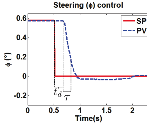
Figure 3.11 – Step response for the steering angle actuator to estimate the dead time t_d and time constant \tau . SP is the current control setpoint and PV is the process value.
