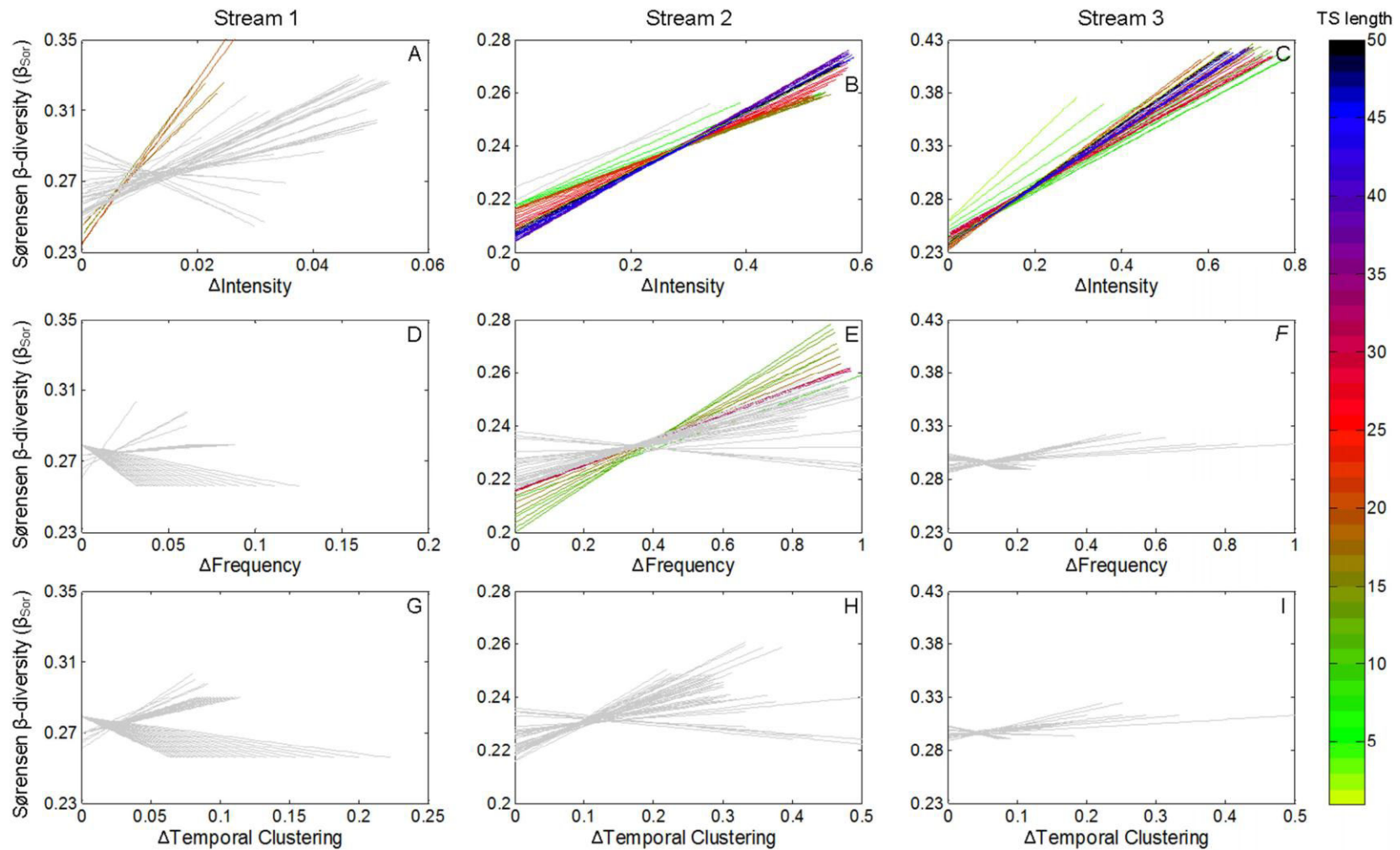
Figure 3: Predictions of the linear regression models of the Sørensen \beta -diversity ( \beta_{sor} ) vs. the difference in intensity ( \Delta I , A-C), frequency ( \Delta f , D-F), and temporal clustering ( \Delta C , G-I) for the three study sites. Predictions of the linear regression models were calculated for time series length from 2 to 50 days before the 14 sampling dates. Colors correspond to the length of the time series. Grey regression lines correspond to non-significant relationships.
