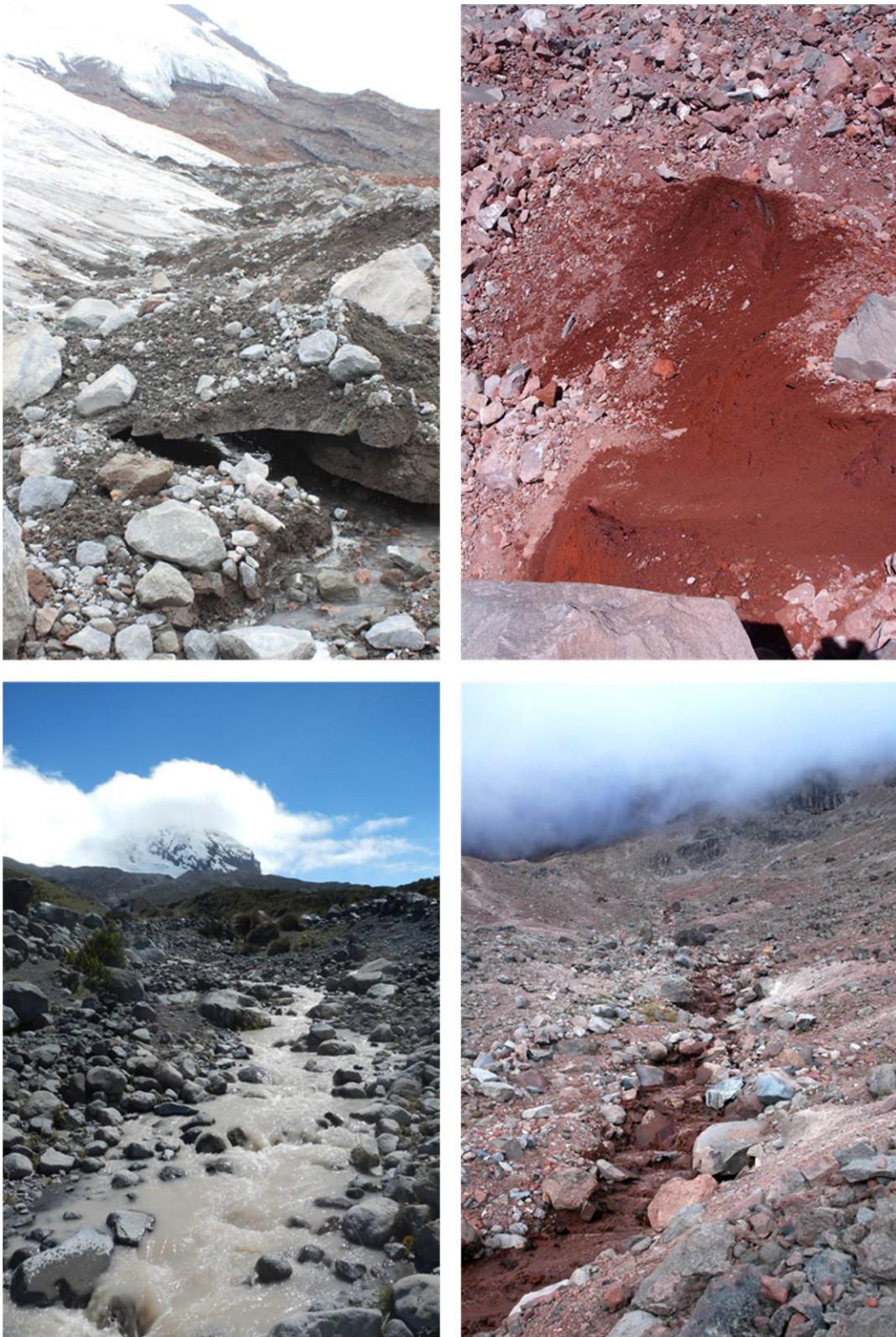
Figure 6: Picture of glacial flour (top) and glacier-fed streams (bottom) with high turbidity. Nature of sediments in the streams and on the glacier margin depends on bedrock composition. Pictures on the left side were taken in the Antisana reserve, while pictures on the right side in the Chimborazo, two volcanoes in the tropical Andes in Ecuador.
