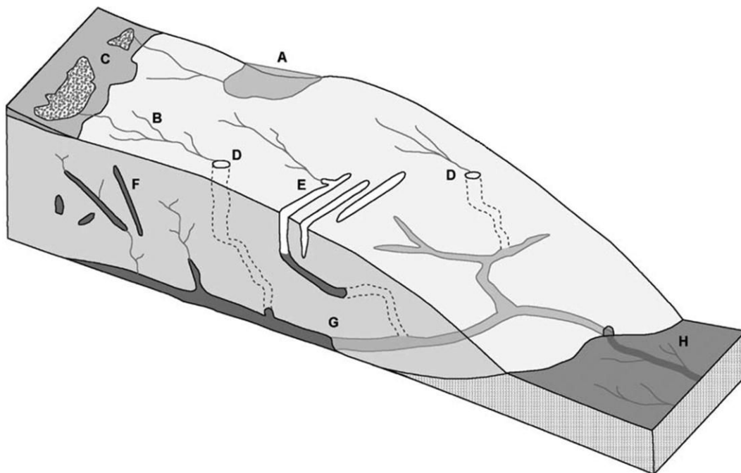
Figure 3: Some elements of the glacier water system. A: Supraglacial lake. B: Surface streams. C: Swamp zones near the edge of the firn. D: Moulin, draining into subglacial tunnels. E: Crevasses receiving water. F: Water-filled fractures. G: Subglacial tunnels, which coalesce and emerge at the front. H: Runoff in the glacier foreland, originating from tunnels and also from upwelling groundwater. Figure taken from Cuffey and Paterson (2010).
