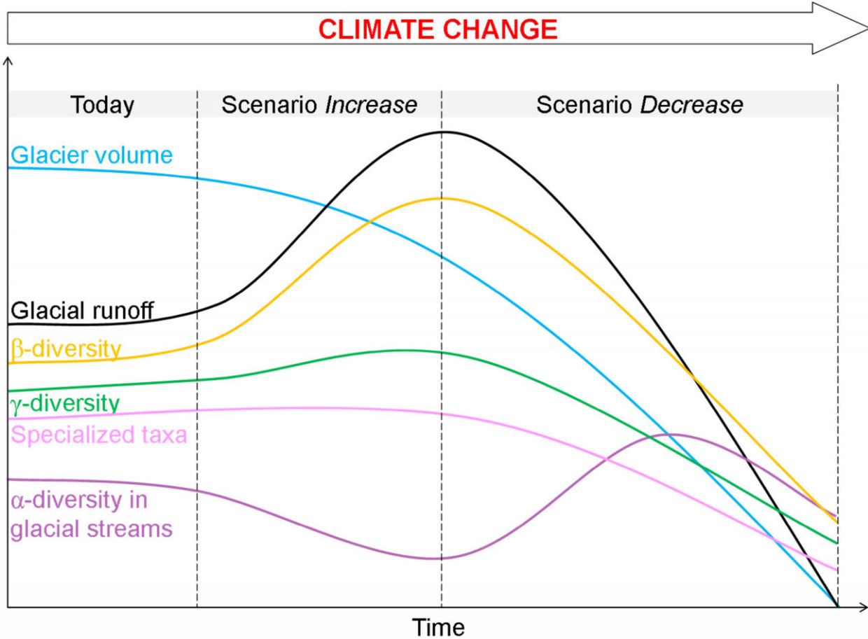
Figure 2: Conceptual diagram illustrating the expected temporal changes in \alpha -diversity in glacier-fed stream, in spatial \beta -diversity, \gamma -diversity, and number of specialized taxa (in both glacial streams and headwater groundwater streams) within the glacierized catchment according to glacial runoff fluctuation during glacial shrinkage.
