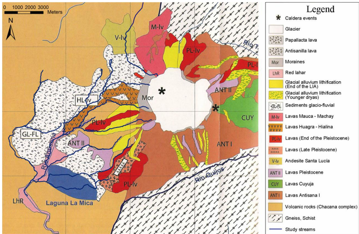
Figure 12: Geological map of the Antisana volcano. Image was taken from Hall et al. (2012), georeferenced and modified in ArcGis (10.0). Study streams were added in blue.
