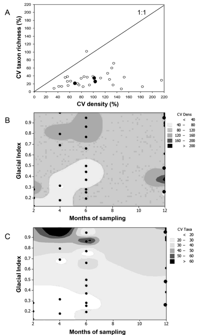
Figure 4. Coefficient of variation (CV) in taxon richness as a function of CV in density at various sites in different streams (A), and CV in density (B) and taxon richness (C) as a function of the Glacial Index (GI) and the number of months that the sampling covered. The GI was proposed by Jacobsen and Dangles (2012) as a proxy for environmental harshness. Values close to 1 are obtained close to large glaciers (see Methods for details). Large black dots = this study. Data from Brown et al. (2006), Robinson et al. (2001), Burgherr and Ward (2001), Lods-Crozet et al. (2001), Schütz et al. (2001), and this study.
