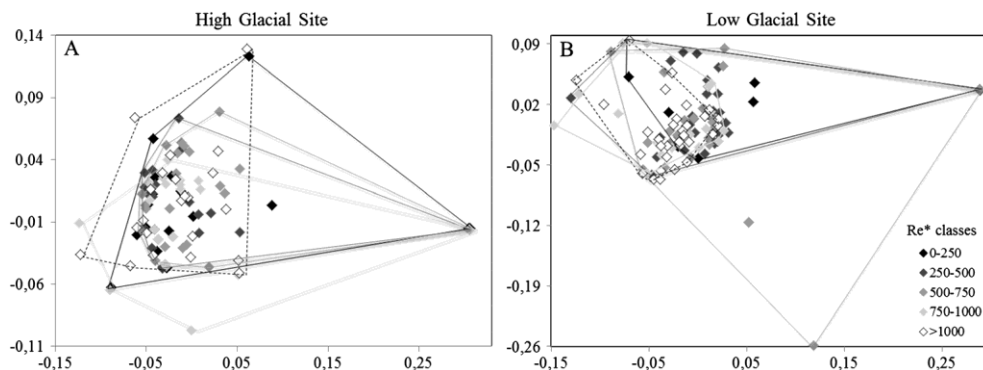
Figure 7. Non-metric multidimensional scaling ordination of log-transformed macroinvertebrate community data in the both high glacial (A) and low glacial (B) sites. The five different classes of boundary Reynolds number are shown (stress = 0.3622 and 0.3058 for high glacial and low glacial site, respectively)
