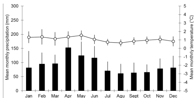
Fig. 2. Mean monthly precipitation (bars) and temperatures (dots) over 1 yr at the Antisana volcano, Ecuador. The weather station is located on the proglacial margin of Glacier 15 at 4850 m. Mean values and standard deviations were calculated over 6 yr (2005–2010).
