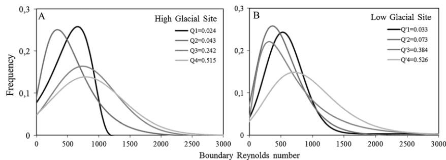
Figure 2. Frequency distribution of boundary Reynolds number values for the four discharges observed during the study. For both high glacial (A) and low glacial (B) sites, two discharges corresponding to base-flow conditions ( Q_1 , Q_2 and Q'_1 , Q'_2 for high glacial and low glacial site, respectively) and two others: one corresponding to a moderate glacial flood pulse ( Q_3 and Q'_3 for high glacial and low glacial site, respectively) and one corresponding to a high glacial flood pulse ( Q_4 and Q'_4 for high glacial and low glacial site, respectively). Each flood event corresponds to one date
