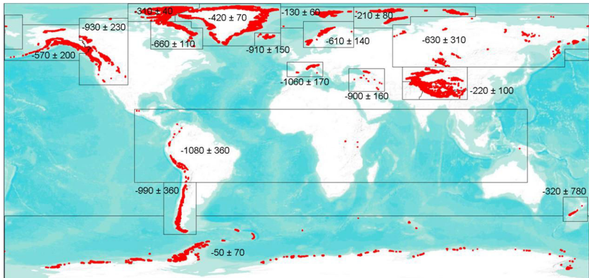
Figure 4: Regional glacier mass change rates in \text{kg m}^{-2} \text{yr}^{-1} for the period 2003-2009. Mean mass changes with the 95% confidence intervals are available for each Randolph Glacier Inventory region (see Gardner et al. 2013). Glacier outlines were taken from the Randolph Glacier Inventory ( http://glims.org/RGI/ ). The map was made using ArcGis (10.0).
