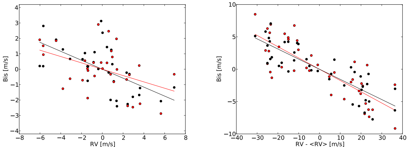
Figure 4.11: This example shows the comparison between the bisector-span derived by the CCF (red) and the experimental RV_{\chi^2-bis} (black) from NAIRA. Left panel corresponds to data from G1 674 ( P_{rot} \approx 35 d ), a star with a planetary companion – which signal was removed – and an active region; the RMS of the linear fits are 1.27 (CCF) and 1.18 (NAIRA). In the right panel I used data from the very active star G1 388 (AD Leo, P_{rot} \approx 2.24 d ), in this case the RMS of the linear fits are 2.54 (CCF) and 1.94 (NAIRA).
