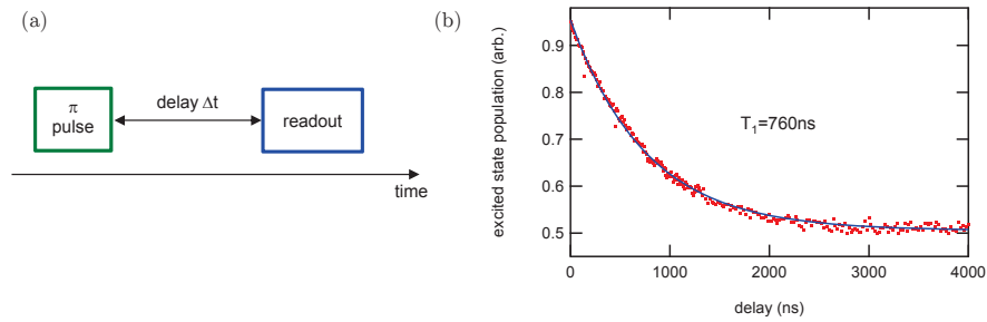
Figure 2.8: T_1 measurement. (a) Pulse sequence. (b) Population of the excited state as a function of the delay time \Delta t .
