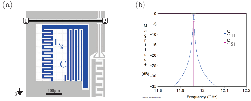
Figure 3.16: Readout resonator coupled to the transmission line. (a) drawing placed in the simulator. (b) simulated reflection ( S_{11} ) and transmission ( S_{21} ) parameter as a function of the frequency.
