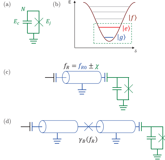
Figure 1.2: (a) Cooper pair box circuit: a Josephson junction of Josephson energy E_j in parallel with a capacitance with charging energy E_c = (2e)^2 / 2C . (b) Josephson potential energy of the Cooper pair box as a function of the phase difference \delta across the junction. Energy levels of the Cooper pair box in the transmon regime. The two first level of this anharmonic spectrum define a qubit. (c) Circuit QED qubit architecture: a Cooper pair box is capacitively coupled to a microwave resonator. The resonator frequency change ( \pm\chi ) with the qubit state is used for qubit readout. (d) Josephson bifurcation (JBA) readout scheme used in this thesis. The Josephson junction embedded in the readout resonator makes it non linear; the switching between two dynamical states of the resonator occurs at a rate \gamma_B depending on the qubit state; this switching can provide high fidelity qubit readout.
