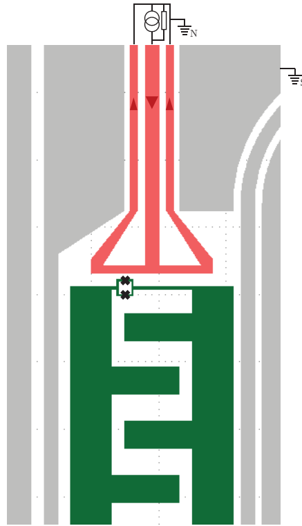
Figure 3.14: Design of our flux lines. The colors are only given for The qubit is in green while the flux line is in red. The ground symbol “S” (“N”) represents connection to the main ground via superconducting (normal) material.
