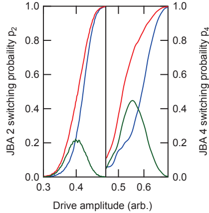
Figure 6.5: Measured switching curves for JBA 2 (left) and JBA 4 (right), for the qubit in its ground (blue) and excited state (red), as a function of the drive amplitude. The green curves are the corresponding differences, or contrast of a \pi pulse.
