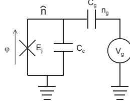
Figure 2.4: The Cooper pair box: schematic electrical circuit.
