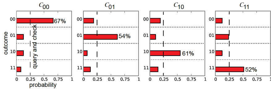
Figure 2.29: Single-run success probabilities of the implemented Grover search algorithm, for the 4 possible oracle operators. The success probability is always larger than the success probability of the query-and-check classical algorithm.
