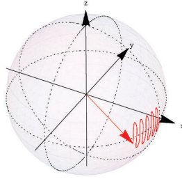
Figure 3.3: Spurious Rabi oscillation in the Bloch sphere
