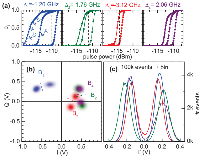
FIG. 3. (Color online) Simultaneous readout of the four qubits at a magnetic field such that \Delta_{1-4}/2\pi = (-1.2, -1.76, -3.12, -2.06) GHz. (a) Switching probabilities p_i of the four readouts as a function of readout power P_R , after no control pulse (right curves in each panel), and after a \pi_1^{01} pulse without (middle) and with shelving (left curves for B_{1,2,3} ). Dashed vertical lines indicate the optimal readout powers used in (b) and (c) and in Fig. 4 (shelving used only for B_2 and B_4 ). (b) Density plots of the four (I_i, Q_i) obtained from 10^5 measurements. Segments indicate the separatrices between switching and nonswitching events. (c) Corresponding histograms along the lines perpendicular to separatrices.
