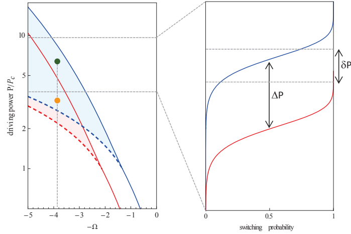
Figure 2.17: (a) Stability diagram for the two possible qubit states |g\rangle (blue) and |e\rangle (red) for a typical operating point (green). (b) Switching probability as a function of the power for the selected frequency.
