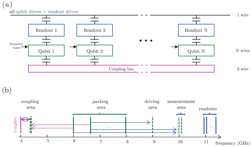
Figure 3.1: (a) ' N+1 architecture' of a simple N -qubit processor with a single wire used for drives and readouts, and N wires to control the qubit frequencies. (b) Frequency domain overview of the processor: qubit frequencies are shown (green) at various positions corresponding to different operation (parking, driving, coupling and readout), whereas coupling bus (magenta) and readout resonators (blue) are fixed.
