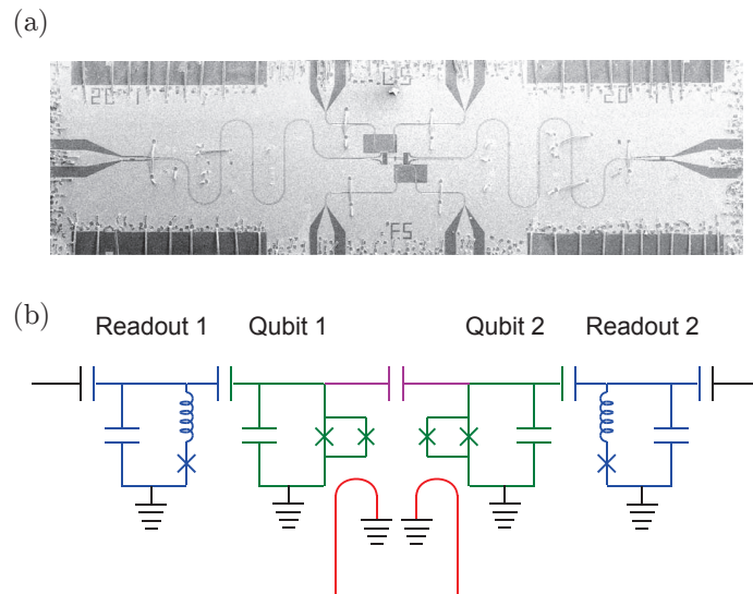
Figure 1.3: Two-qubit processor. (a) Optical micrograph of the two-transmon qubit circuit. (b) Electrical equivalent scheme. The qubits are capacitively coupled, and each of them is fitted with its non-linear readout resonator.
