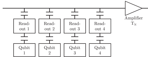
Figure 3.6: Multiplexed readout method
