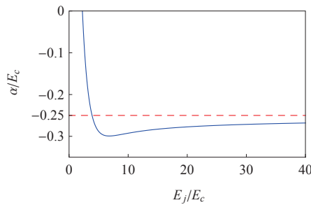
Figure 2.6: Reduced anharmonicity \alpha/E_c as a function of E_j/E_c
