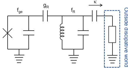
Figure 2.20: Electrical scheme of a transmon in a CQED geometry.
