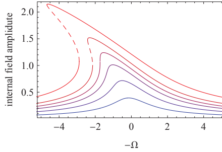
Figure 2.15: Internal field stationary amplitude for different reduced drive amplitudes \beta_c/10 , \beta_c/3 , 2\beta_c/3 , \beta_c , 3\beta_c/2 , and 3\beta_c (from blue to red). Dashed lines represent unstable solutions.
