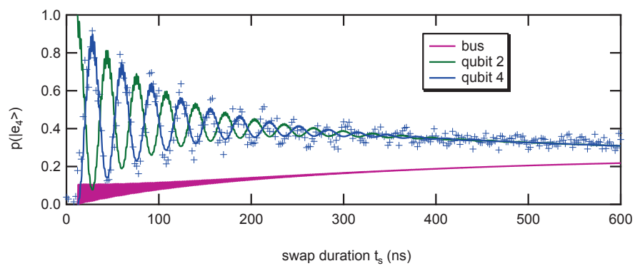
Figure 1.10: Coherent swapping oscillations between qubit 2 and qubit 4 mediated by coupling them through the bus resonator. The symbols are the measured excitation probability of qubit 4 corrected from readout errors. The solid lines are the simulated excitation probabilities of qubit 2 (green), qubit 4 (blue) and of the bus resonator (magenta).
