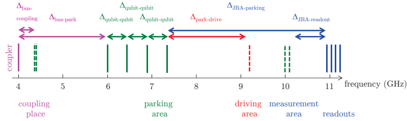
Figure 3.9: Overall frequency staging
