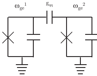
Figure 2.23: Electrical scheme of the capacitively coupled transmons.
