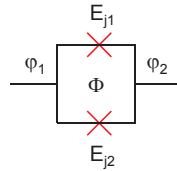
Figure 2.3: The SQUID: a flux controlled Josephson junction.
