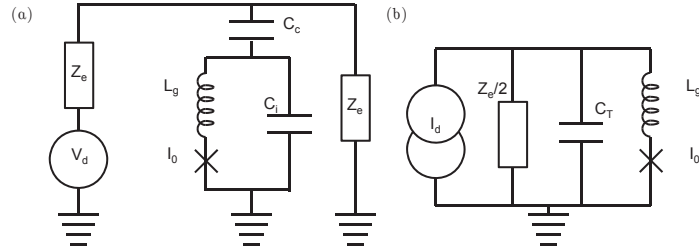
Figure 2.14: (a) Electrical scheme of a JBA. (b) Simplified equivalent circuit close to resonance, with I_d = V_d/Z_e and C_T = C_j + C_c .
