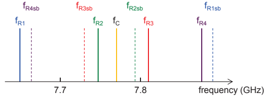
Figure 5.12: Readout frequency overview. The carrier frequency is f_c = 7.77 GHz, f_{Ri} stand for readout frequency and f_{Risb} represent the ideally canceled sideband.
