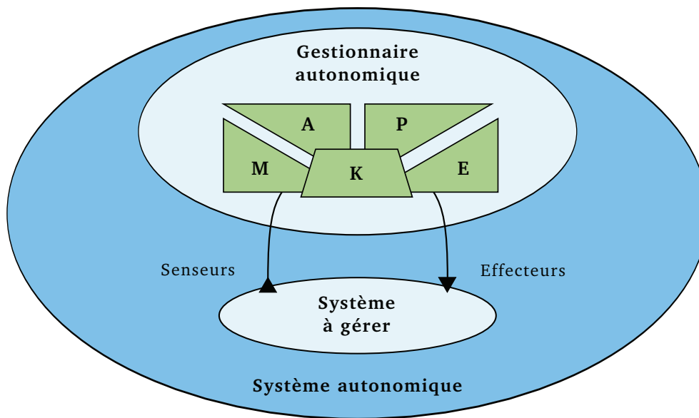
FIGURE 3.16 – Architecture MAPE-K
