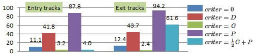
FIGURE 2.27: Percent of flights deviated from their desired tracks for different criteria included in the objective function
