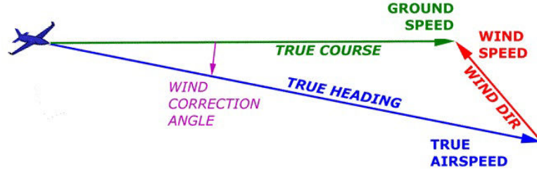
FIGURE 1.5: Aircraft true air speed (TAS), ground speed (GS) and wind speed (WS) triangle
