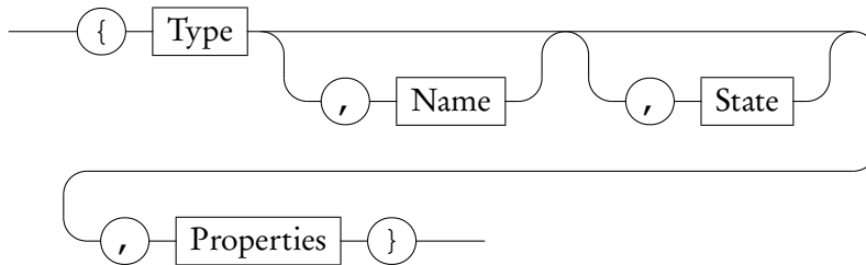
Figure 5.24: Syntax Diagram of Generic Resource
