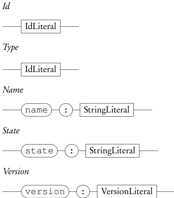
Figure 5.22: Id, Type, Name and State
