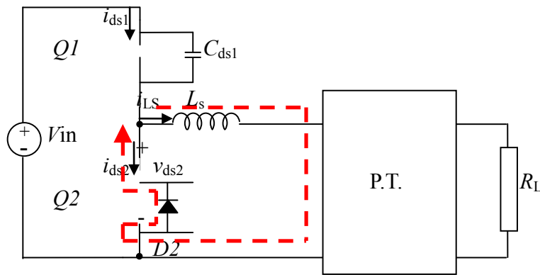
Figure 4-9. The operation of the ZVS-mode half-bridge circuit with a PT during mode 3
