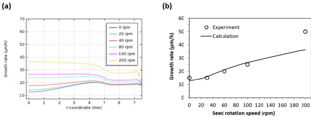
Fig. 6.11 (a) Growth rate profile along the seed radius for various rotation speed and (b) growth rates at the seed center plotted as a function of the rotation speed compared with the experimental results
