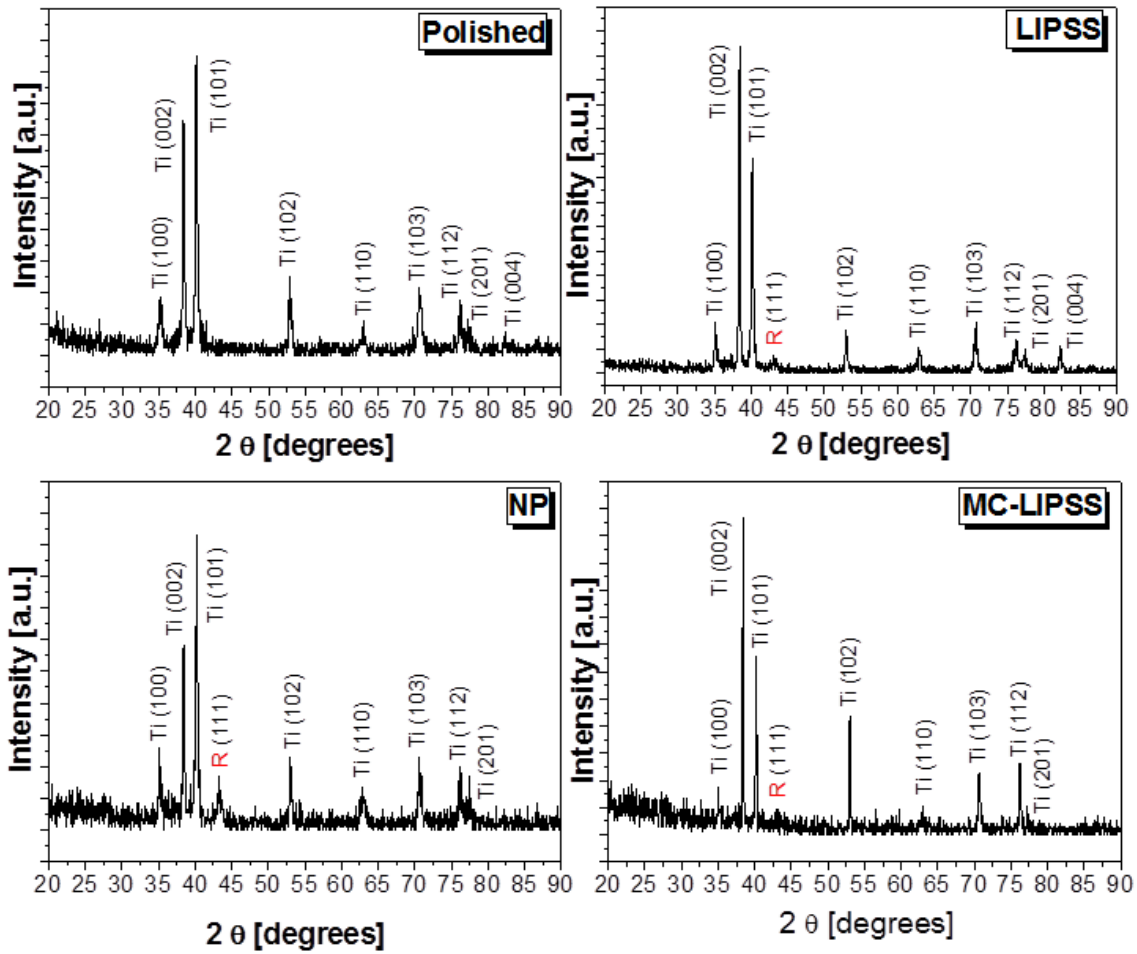
Figure III-18. X-ray diffractograms for cp Ti surfaces obtained by glancing incidence. A and R denotes the \text{TiO}_2 polymorphs anatase and rutile, respectively.
