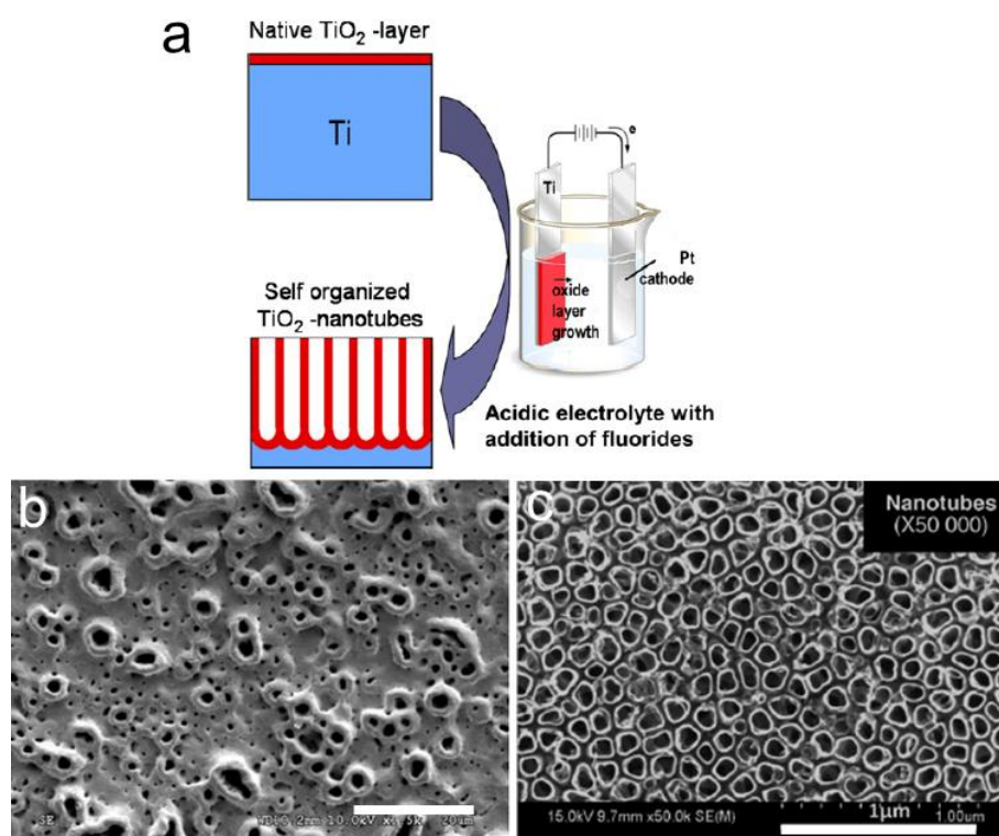
Figure I-9. Schematic setup for anodisation of titanium in fluoride containing electrolytes (a). SEM micrographs of \text{TiO}_2 micropores (b) and nanotubes (c) (adapted from [5, 11]). The scale bar is 20 \mu\text{m} (b) and 1 \mu\text{m} (c).
