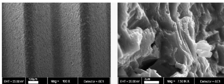
Figure I-7. Low and high magnifications SEM micrographs of a titanium surface blasted with \text{TiO}_2 particles (adapted from [54]). The scale bar is 100 \mu\text{m} (left) and 2 \mu\text{m} (right).
