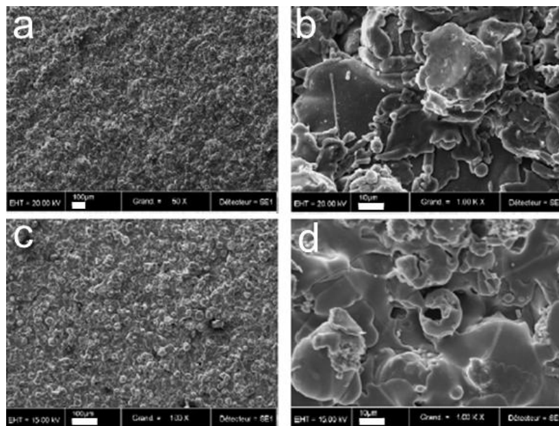
Figure I-6. Low and high magnifications SEM micrographs of plasma-sprayed titanium (a-b) and hydroxyapatite (c-d) coatings (adapted from [54]). The scale bar is 100\text{ }\mu\text{m} (a and c) and 10\text{ }\mu\text{m} (b and d).
