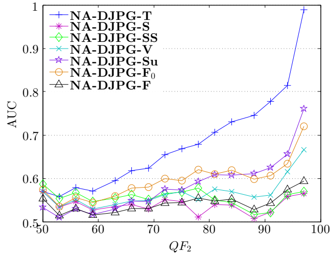
Figure 5.13: Average AUC value of the NA-DJPG compression detector [BP12a] as a function of QF_2 , when tested on NA-DJPG-R , created from UCIDTE. The improvement of forensic undetectability of NA-DJPG-F over NA-DJPG-F 0 shows the necessity of conducting the DCT histogram smoothing.
