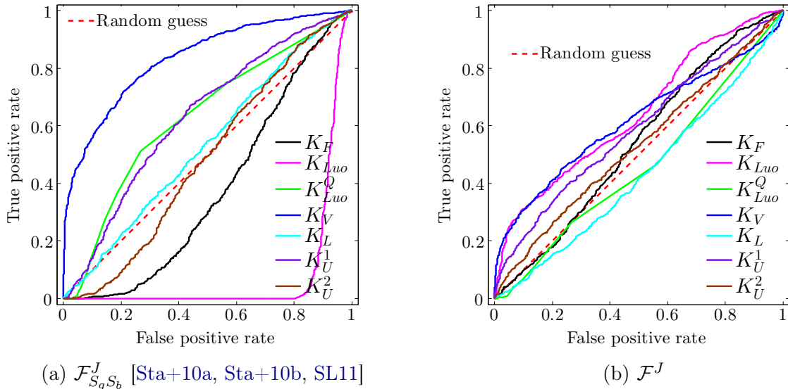
Figure 5.8: ROC curves achieved by \mathcal{F}^J and \mathcal{F}_{S_q S_b}^J [Sta+10a, Sta+10b, SL11] against JPEG forensic detectors. Results are obtained on UCIDTest dataset.
