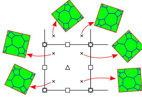
Fig. 17.1: Macroscale enhanced finite elements with REV orientation \theta^{REV} assigned randomly to the integration points.
