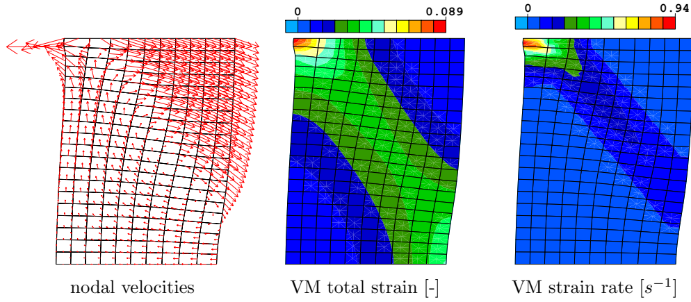
Fig. 14.11: Deformed meshes for D = 0.5kN (displacements multiplied 10\times ).
