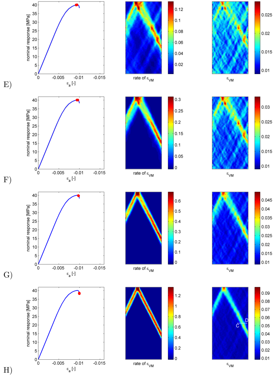
Fig. 17.7: Post-peak (rate of) Von Mises equivalent strain ( \varepsilon_{VM} ) for D = 25\ N .
