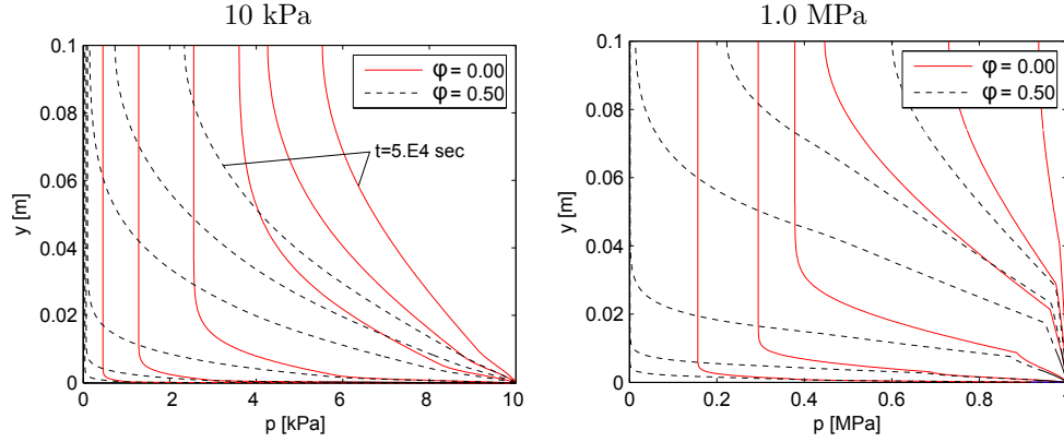
Fig. 10.4: Fluid pressure curves as a response to fluid pressure loading (Figure 10.3) at t=10, 100, 1000, 10,000, 25,000 and 50,000 seconds.
