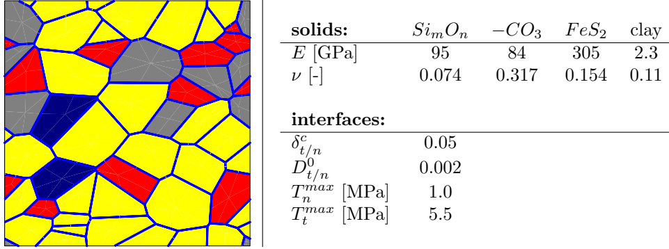
Fig. 14.3: Microstructure '8' with carbonate (gray), tectosilicate (red) and pyrite (deep blue) inclusions in a matrix of clay (yellow). Grain selection for material allocation has been performed randomly.
