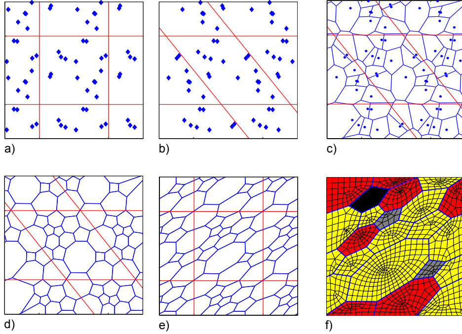
Fig. 11.1: Illustration of the algorithm for anisotropic REV generation with grain shape tensor T = \begin{bmatrix} 1 & 0.8 \\ 0 & 1 \end{bmatrix} .
