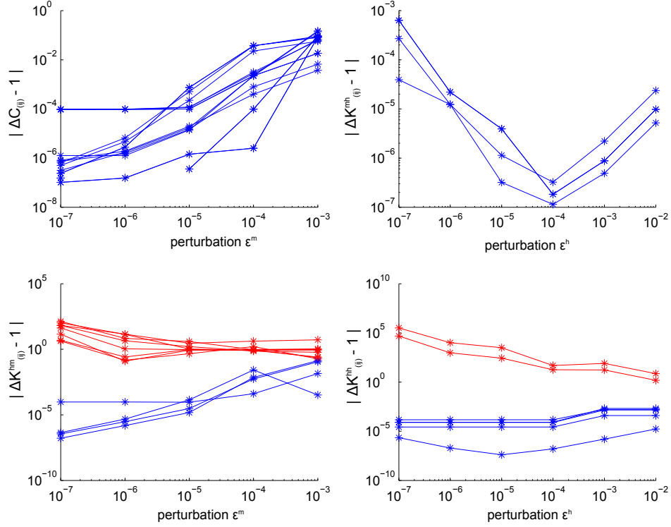
Fig. 9.4: Relative difference in the components of the tangent stiffness matrix [A_{(7 \times 7)}] for different perturbations \epsilon
