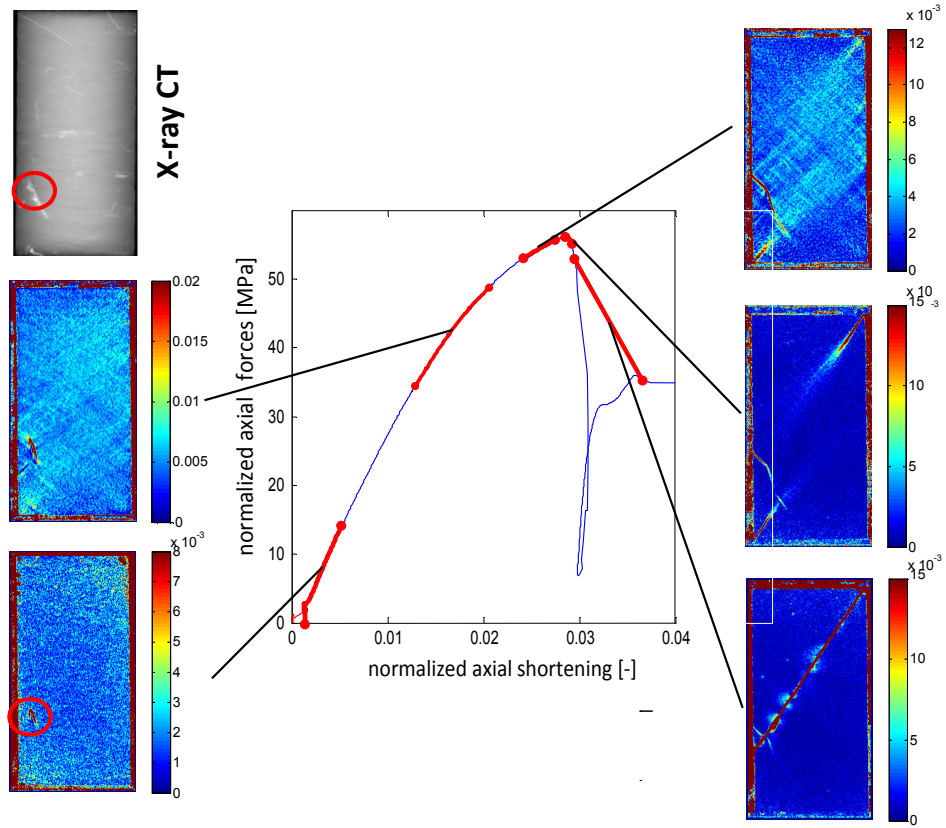
Fig. 17.11: Second invariant of the strain increment . Obtained from digital image correlation of pictures taken during a biaxial compression test on Callovo-Oxfordian claystone at 12 MPa lateral confinement [Bésuelle, 2015]
