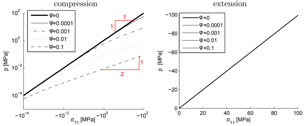
Fig. 8.7: Pore fluid pressure as a reaction to undrained loading
