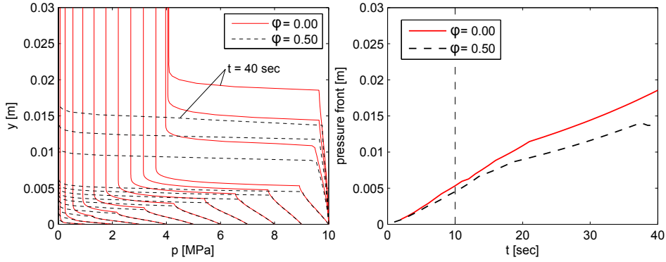
Fig. 10.6: Pressure response to pressure loading for p(y = 0) = 10 \text{ MPa} . Left: pressure profiles for t = 1, 2, 3, 4, 5, 6, 7, 8, 9, 10, 20, 30, 40 seconds. Right: advance of pore pressure front as a function of time.
