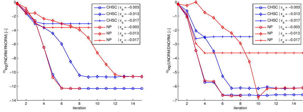
Fig. 12.2: Convergence at \varepsilon_a = -0.30\% , \varepsilon_a = -1.3\% and \varepsilon_a = -1.90\% for the mechanical biaxial test in Section 10.3
