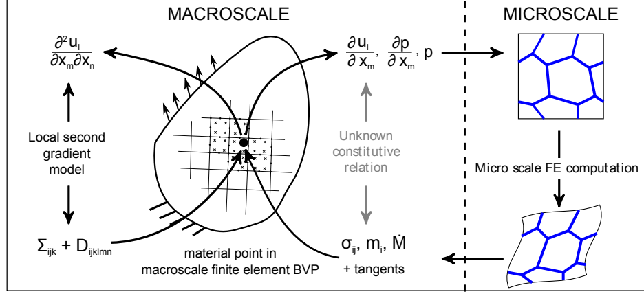
Fig. 3.4: Schematic representation of the hydromechanically coupled doublescale model with local second gradient model.
