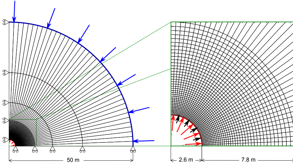
Fig. 16.1: Macroscale mesh for the modelling of gallery excavation.
