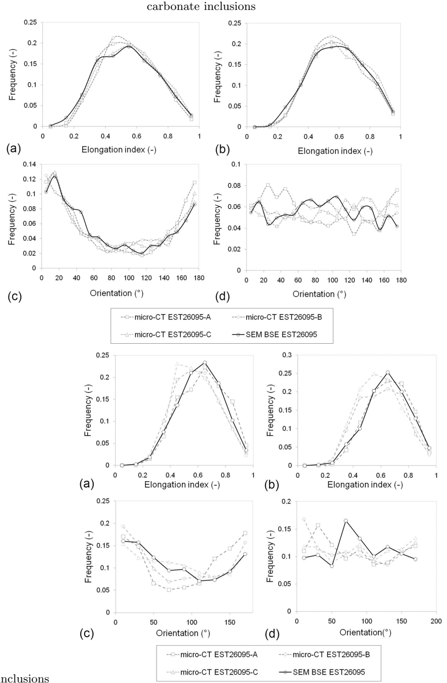
Fig. 1.3: Statistical characterization of the elongation index e and orientation \beta of carbonate (top) and tectosilicate inclusions (bottom) in the bedding plane (b,d) and in the plane parallel to the bedding (a,c) [Robin et al., 2012].
