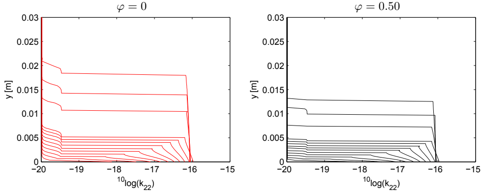
Fig. 10.7: Permeability evolution as a response to pressure loading p(y = 0) = 10 \text{ MPa} for grain porosity \varphi = 0 (left) and \varphi = 0.50 (right) for time t = 1, 2, 3, 4, 5, 6, 7, 8, 9, 20, 30, 40
