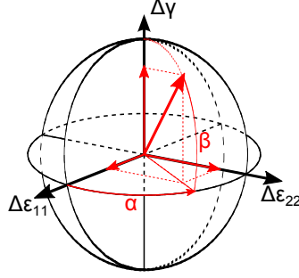
Fig. 15.5: Coordinate system for the extended Gudehus diagrams with (symmetric) shear strain component d\gamma = dF_{12} + dF_{21} where dF_{12} = dF_{21} is used to avoid the influence of stress rotation.
