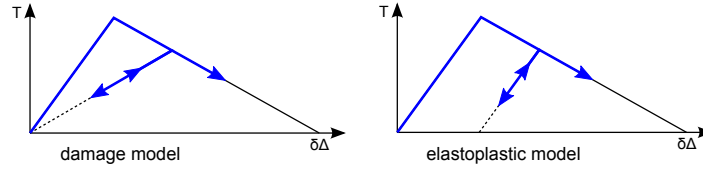
Fig. 14.9: Original damage model for interface cohesion (left) and alternative plastic damage model (right).
