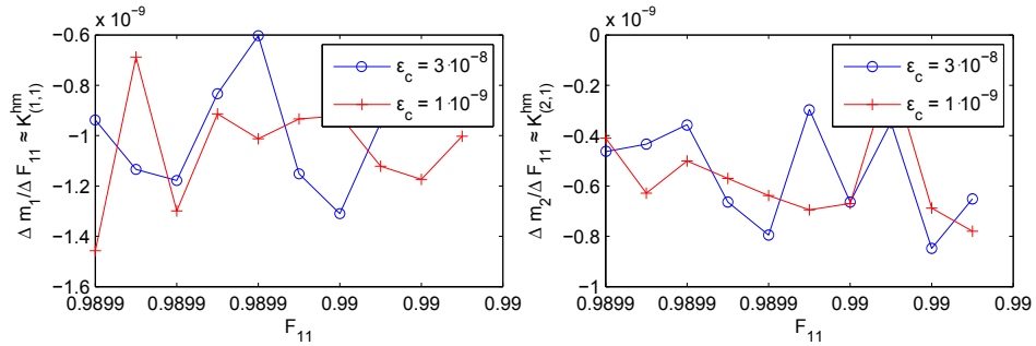
Fig. 9.5: Variation in the increment of flux as a response to an increment of deformation for two computations with different convergence criteria \epsilon_c .
