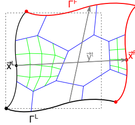
Fig. 4.2: Schematic representation of deformed REV with fixed lead \bullet , lead REV boundary \text{---} , follow REV boundary \text{---} , periodic vectors \longrightarrow , initial REV boundaries \text{---} , interface elements \text{---} and solid element mesh \text{---} .
