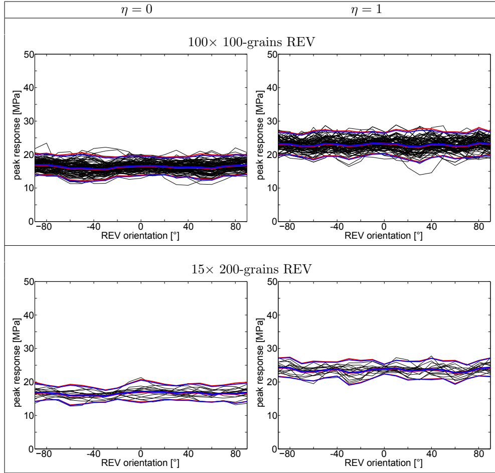
Fig. 11.6: Comparison of series of REV of 100 and 200 grains with the expectation and 2.5% probability upper and lower bound based on fitted normal (blue) and lognormal (red) distribution functions as a function of REV orientation \theta^I
