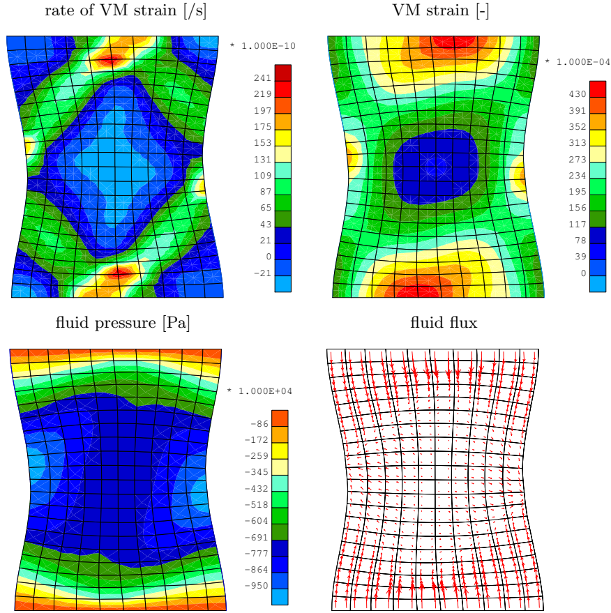
Fig. 10.14: Deformed mesh (displacements multiplied 10×) at the end of Test D.
