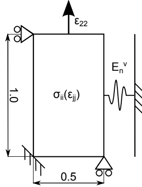
Fig. 8.2: Analytical model of the extension of a block, taking into account the interface stiffness
