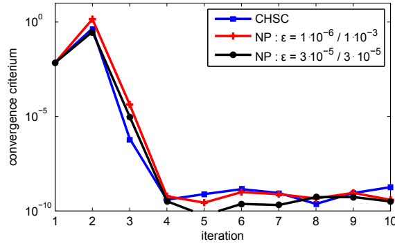
Fig. 9.2: Convergence of a stress-controlled loading step using tangent stiffness matrices obtained by computational homogenization through static condensation (blue), numerical perturbation with 'optimized' perturbation sizes (red) and averaged perturbation sizes (black)
