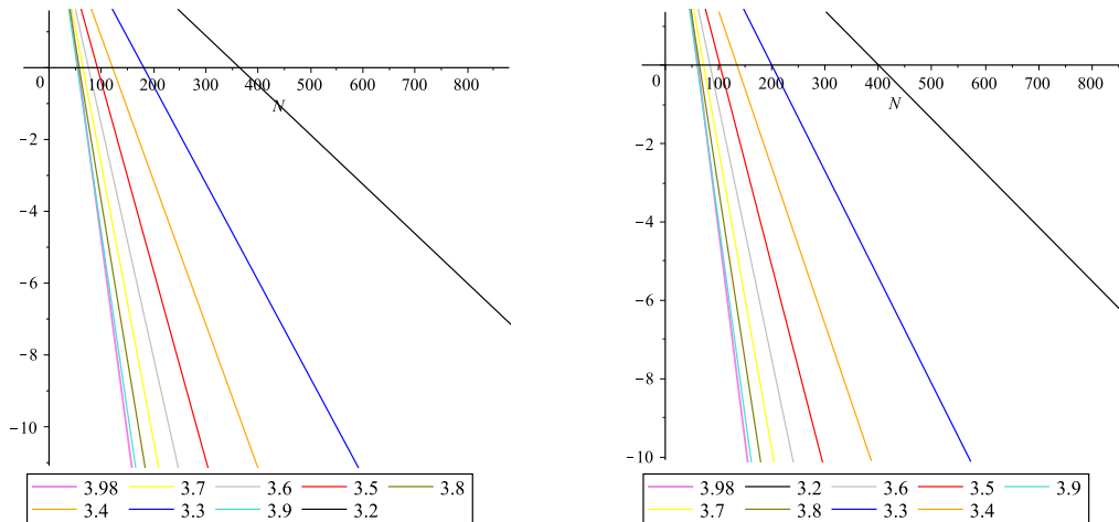
Figure 4.4: \log|E_N(f)| for \mu_2 and \mu_3
