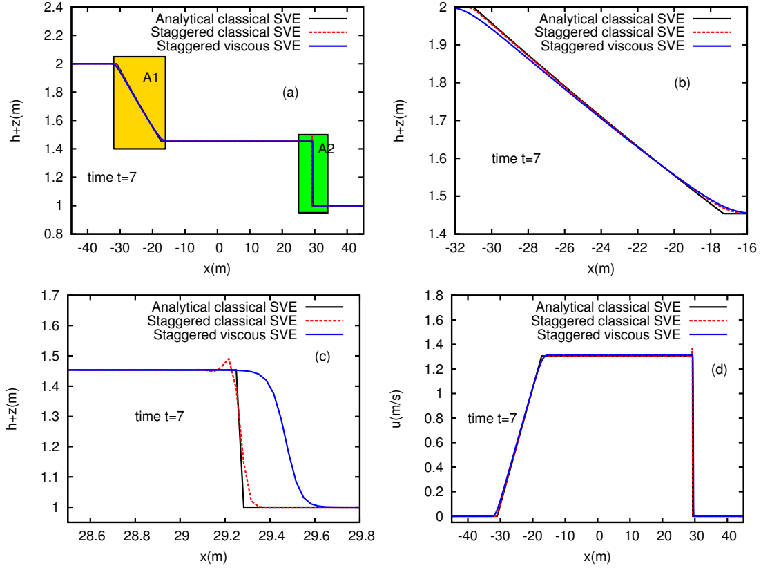
Figure 3.1: Dam-break on a wet bed. (a) The comparison of water level profile on full domain.(b) The zoom area of (A1) on the rarefaction wave. (c) The zoom area of (A2) on the shock wave. (d) The velocity profile on full domain. The CFL condition is 1 and final time t = 7 s.
