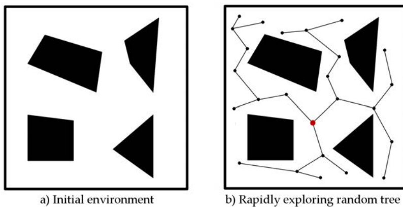
Figure 1.3 – An example of rapidly exploring random tree (b) computed from the environment geometry (a). The origin of the exploration is highlighted in red.
