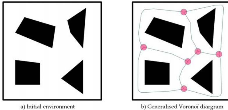
Figure 1.5 – The Generalized Voronoi Diagram (b) computed from the environment geometry (a). Waypoints are highlighted with red circles.
