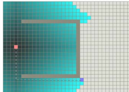
b) Dijkstra (constrained environment)
