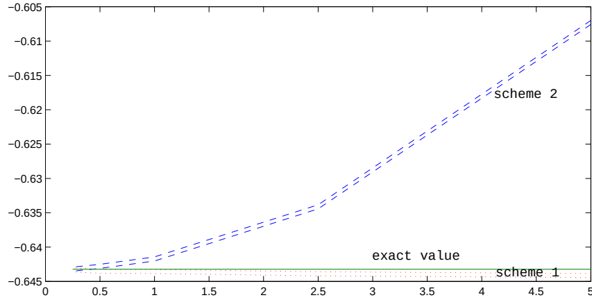
Figure 3.2: Convergence of the discretization schemes. p = d = 3 , 10^7 Monte Carlo samples, T = 5 . The imaginary value of \mathbb{E} [\exp (-i (\operatorname{Tr}(\Gamma X_T) + \Lambda^T Y_T))] , as a function the time step T/N . \Gamma = 0.05I_d, \Lambda = 0.02\mathbf{1}_p and the diffusion parameters x = 0.4I_d, y = 0.2\mathbf{1}_{\mathbb{R}^d}, \alpha = 2.5, a = I_d, \rho = -0.3\mathbf{1}_p, b = 0, K = 0, c = I_d, A = 0 . The value obtained by solving the o.d.e is -0.643222. For each scheme the two curves represent the upper and lower bound of the 95% confidence interval.
