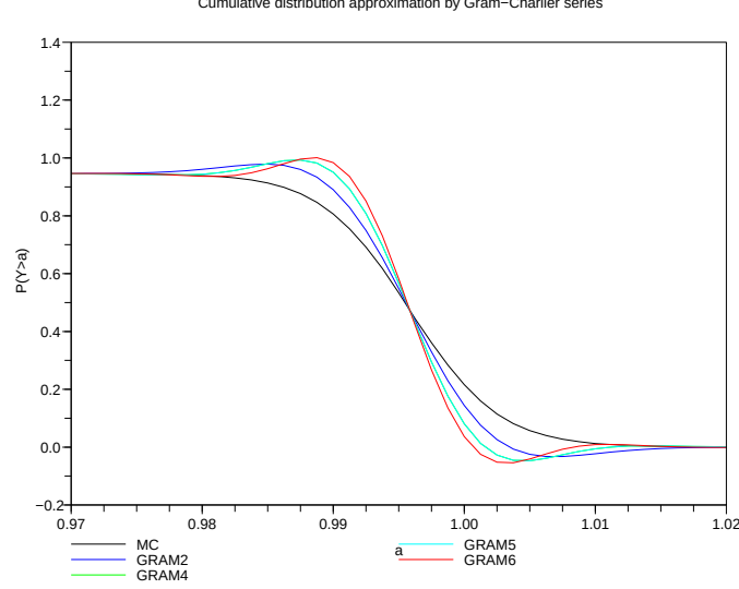
Figure 4.1: Quality of the approximation of Q^T(P_{T,T+\delta} > a) by the Gram-Charlier series at different orders, with T = 4 and \delta = 3m . The model parameters are x = 10^{-4}I_d , y = (-0.02, 0.01) , \alpha = 2.5 , b = \text{diag}(-0.11, -1.1) , K = \text{diag}(1, 0.1) , c = I_d . The higher order moments of the ZCB are computed using the numerical resolution of the MRDE described in 3.1.4, with a time discretization step of 0.01.
